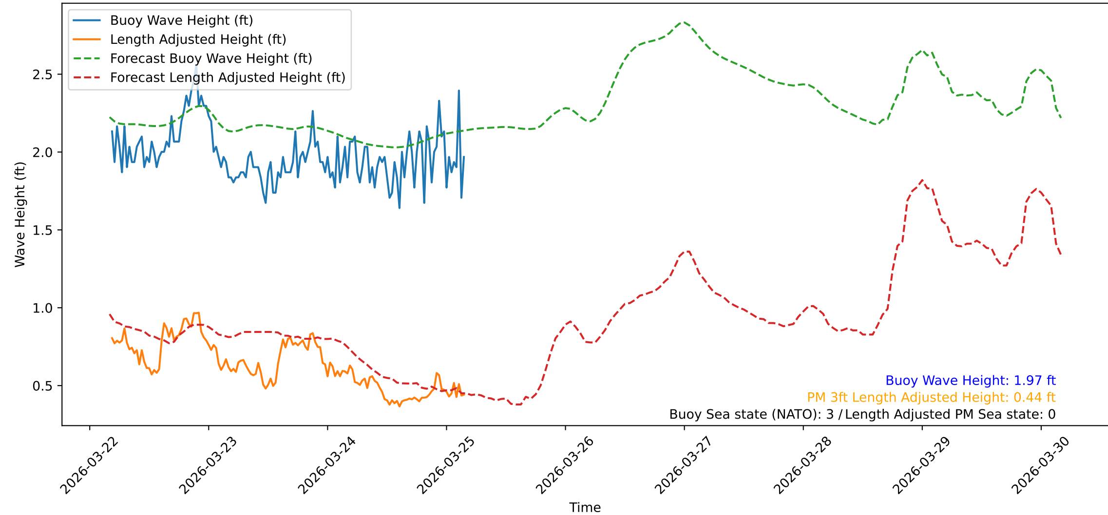
Wave Heights over Time for Red Beach at 2026-03-25 04:20:46
