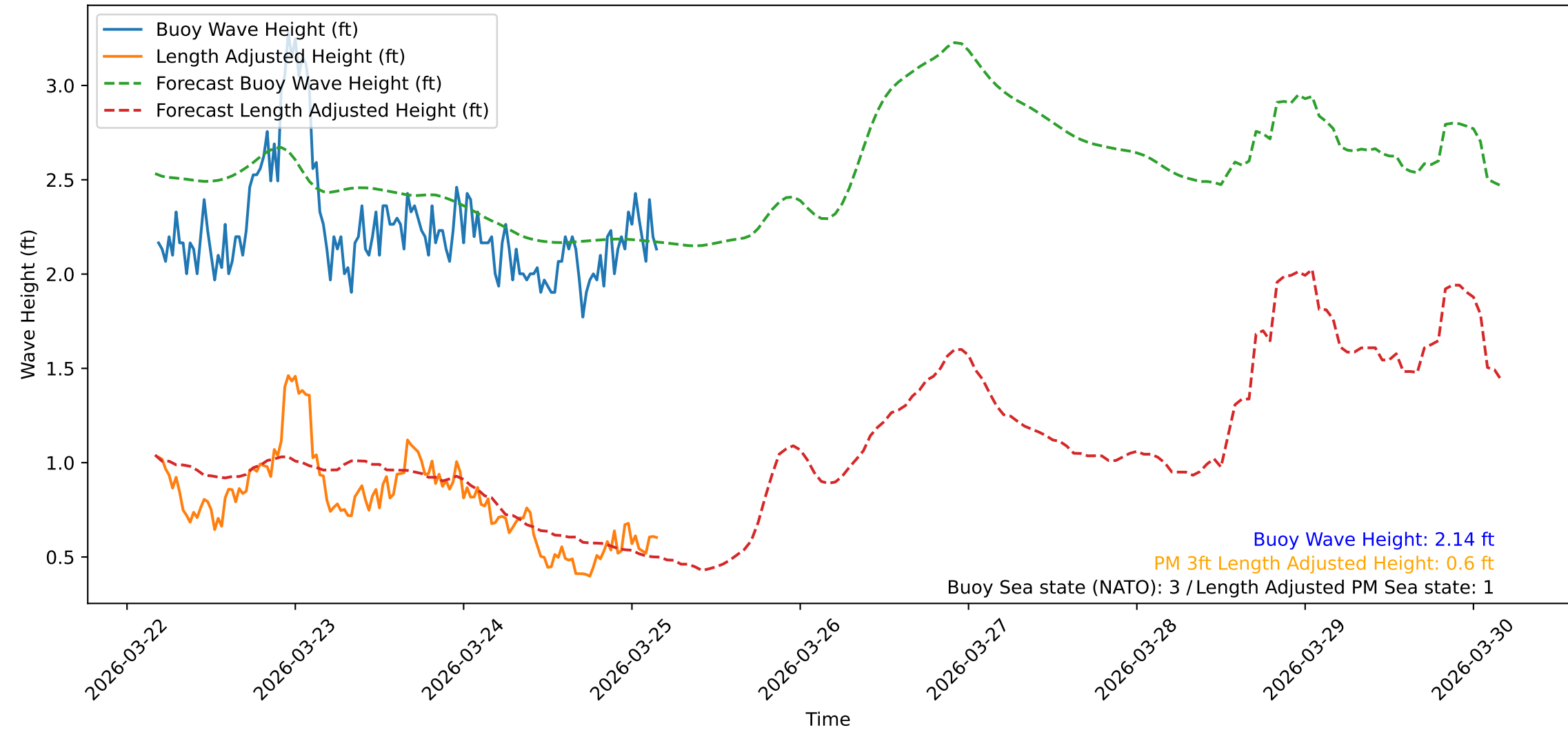
Wave Heights over Time for Green Beach at 2026-03-25 04:21:08
