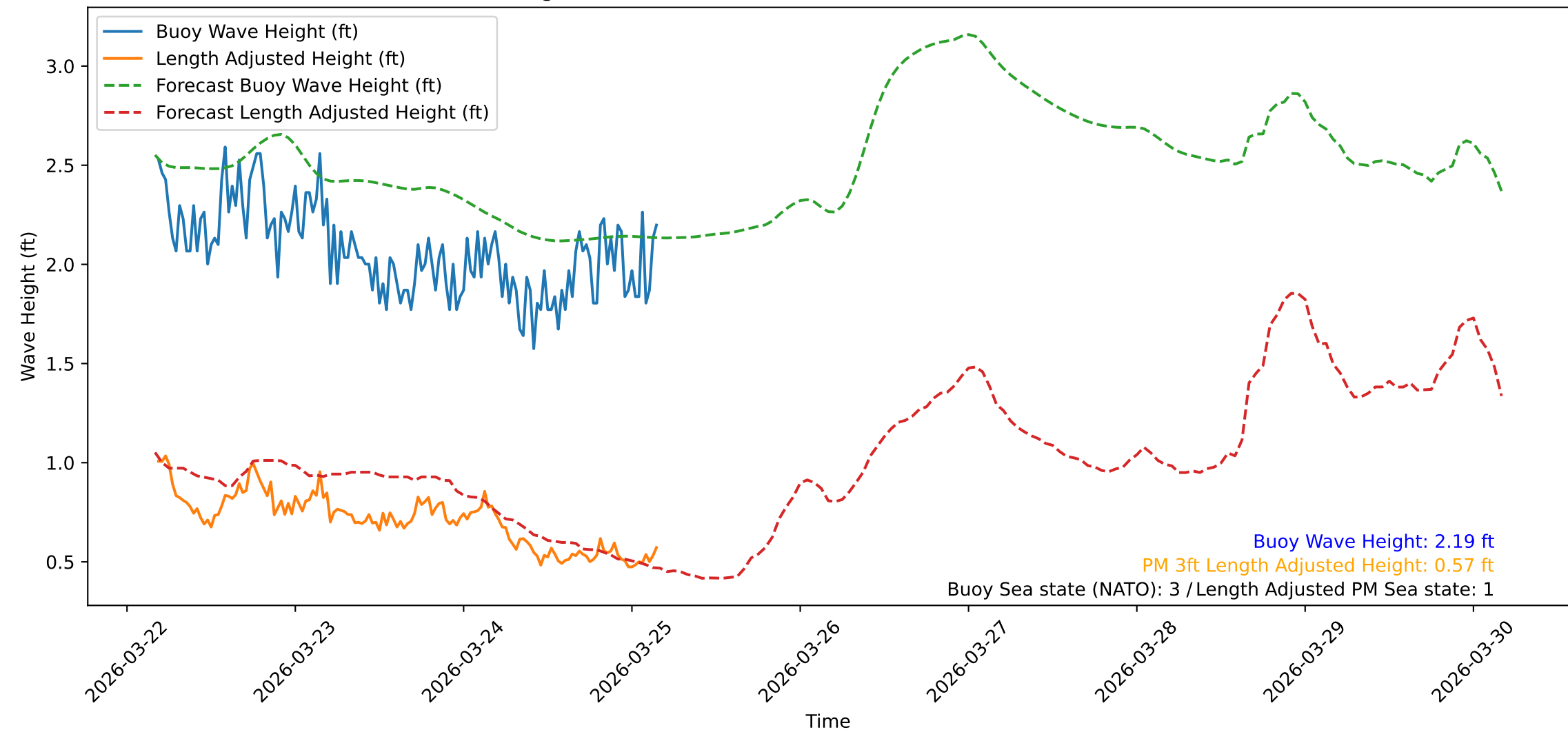
Wave Heights over Time for Oceanside Harbor at 2026-03-25 04:20:30
