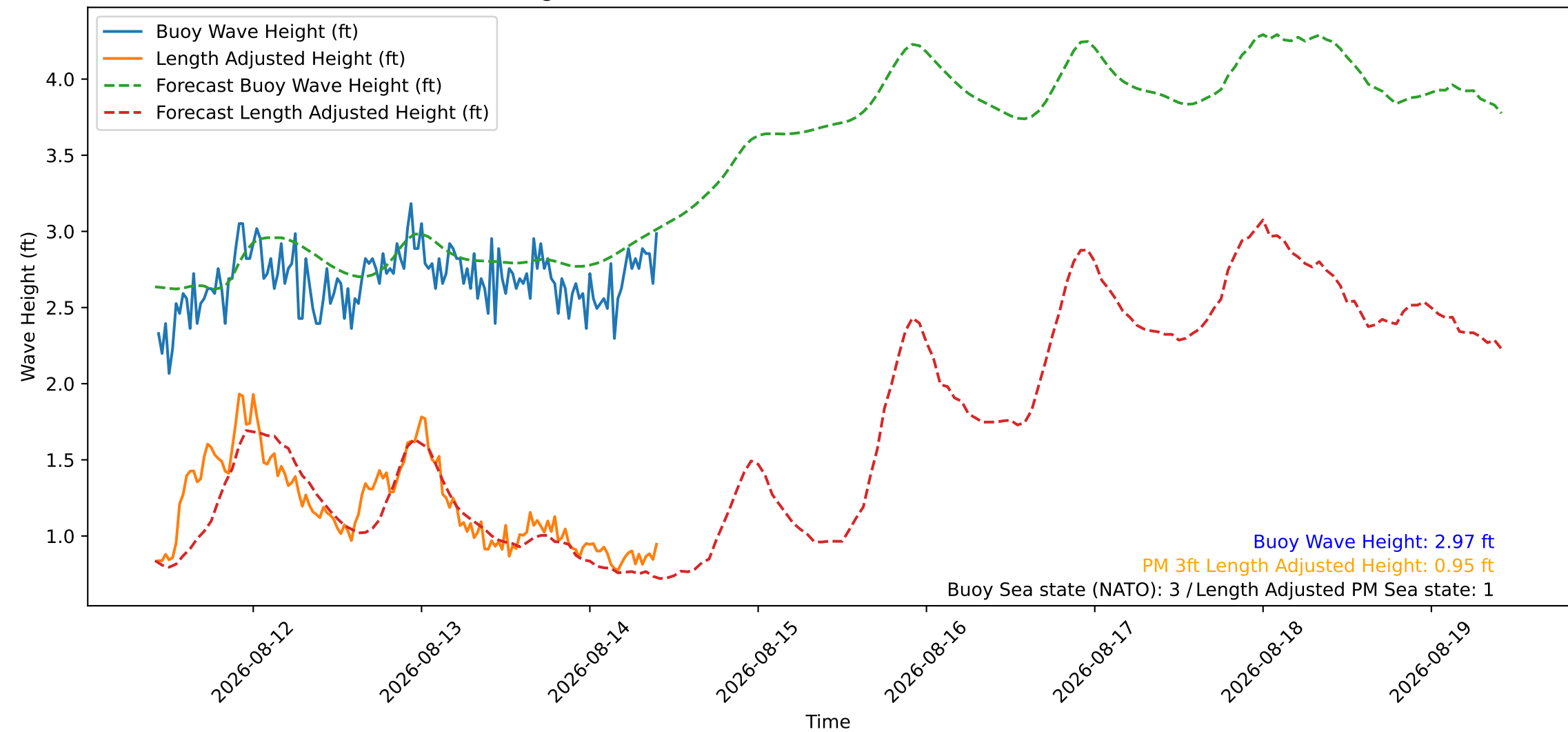
Wave Heights over Time for Oceanside Harbor at 2026-08-14 10:20:26
