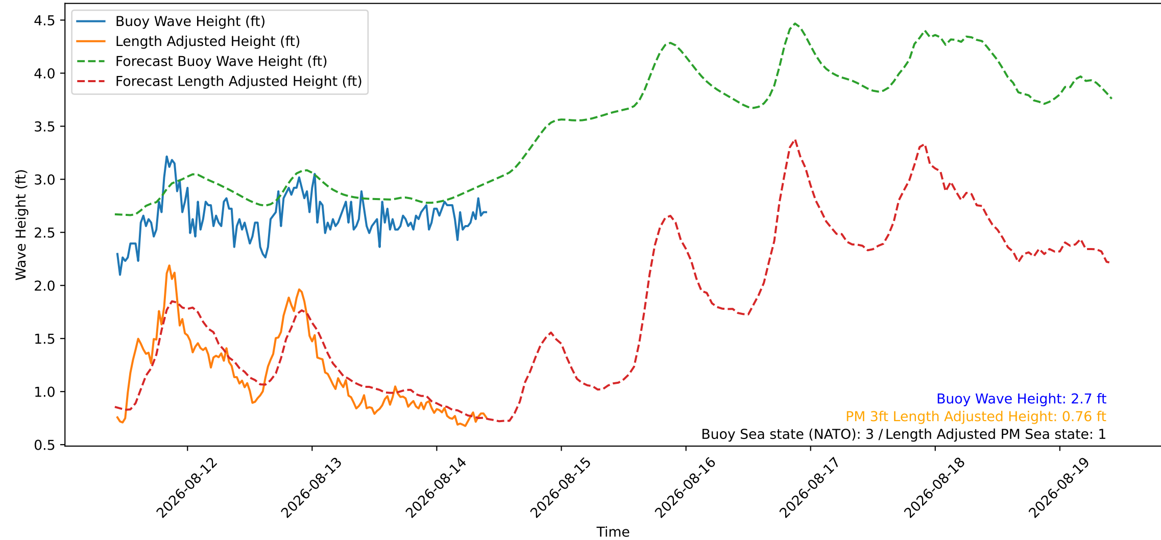
Wave Heights over Time for Green Beach at 2026-08-14 10:21:09
