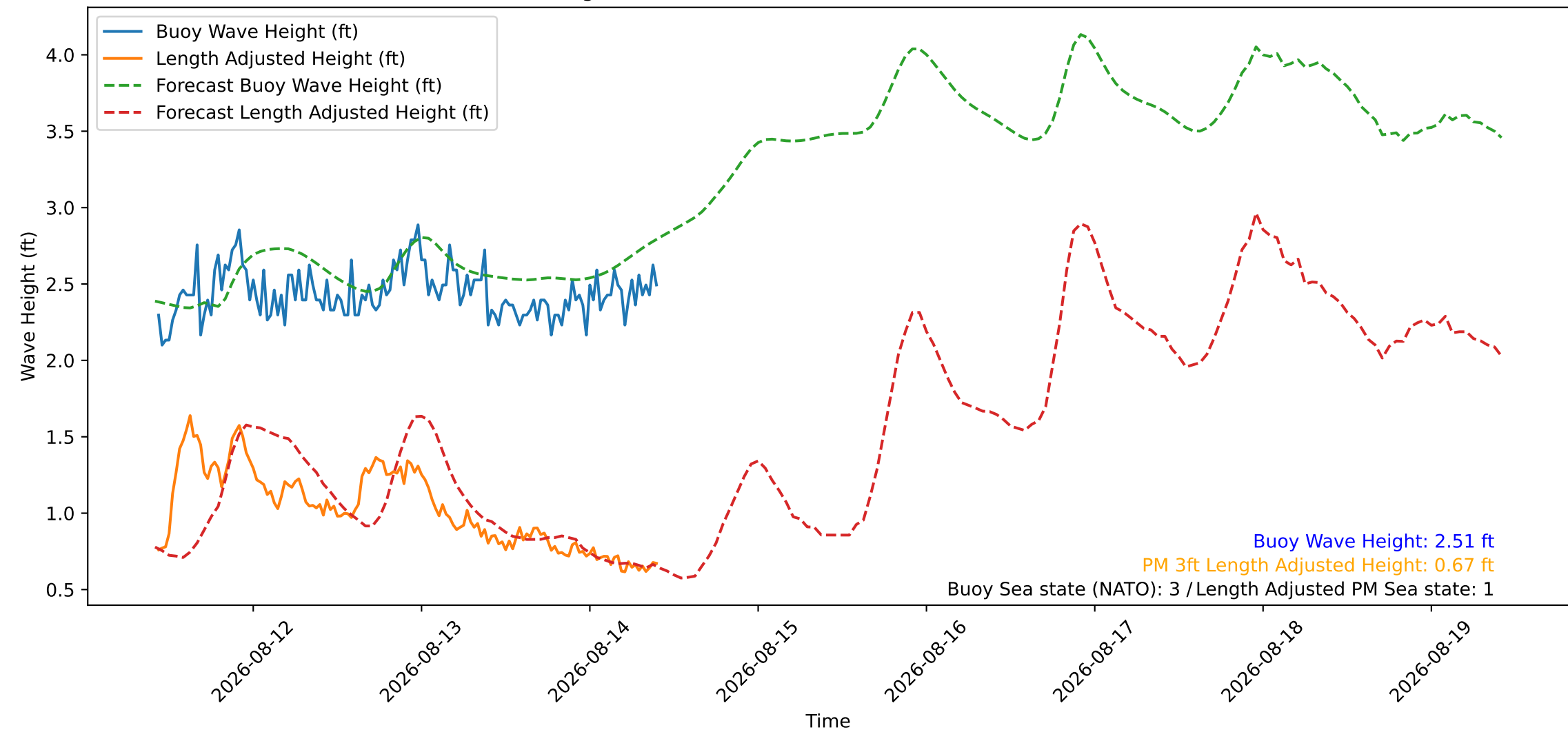
Wave Heights over Time for Red Beach at 2026-08-14 10:20:47
