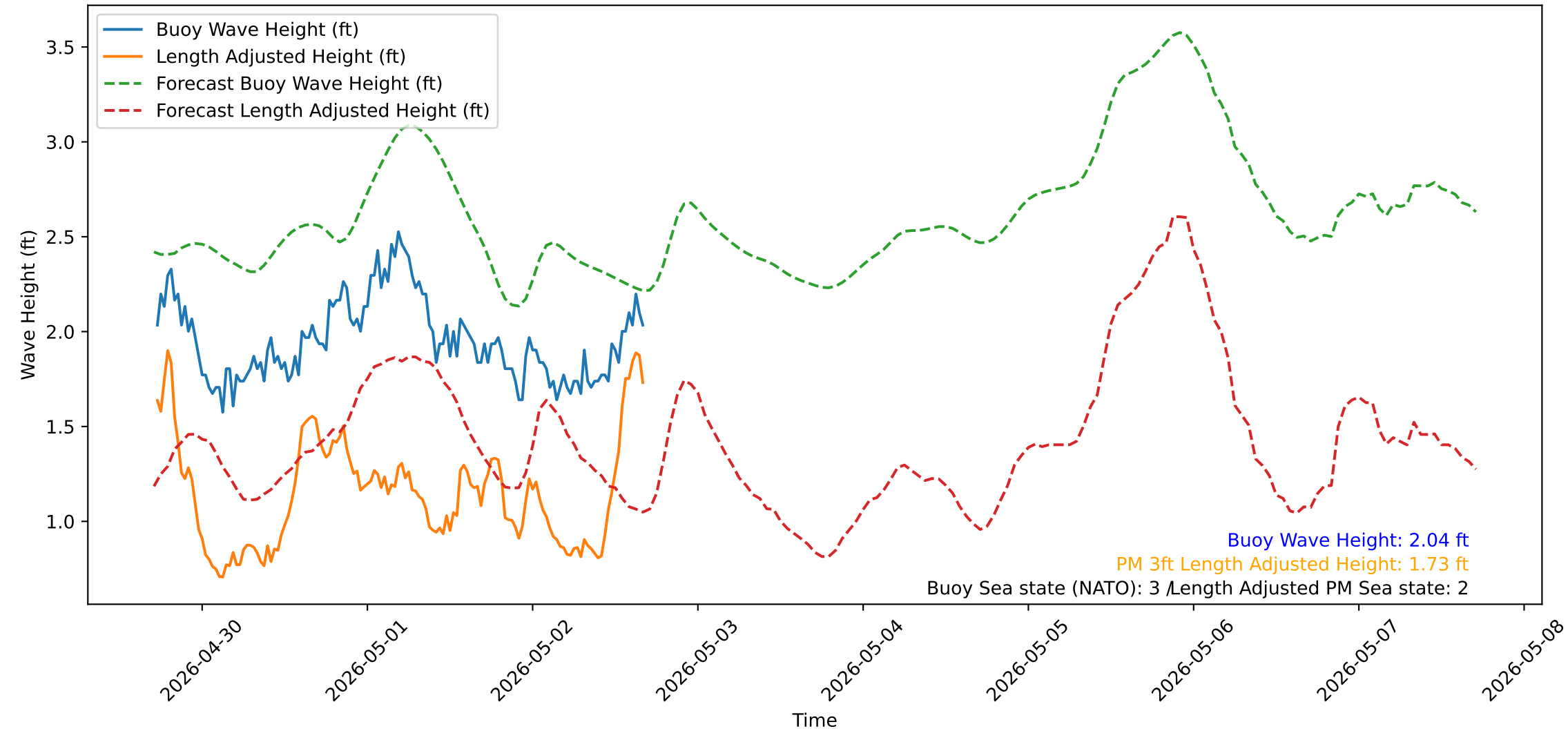
Wave Heights over Time for Red Beach at 2026-05-02 17:00:51
