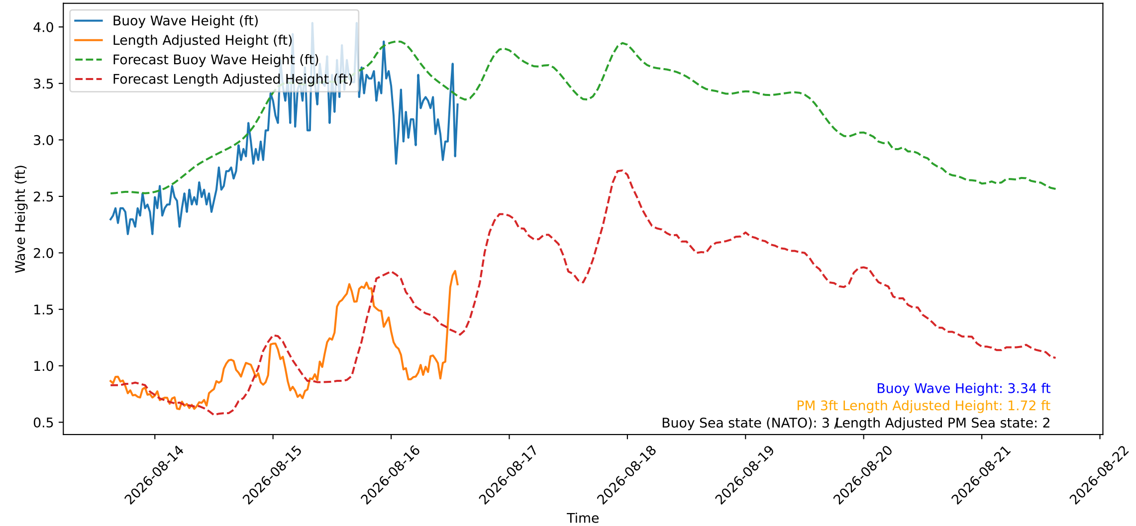
Wave Heights over Time for Red Beach at 2026-08-16 14:40:47
