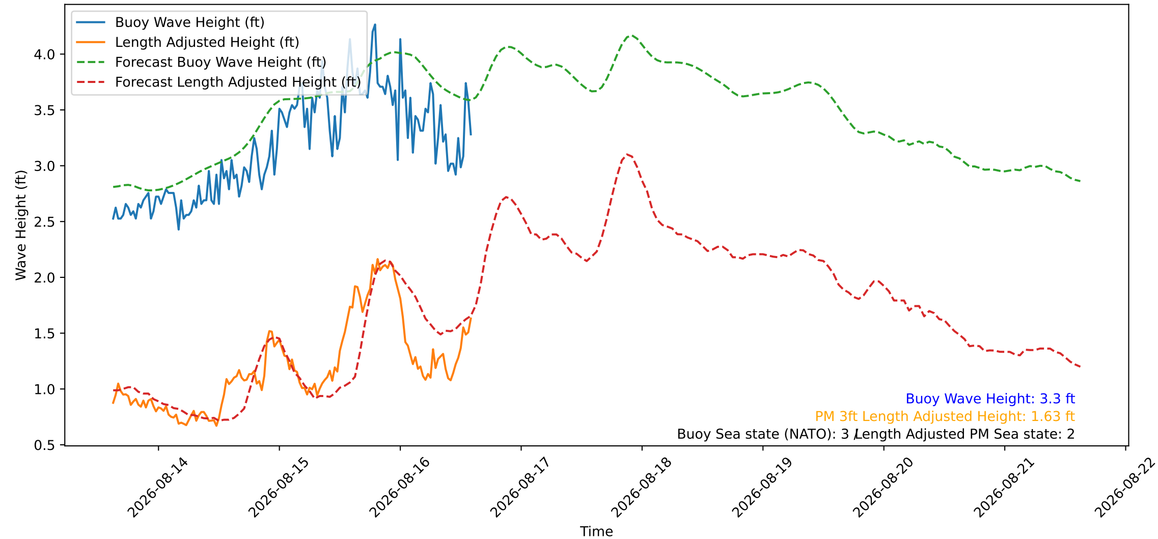
Wave Heights over Time for Green Beach at 2026-08-16 14:41:10
