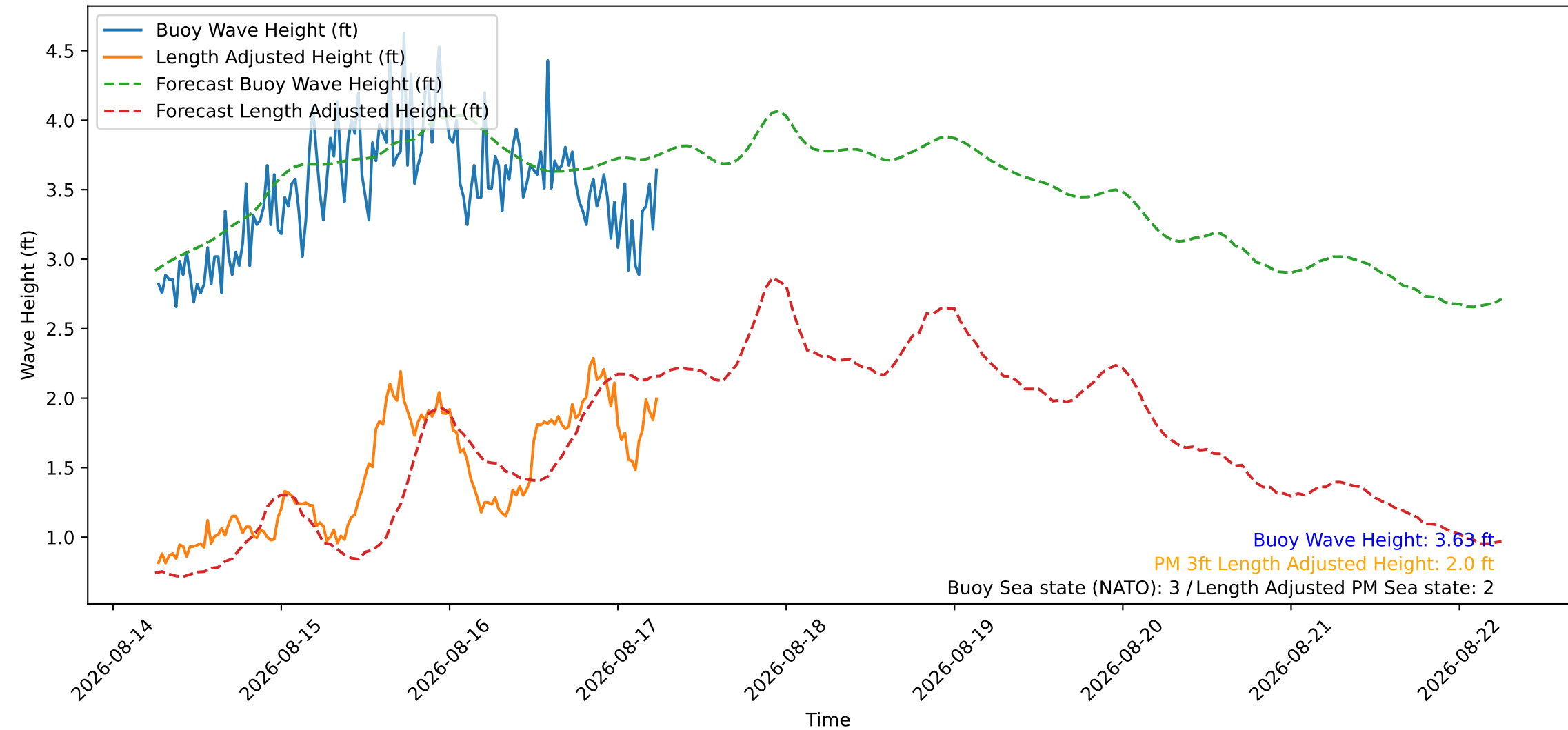
Wave Heights over Time for Oceanside Harbor at 2026-08-17 06:20:27
