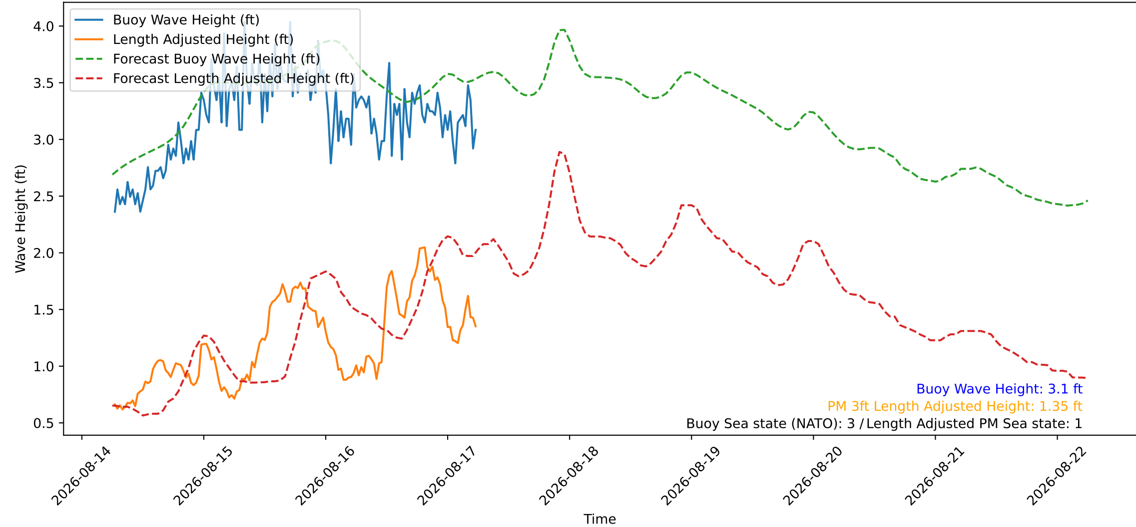
Wave Heights over Time for Red Beach at 2026-08-17 06:20:47
