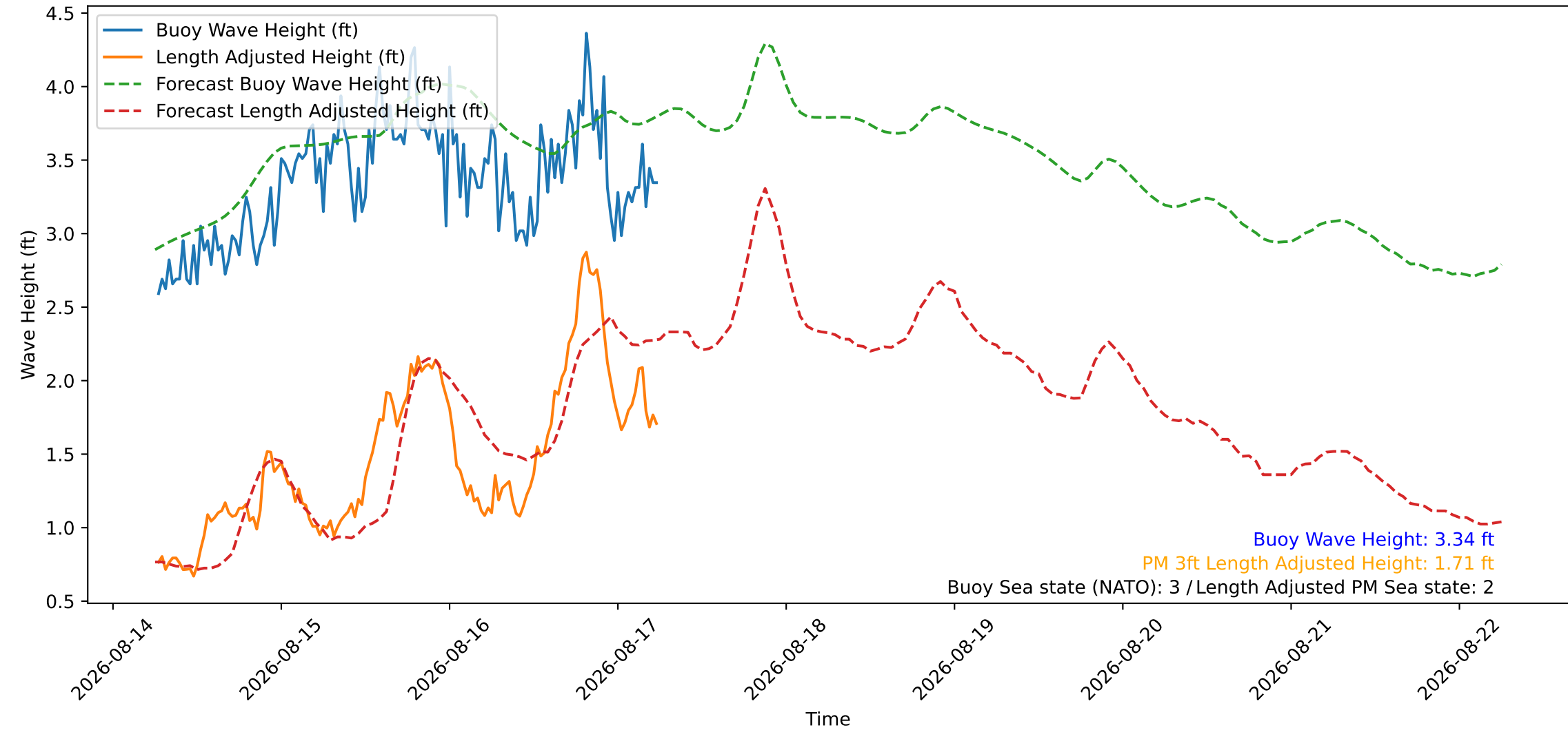
Wave Heights over Time for Green Beach at 2026-08-17 06:21:11
