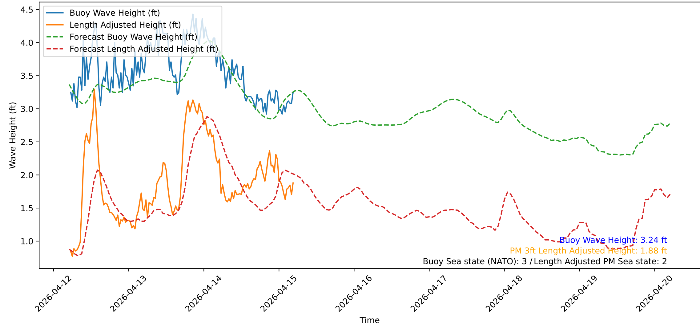
Wave Heights over Time for Red Beach at 2026-04-15 05:20:51
