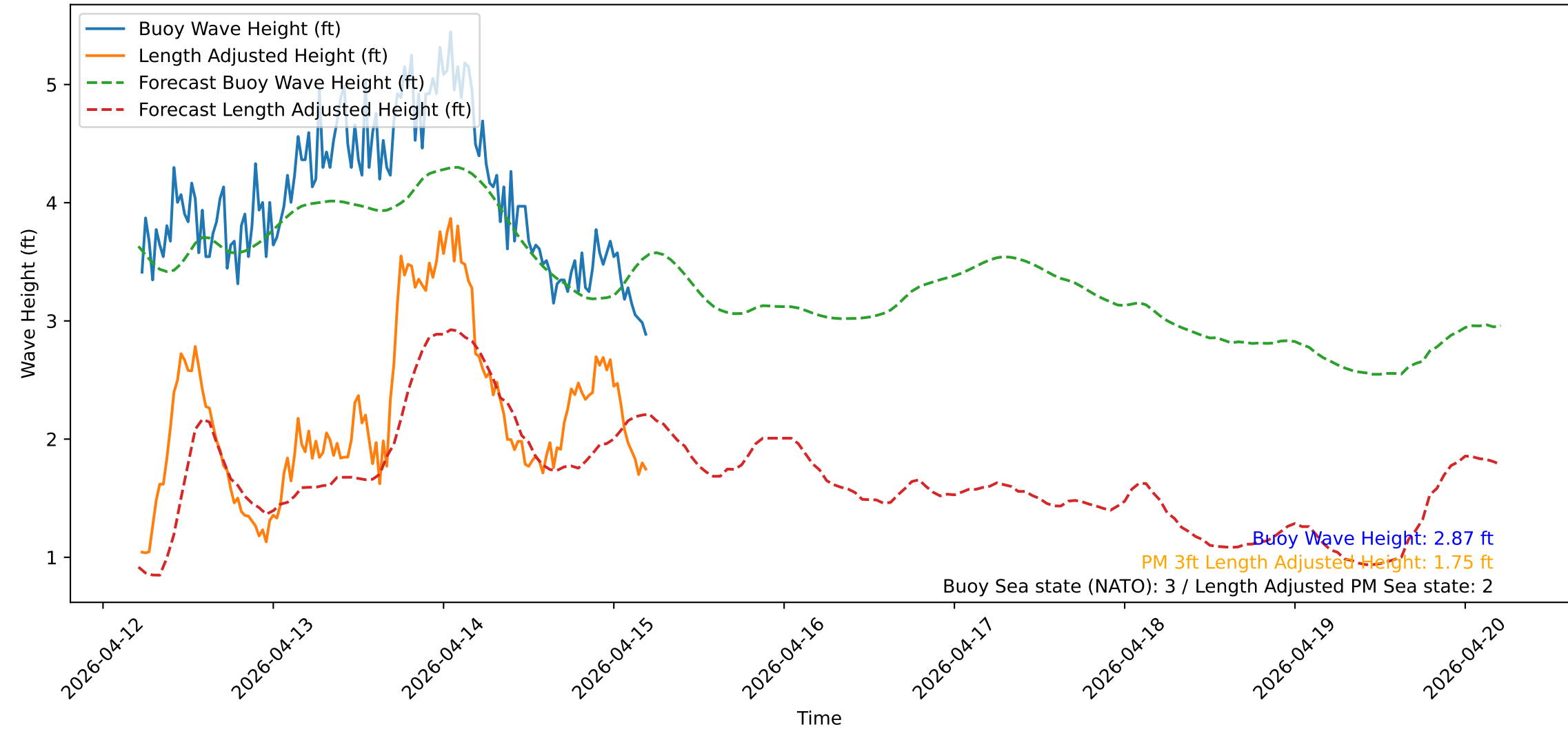
Wave Heights over Time for Oceanside Harbor at 2026-04-15 05:20:31
