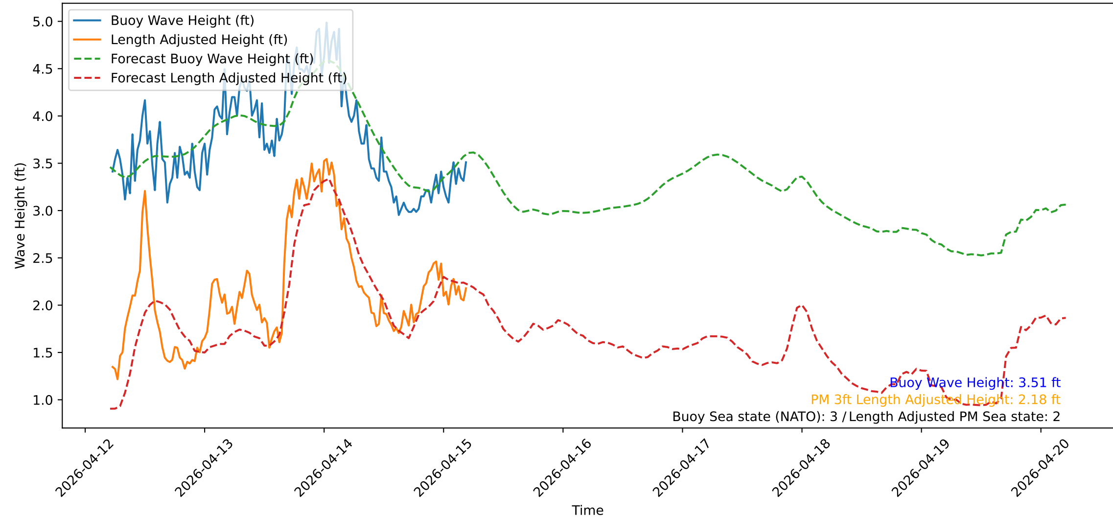
Wave Heights over Time for Green Beach at 2026-04-15 05:21:13
