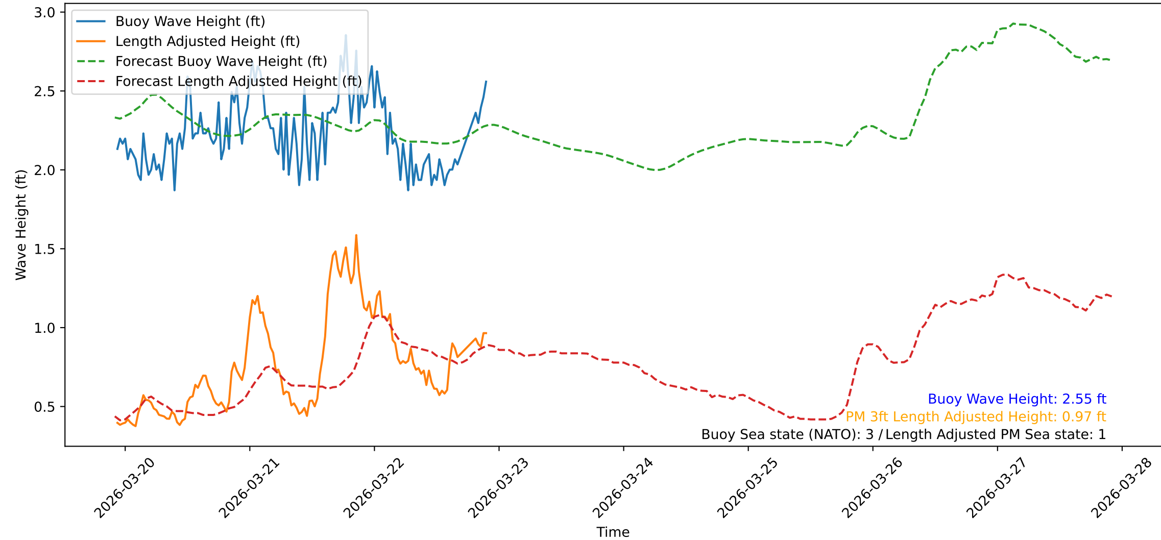
Wave Heights over Time for Red Beach at 2026-03-22 22:10:47
