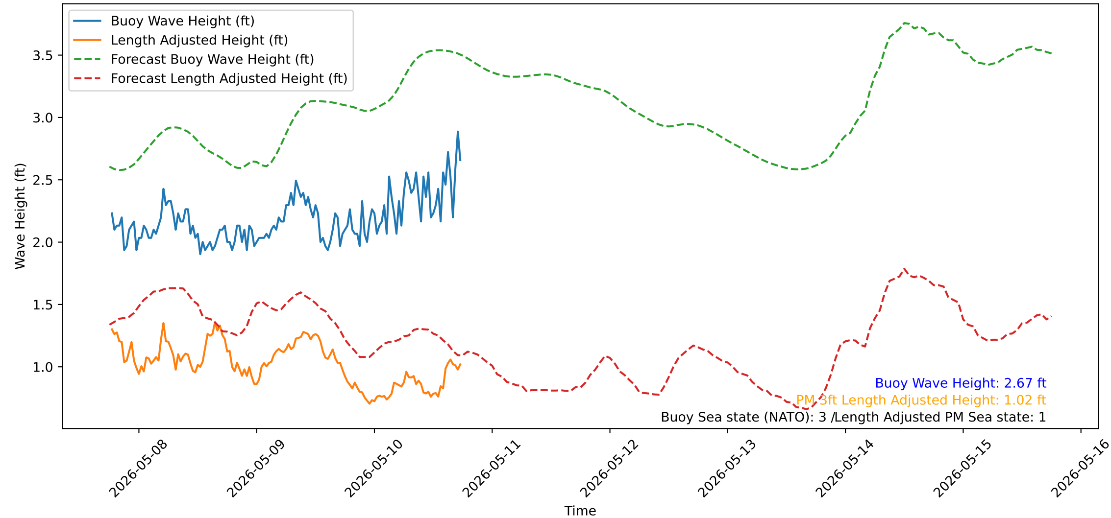
Wave Heights over Time for Red Beach at 2026-05-10 18:20:52
