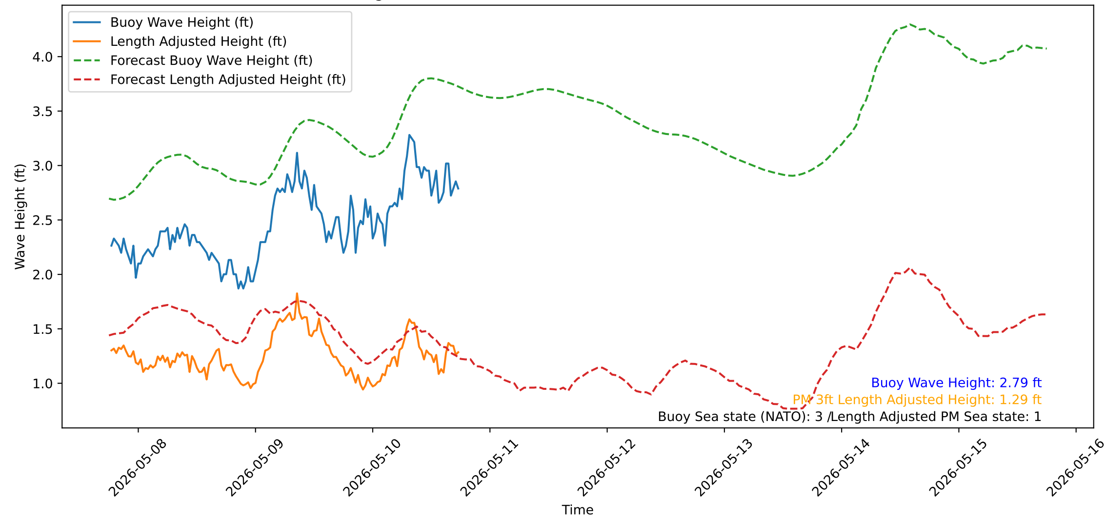
Wave Heights over Time for Oceanside Harbor at 2026-05-10 18:20:32
