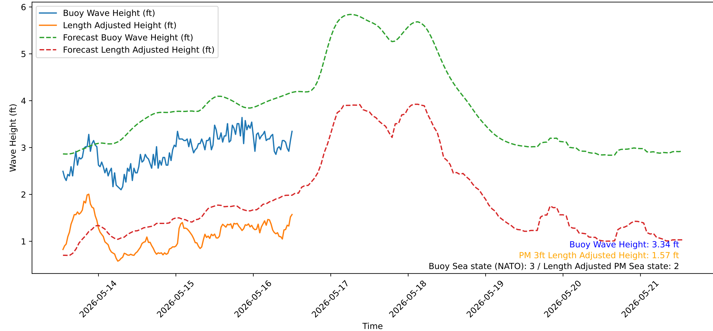
Wave Heights over Time for Green Beach at 2026-05-16 13:01:12
