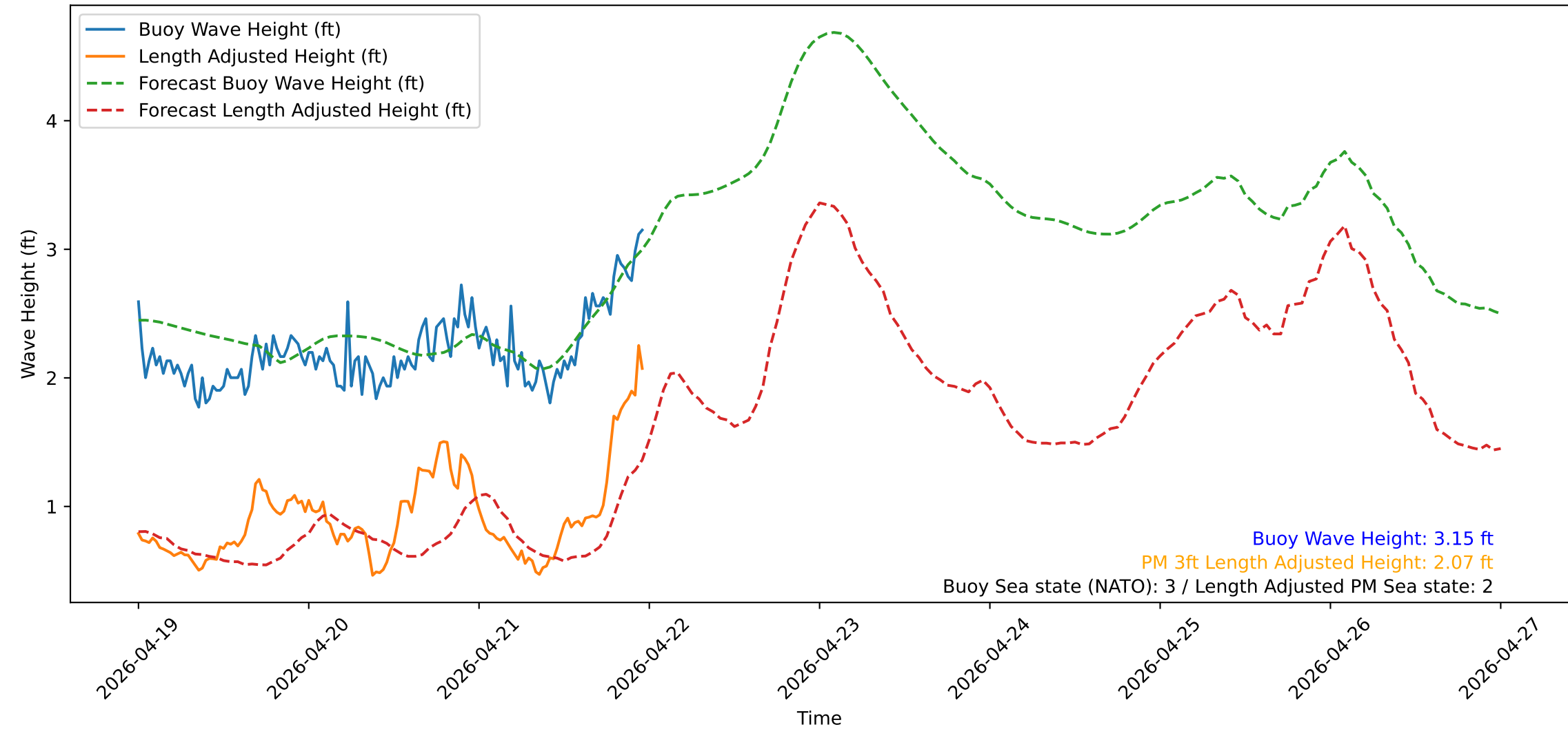
Wave Heights over Time for Red Beach at 2026-04-21 23:40:51
