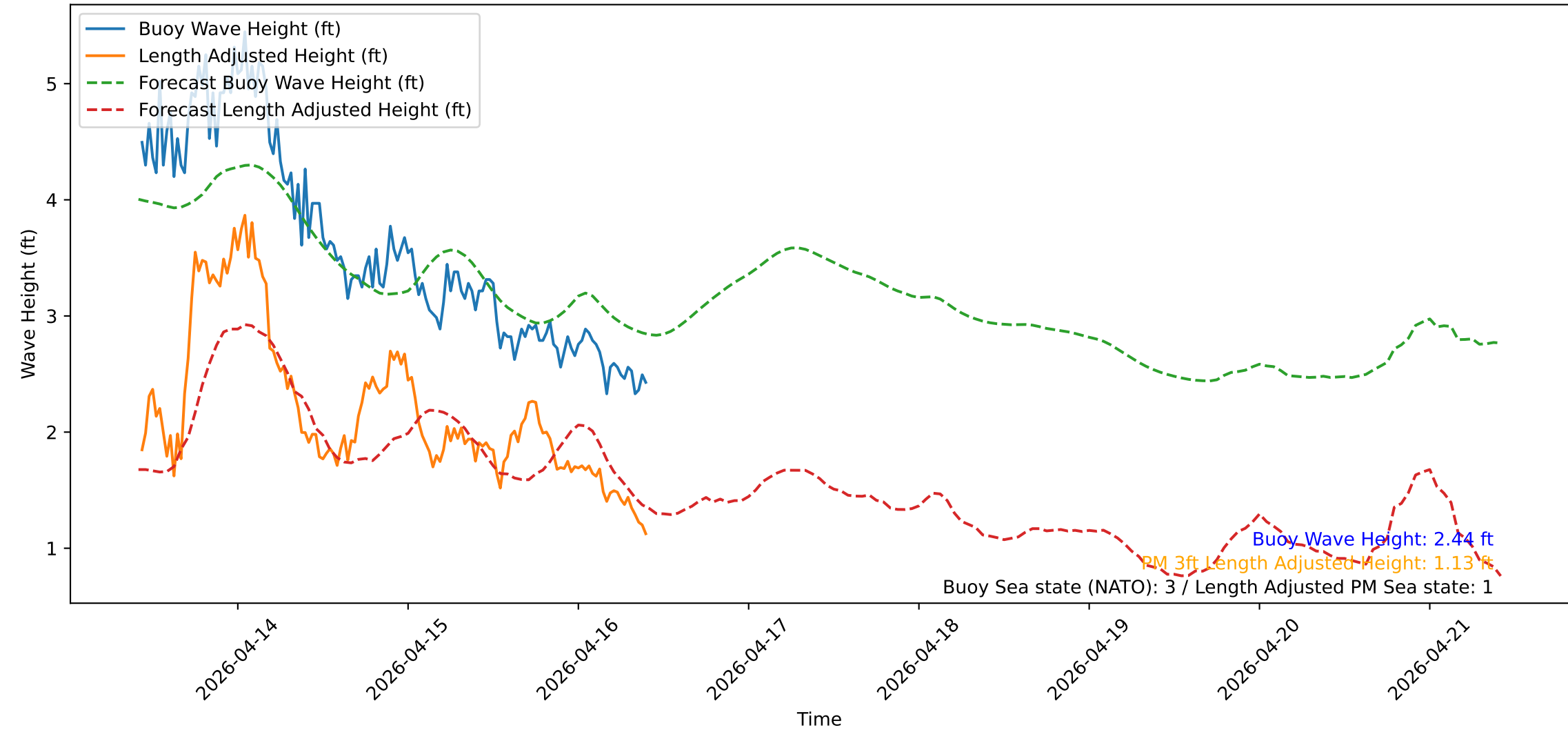
Wave Heights over Time for Oceanside Harbor at 2026-04-16 10:20:31
