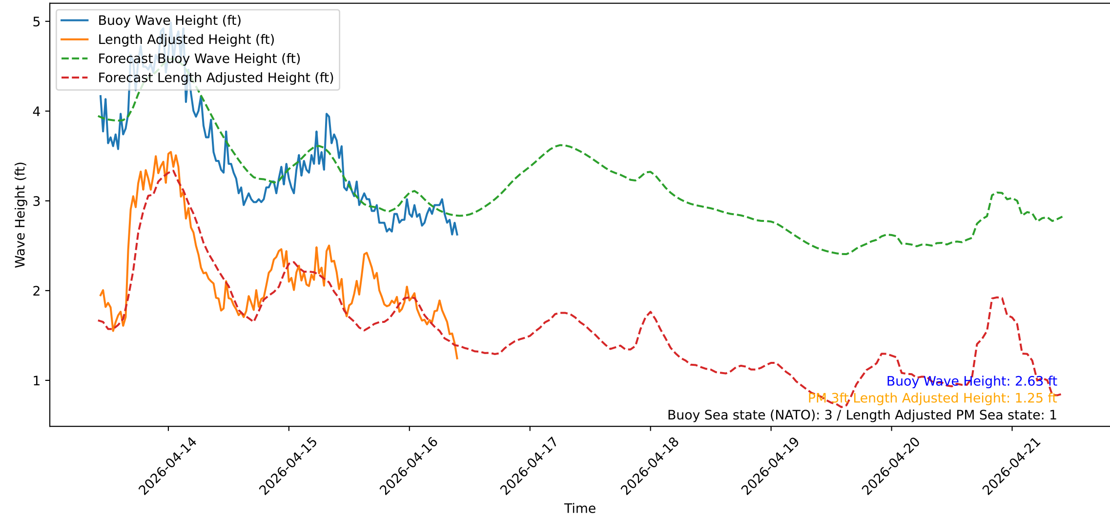
Wave Heights over Time for Green Beach at 2026-04-16 10:21:14
