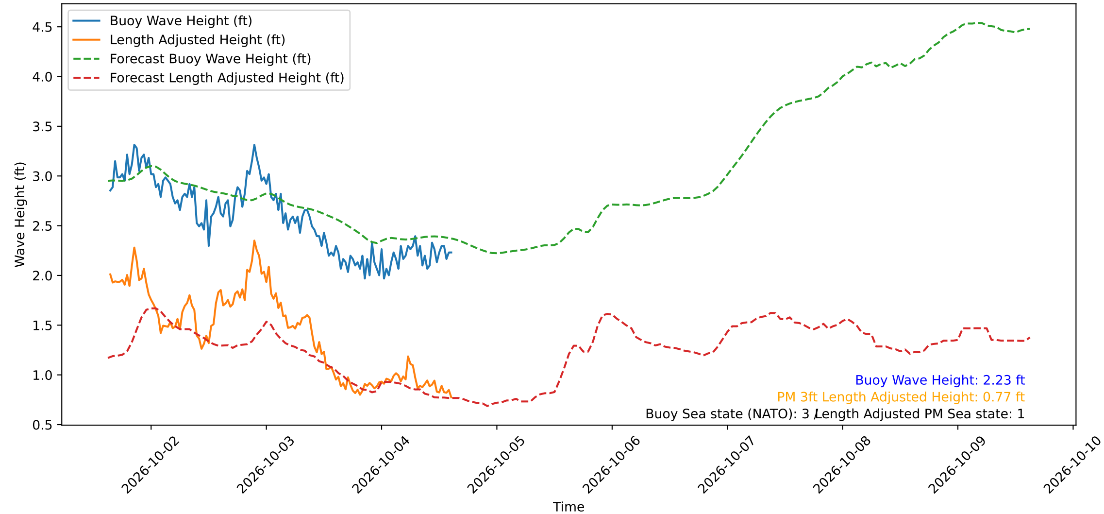
Wave Heights over Time for Oceanside Harbor at 2026-10-04 15:20:29
