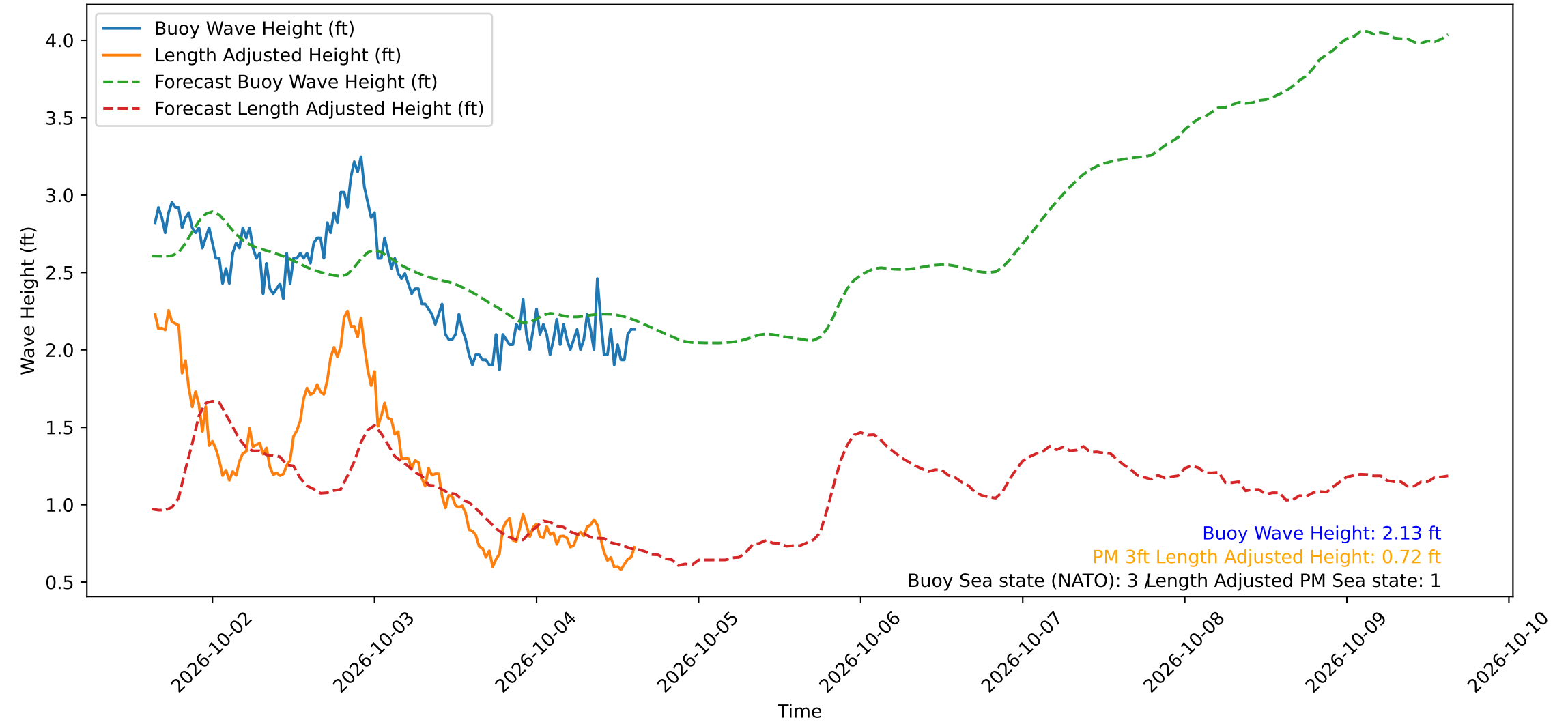
Wave Heights over Time for Red Beach at 2026-10-04 15:20:50
