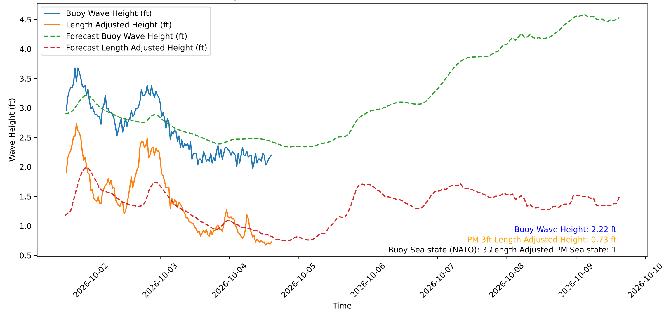
Wave Heights over Time for Green Beach at 2026-10-04 15:21:14
