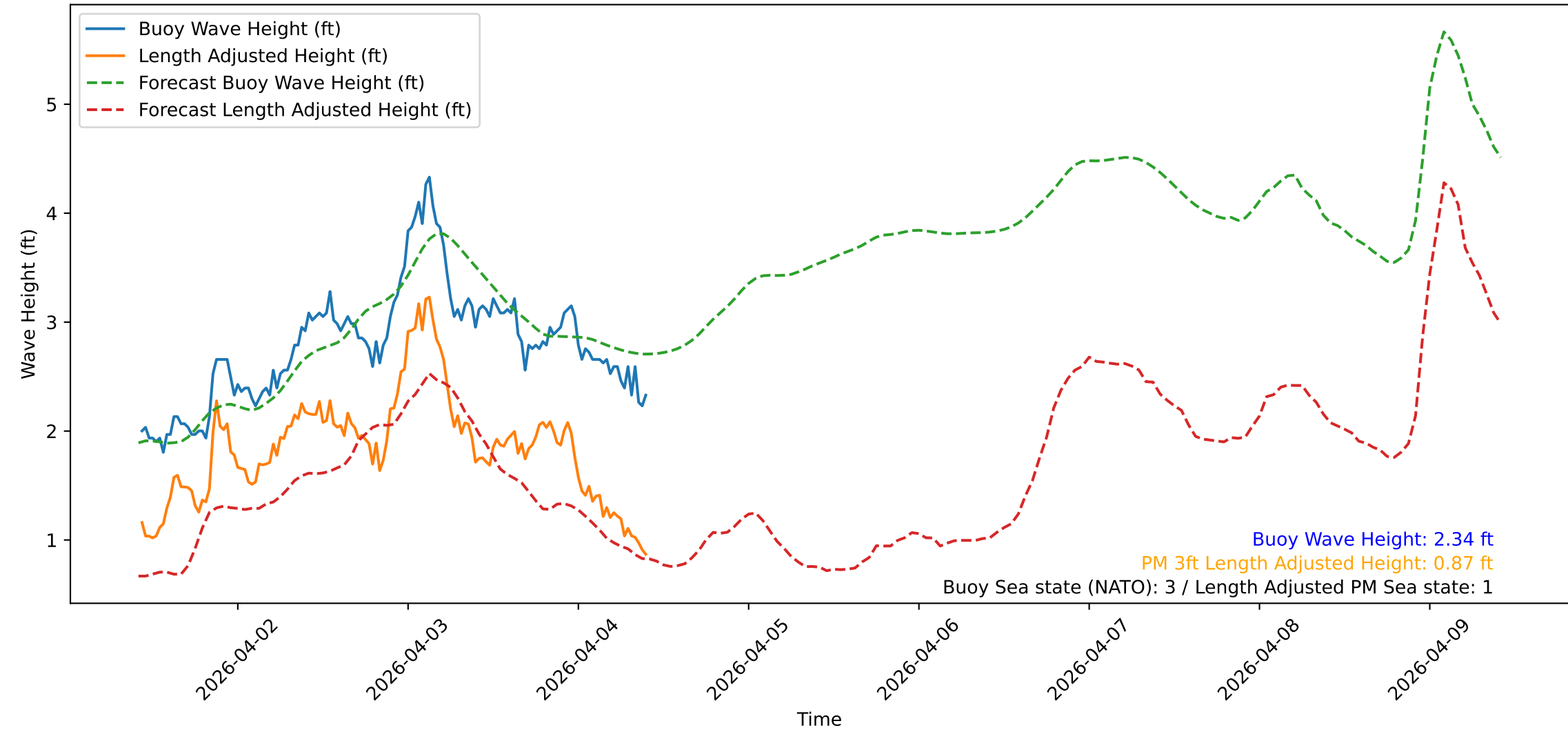
Wave Heights over Time for Green Beach at 2026-04-04 10:21:10
