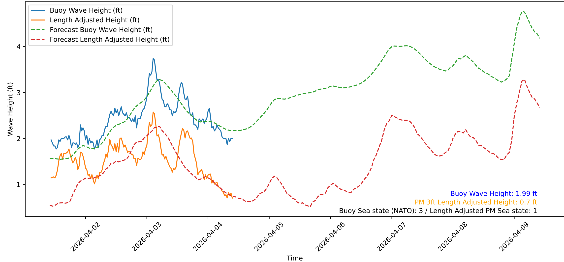
Wave Heights over Time for Red Beach at 2026-04-04 10:20:47
