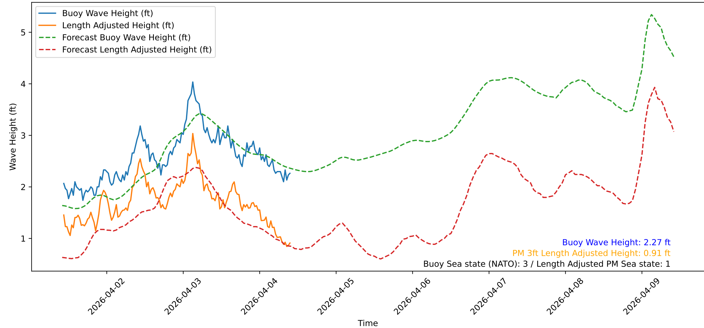
Wave Heights over Time for Oceanside Harbor at 2026-04-04 10:20:31
