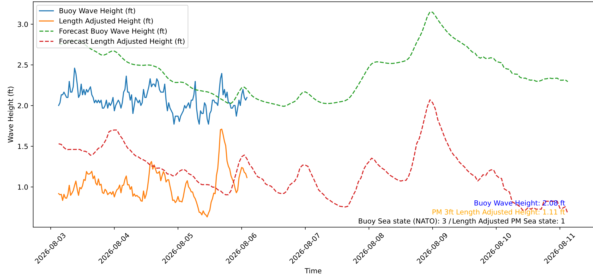
Wave Heights over Time for Red Beach at 2026-08-06 02:50:46
