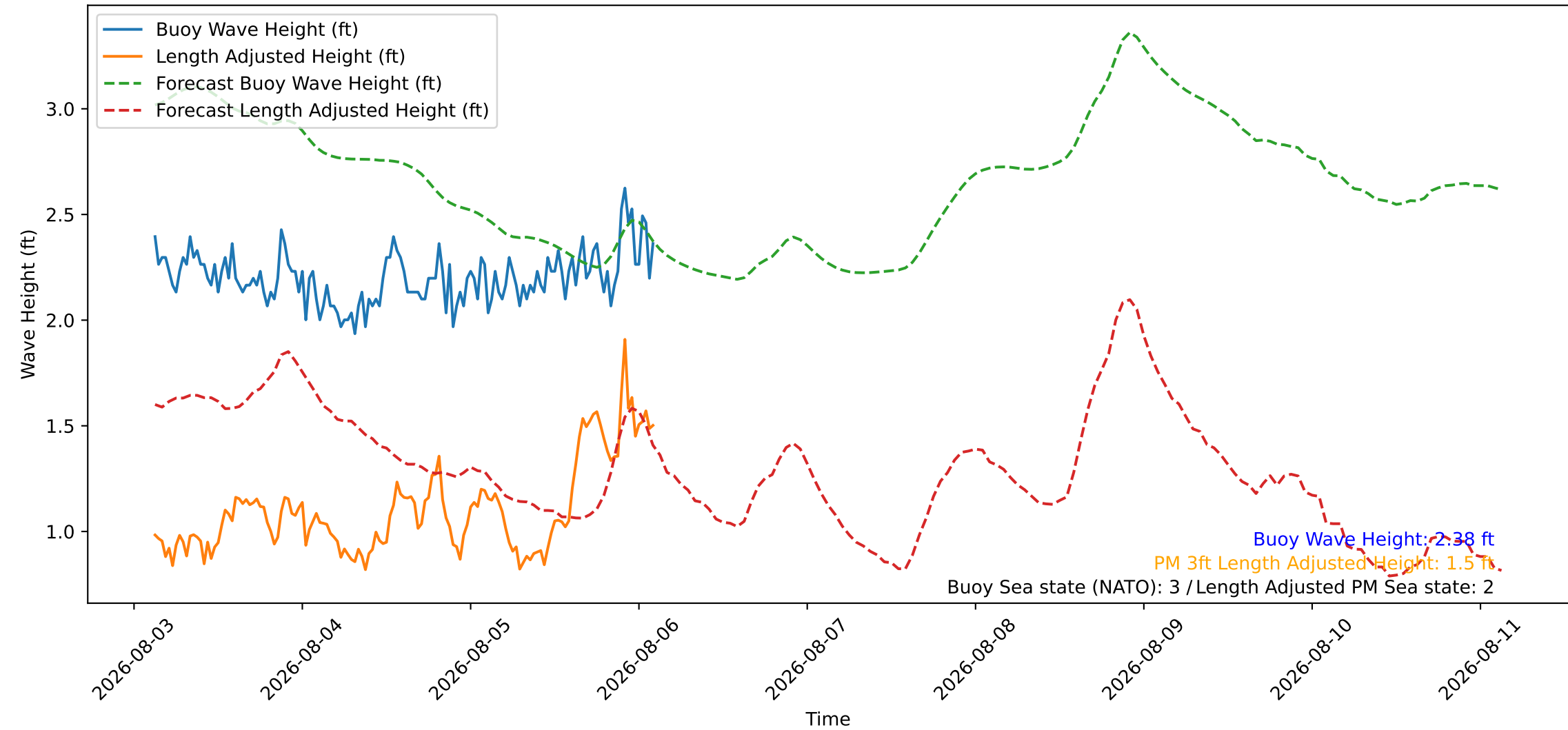
Wave Heights over Time for Green Beach at 2026-08-06 02:51:09
