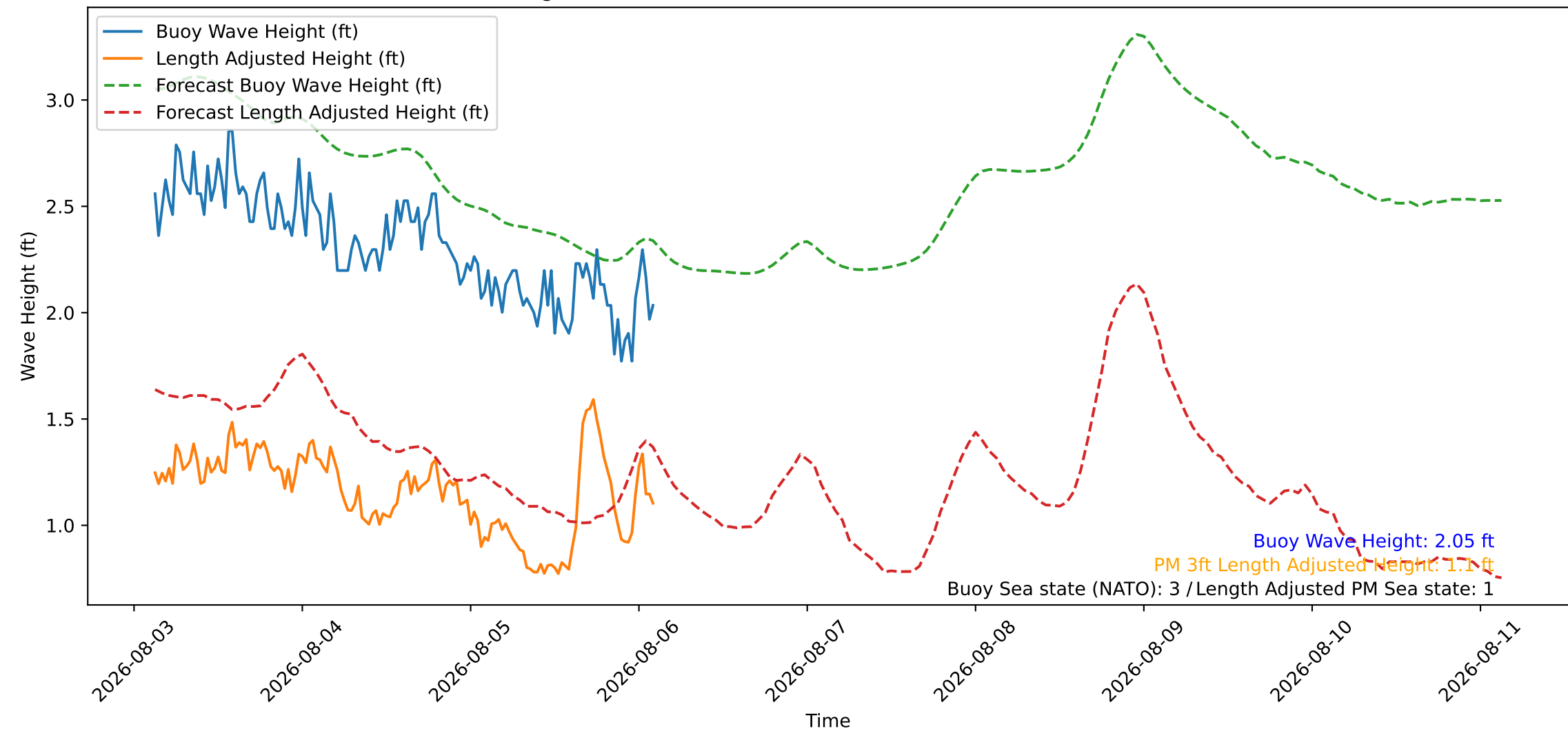
Wave Heights over Time for Oceanside Harbor at 2026-08-06 02:50:26
