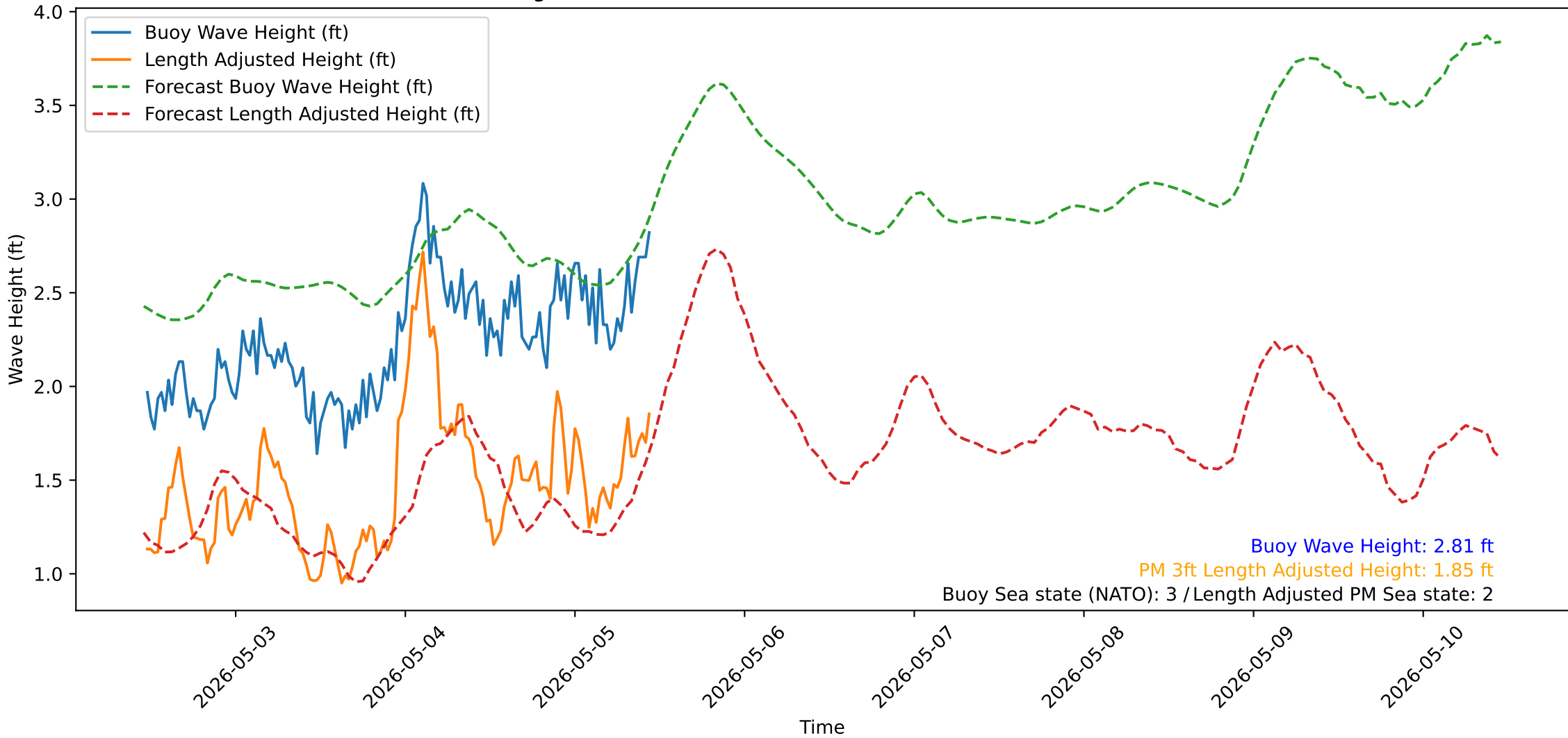
Wave Heights over Time for Oceanside Harbor at 2026-05-05 11:20:31
