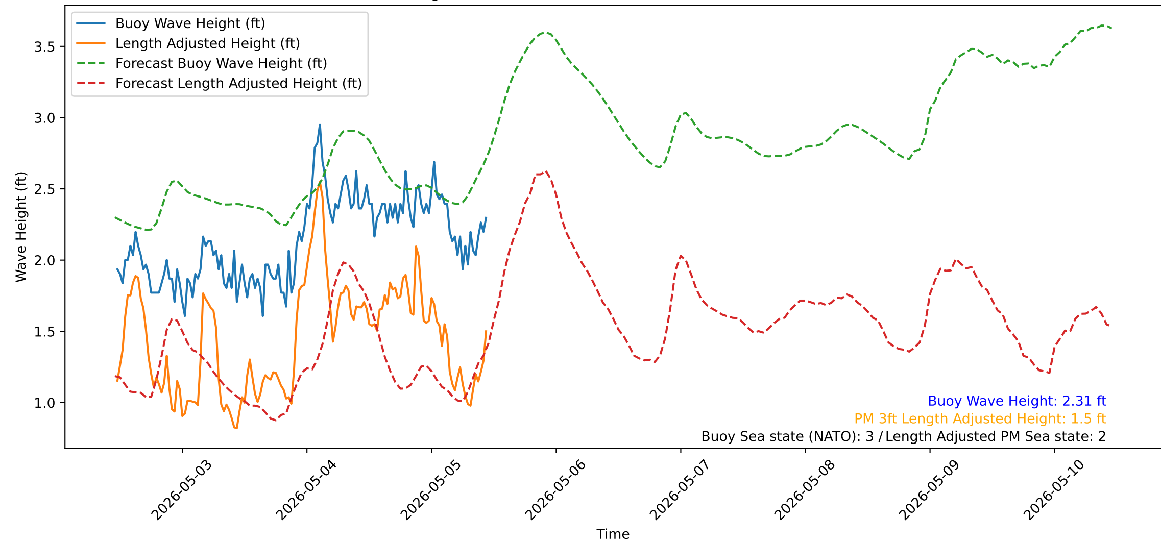
Wave Heights over Time for Red Beach at 2026-05-05 11:20:52
