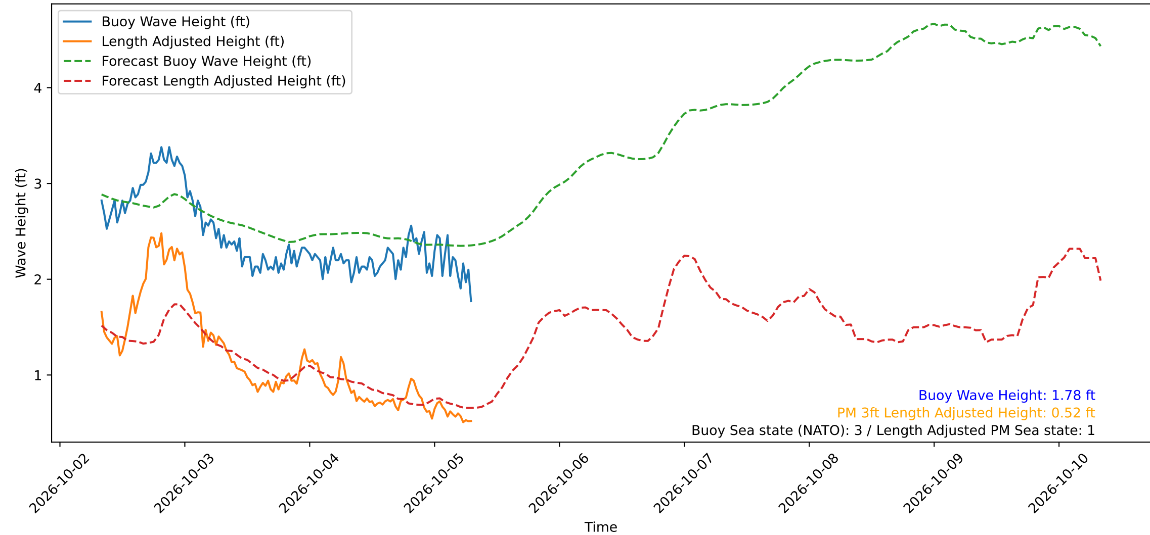
Wave Heights over Time for Green Beach at 2026-10-05 07:41:12
