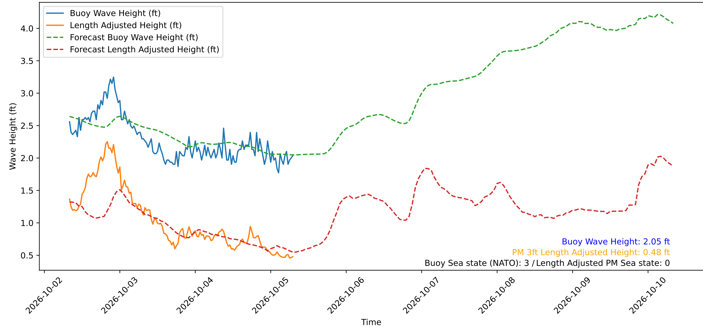
Wave Heights over Time for Red Beach at 2026-10-05 07:40:50
