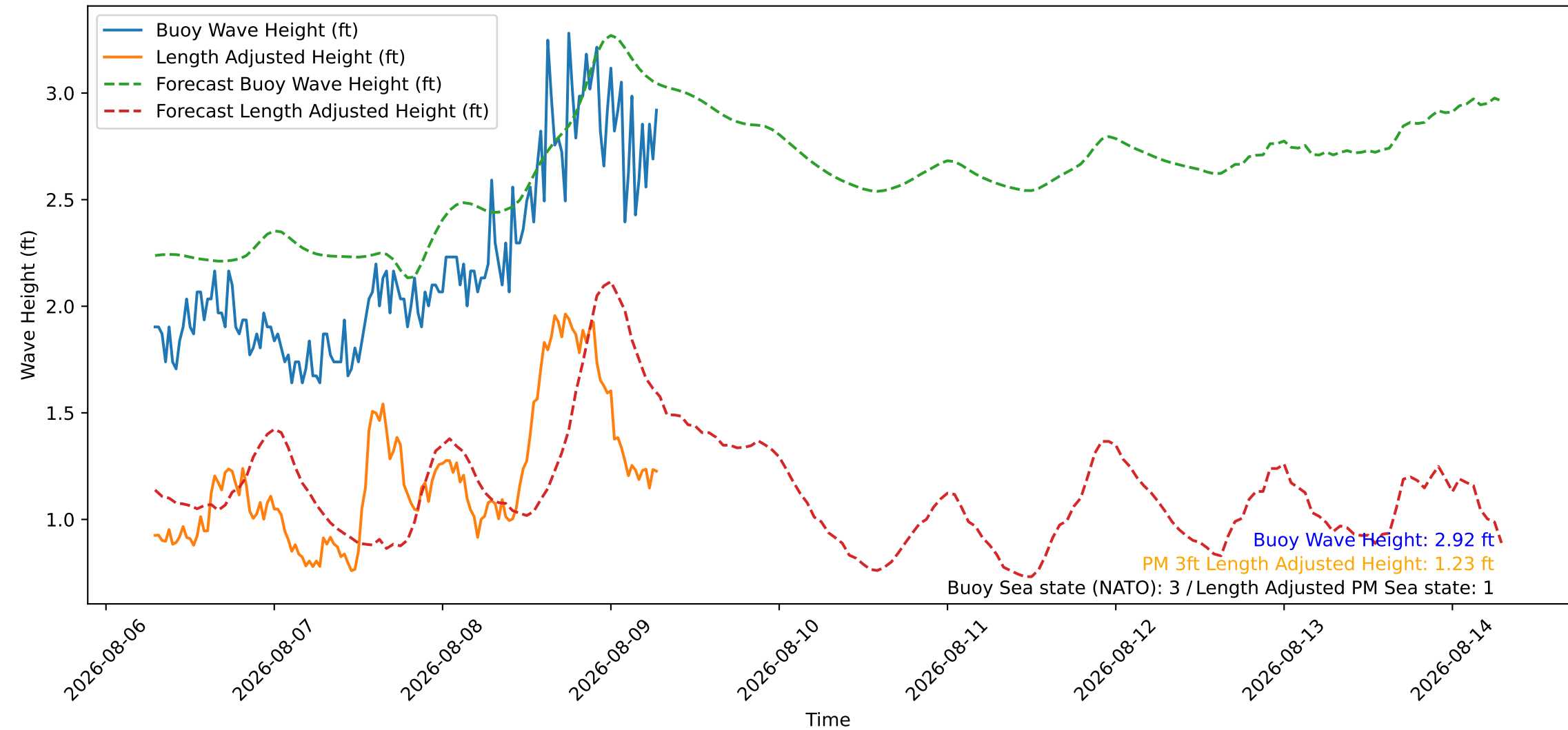
Wave Heights over Time for Oceanside Harbor at 2026-08-09 07:10:26
