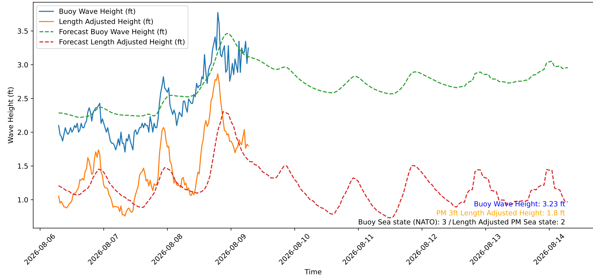
Wave Heights over Time for Green Beach at 2026-08-09 07:11:09
