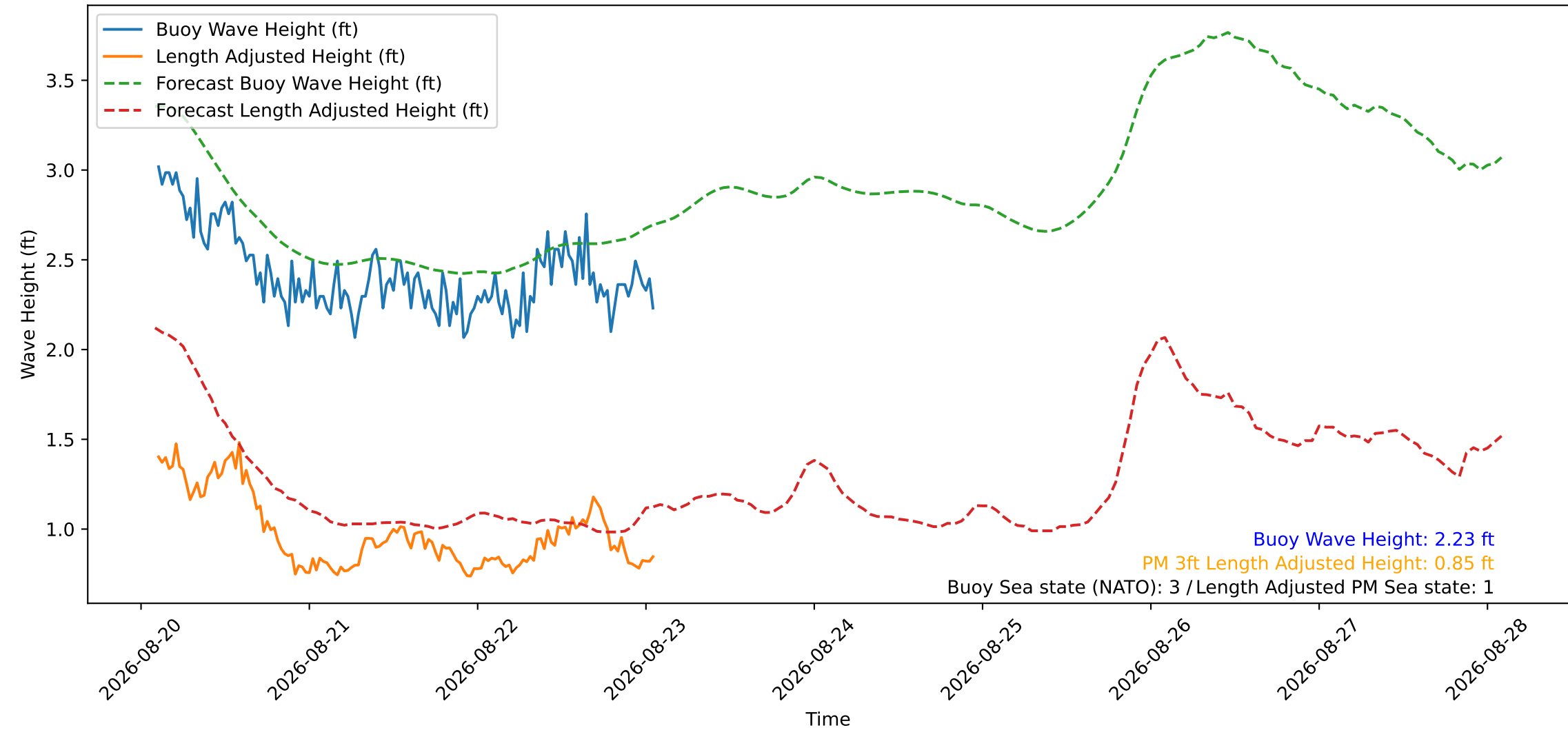
Wave Heights over Time for Red Beach at 2026-08-23 02:00:49
