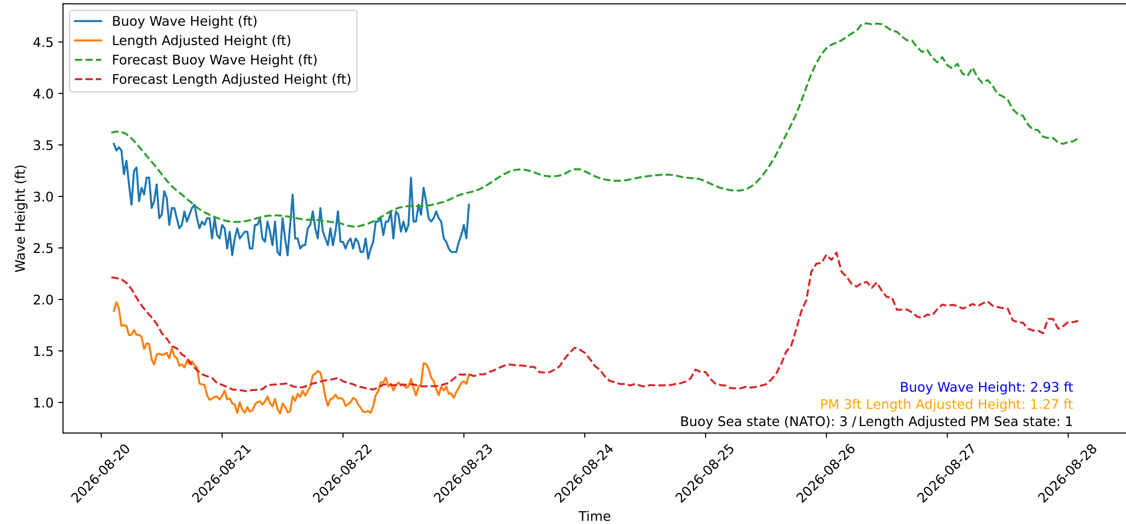
Wave Heights over Time for Green Beach at 2026-08-23 02:01:12
