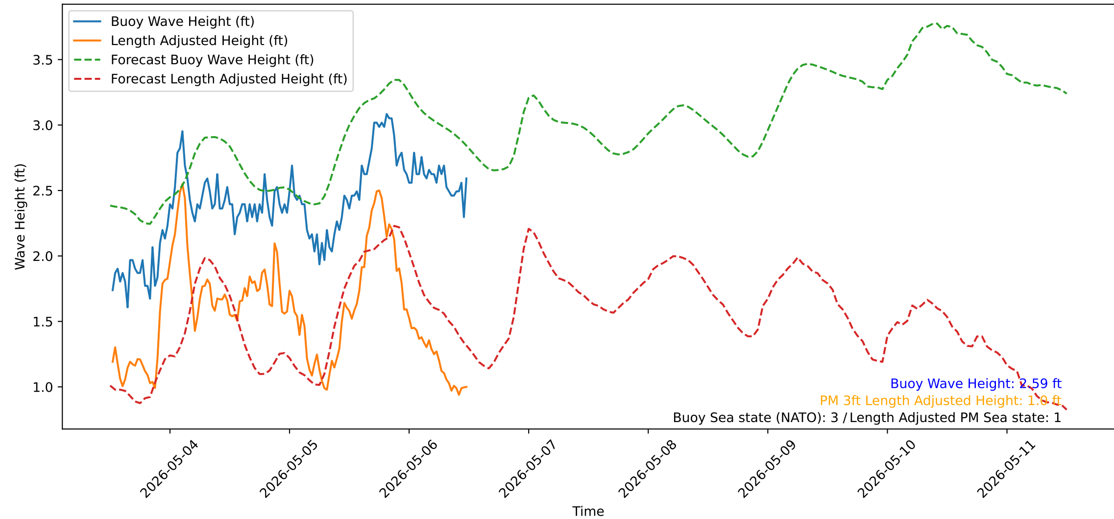
Wave Heights over Time for Red Beach at 2026-05-06 12:10:51
