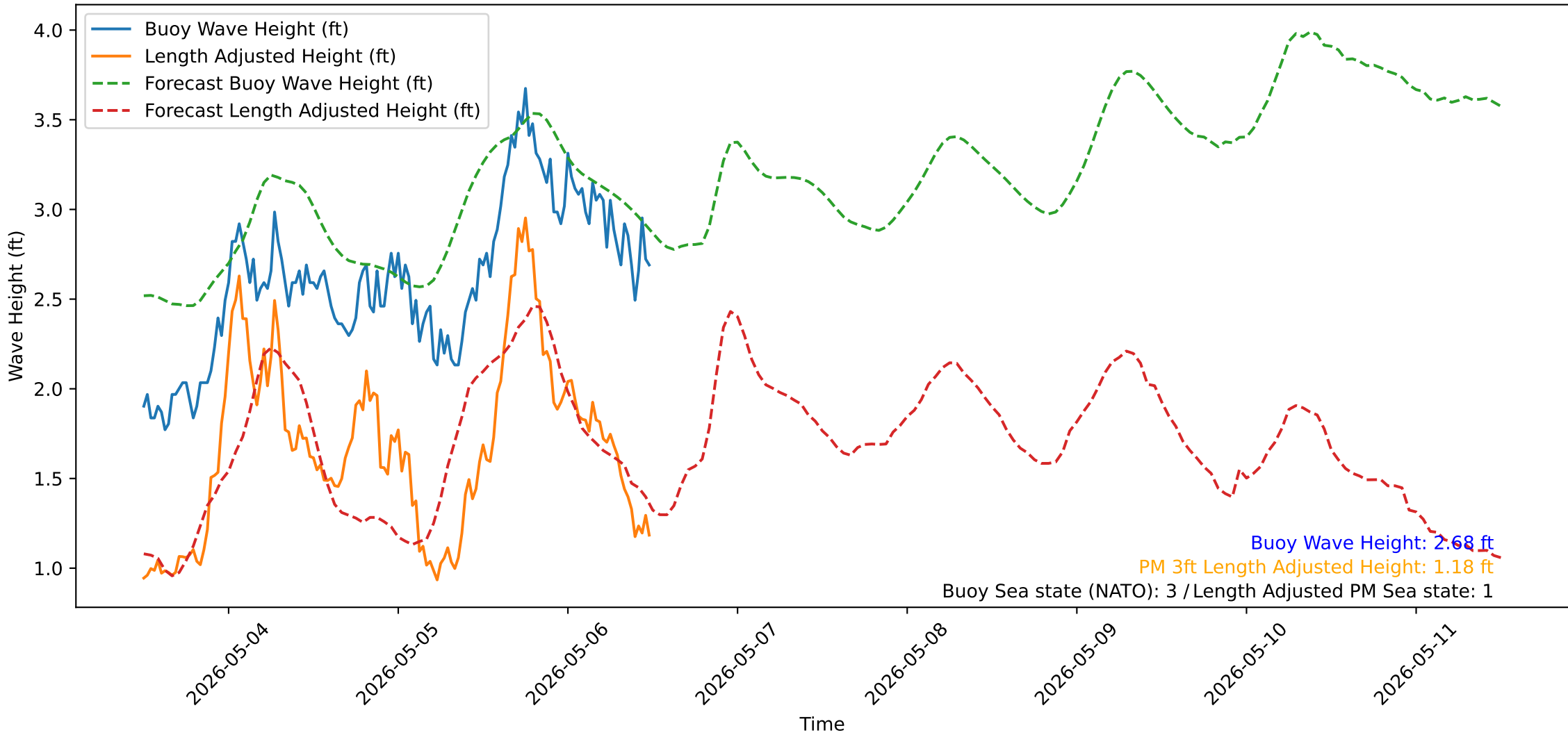
Wave Heights over Time for Green Beach at 2026-05-06 12:11:13
