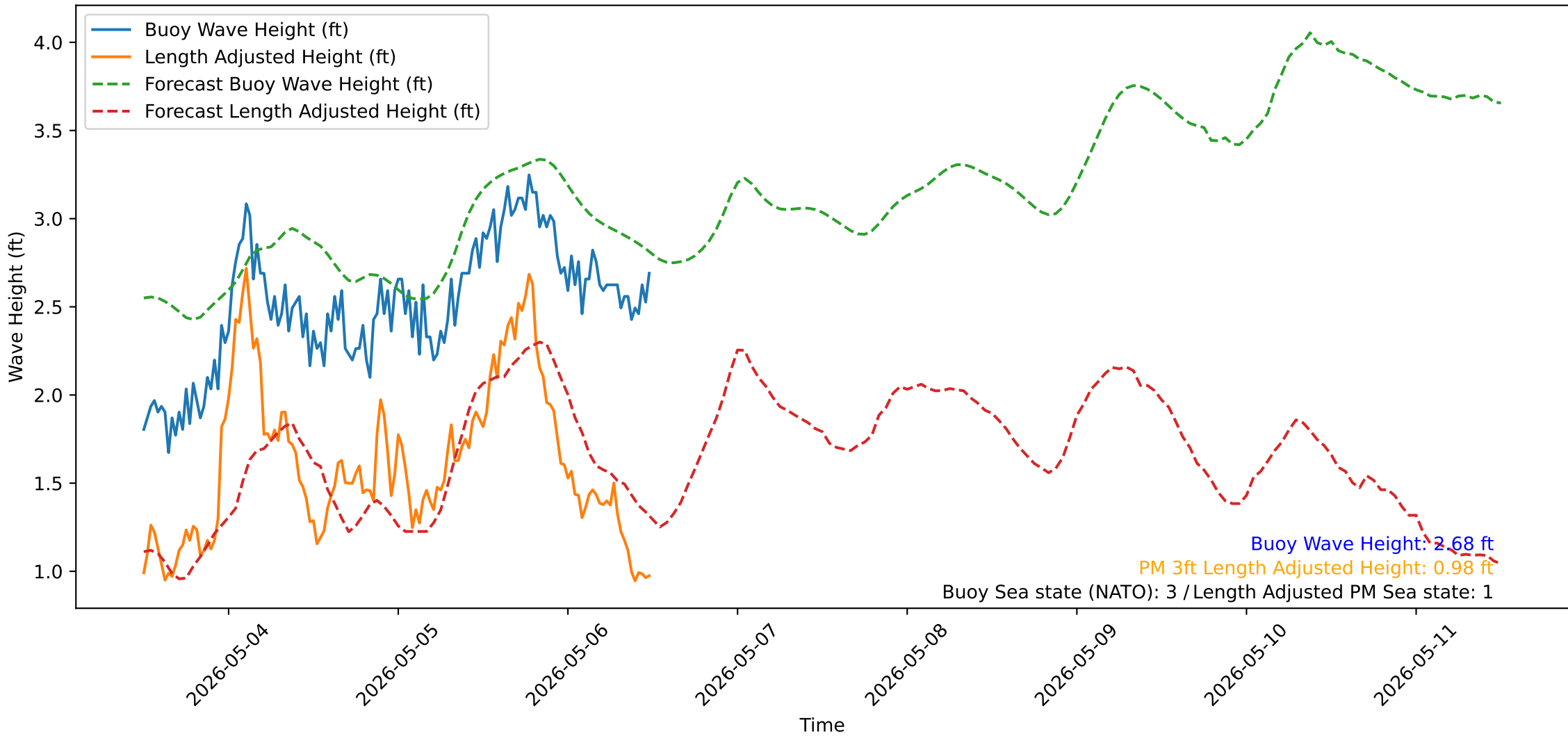
Wave Heights over Time for Oceanside Harbor at 2026-05-06 12:10:31
