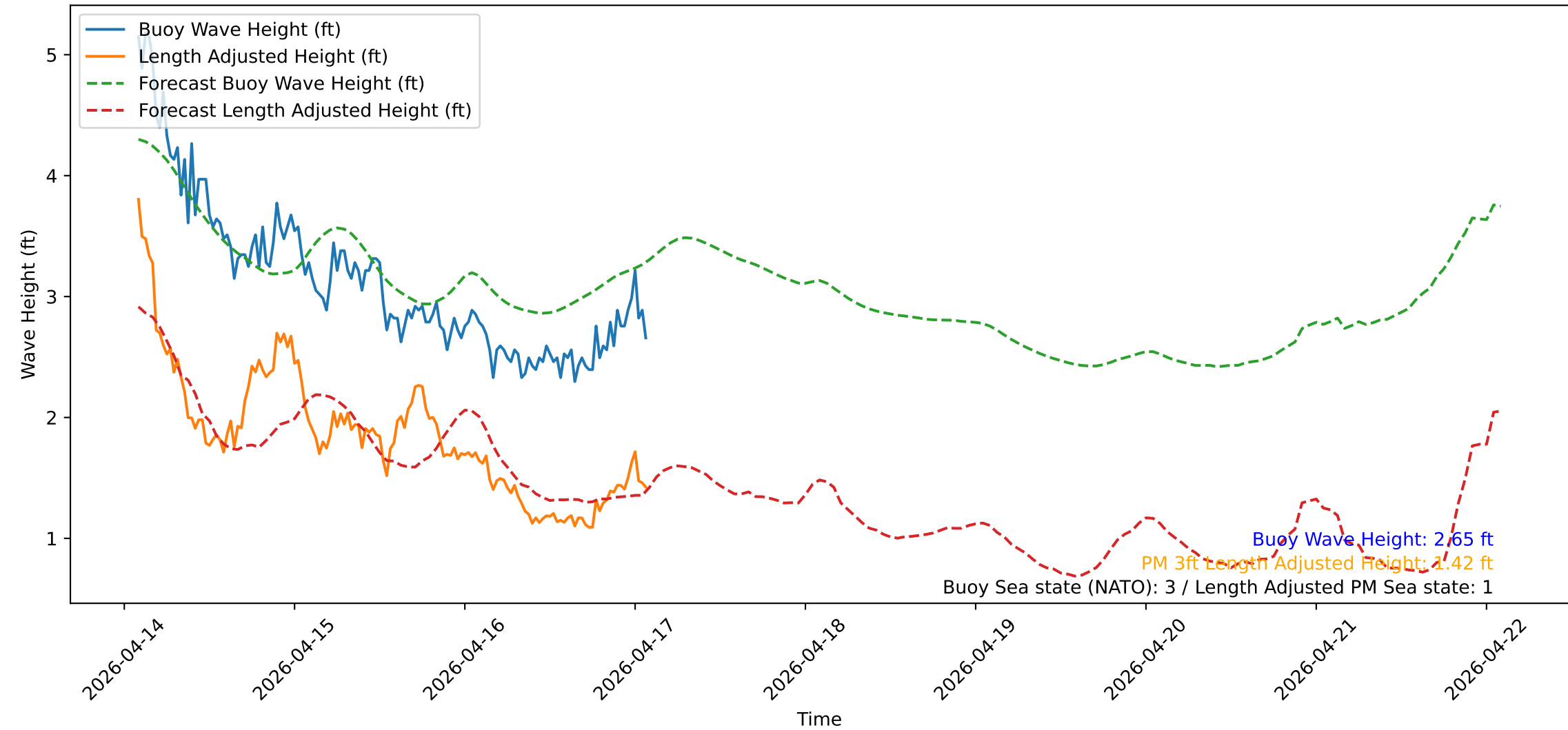
Wave Heights over Time for Oceanside Harbor at 2026-04-17 02:00:31
