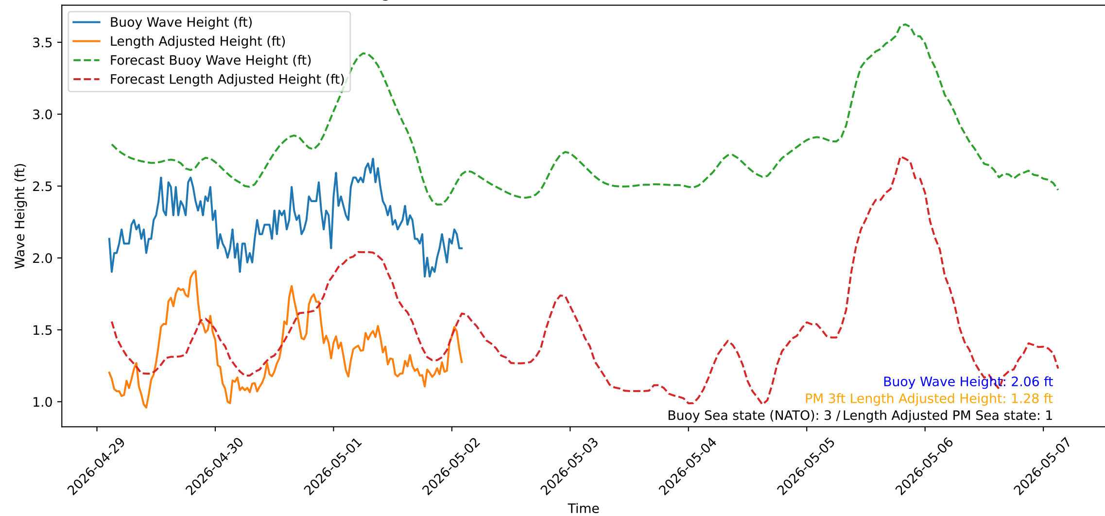
Wave Heights over Time for Oceanside Harbor at 2026-05-02 02:30:31
