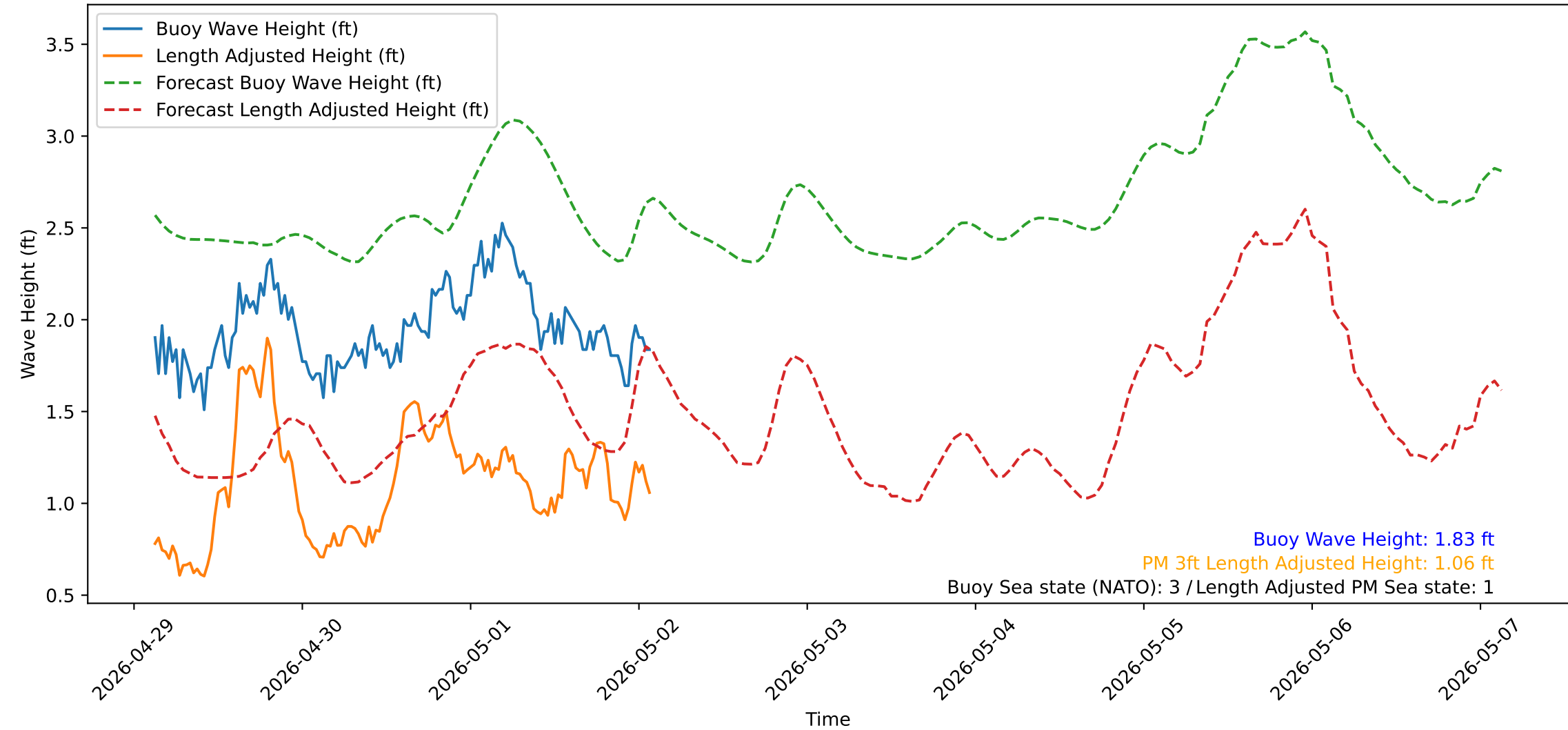
Wave Heights over Time for Red Beach at 2026-05-02 02:30:50
