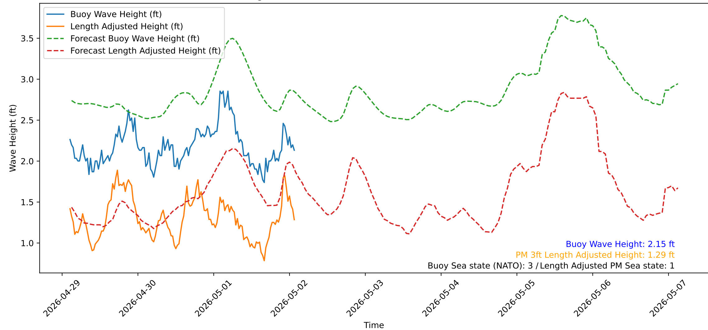
Wave Heights over Time for Green Beach at 2026-05-02 02:31:12
