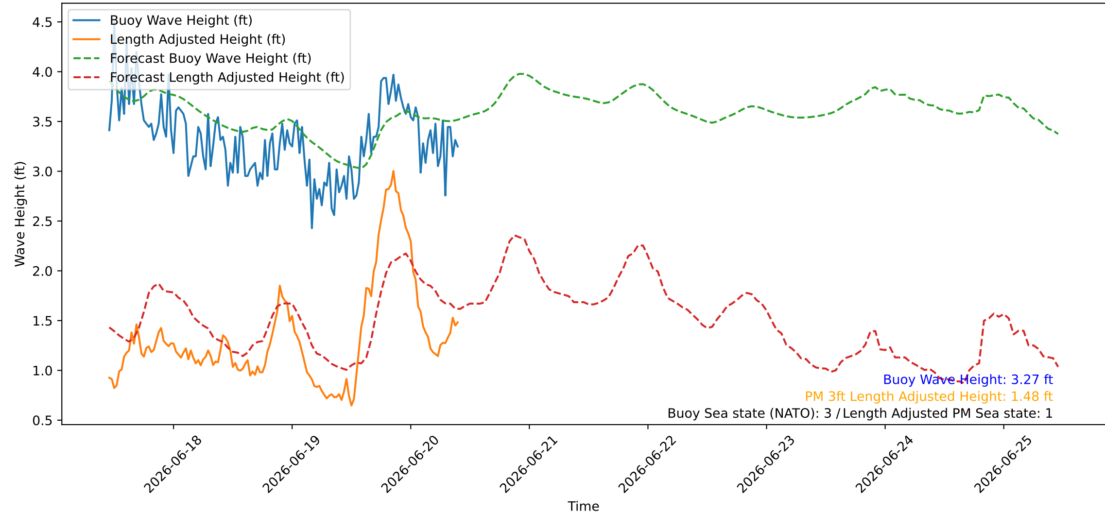
Wave Heights over Time for Green Beach at 2026-06-20 10:51:08
