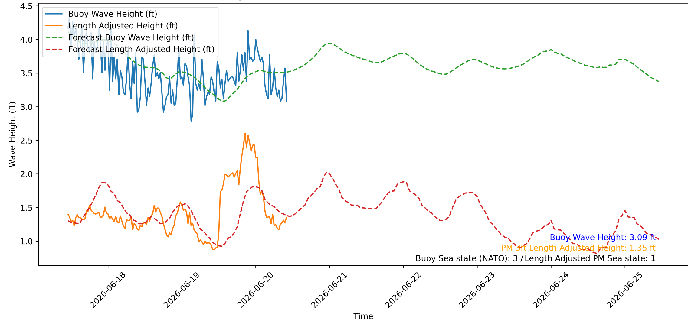
Wave Heights over Time for Oceanside Harbor at 2026-06-20 10:50:26
