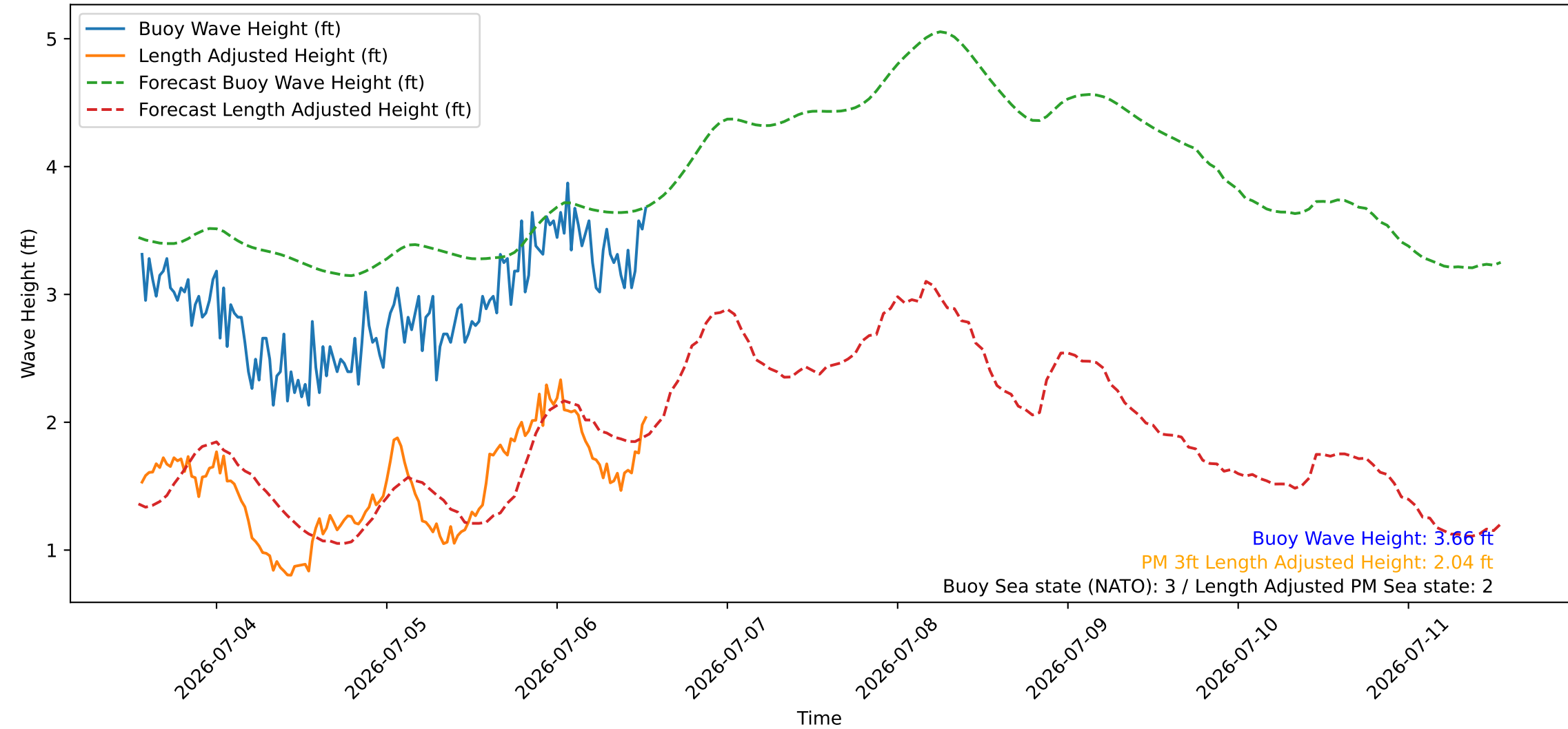
Wave Heights over Time for Oceanside Harbor at 2026-07-06 13:20:26
