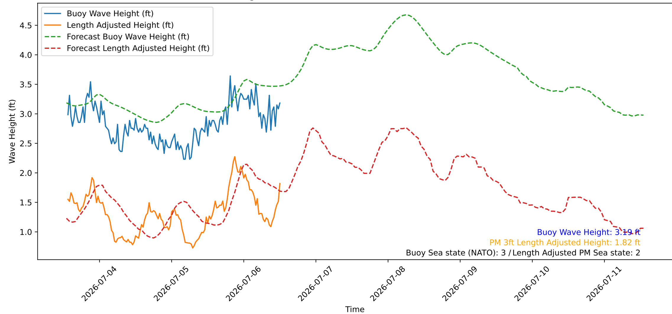
Wave Heights over Time for Red Beach at 2026-07-06 13:20:48
