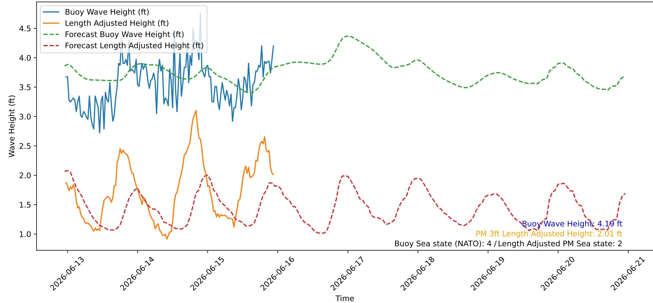
Wave Heights over Time for Red Beach at 2026-06-15 23:20:47
