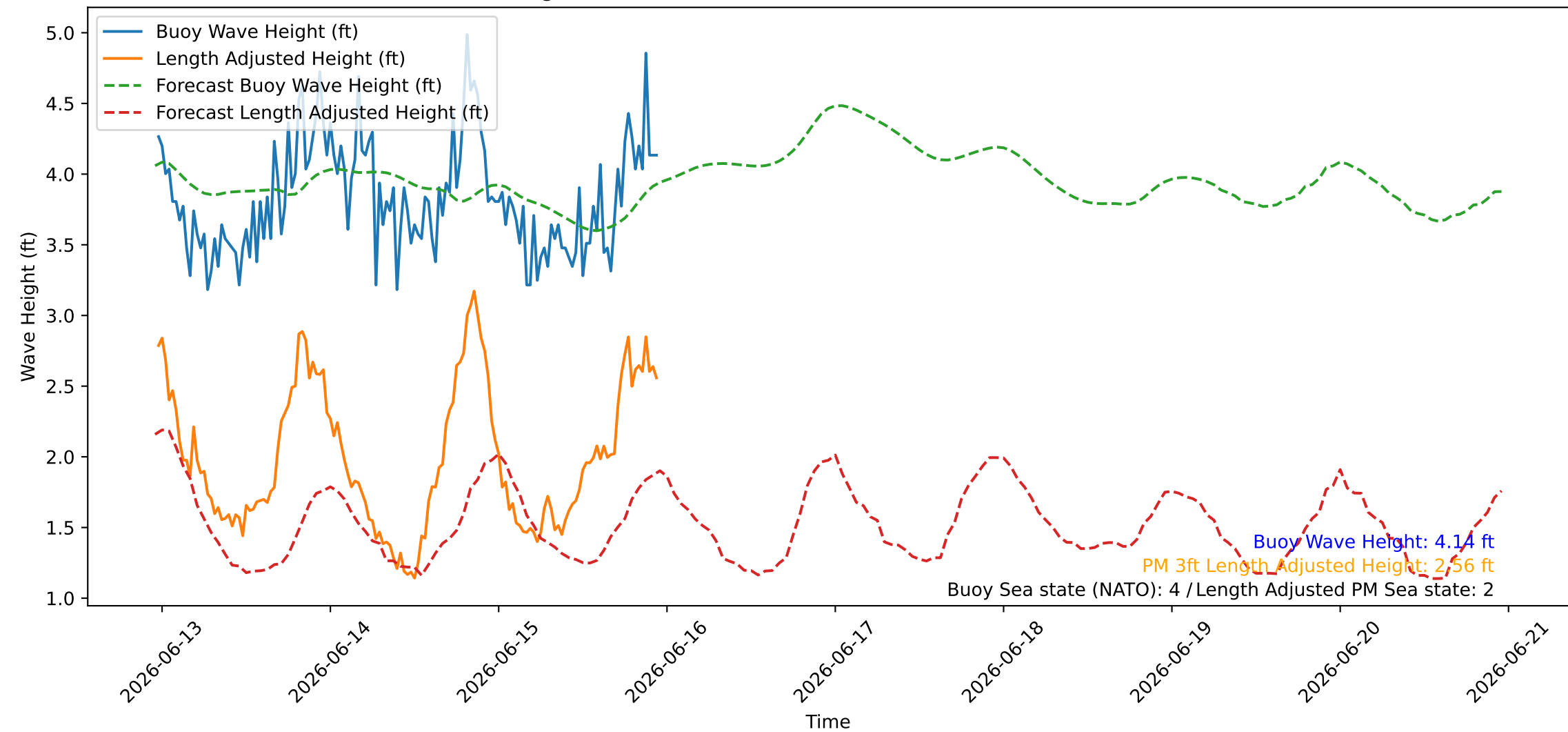
Wave Heights over Time for Oceanside Harbor at 2026-06-15 23:20:26
