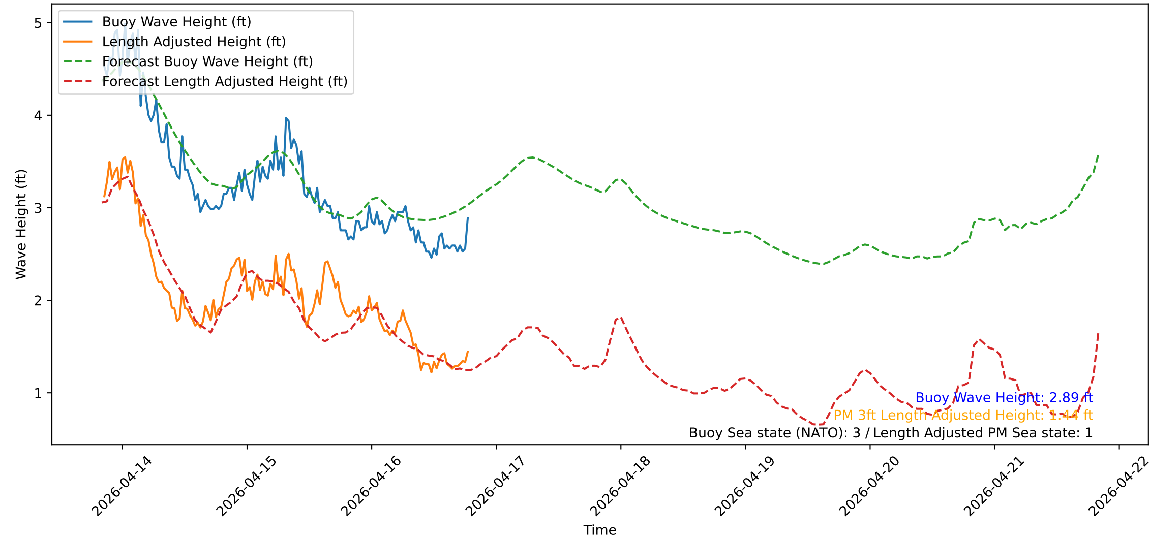
Wave Heights over Time for Green Beach at 2026-04-16 20:21:14
