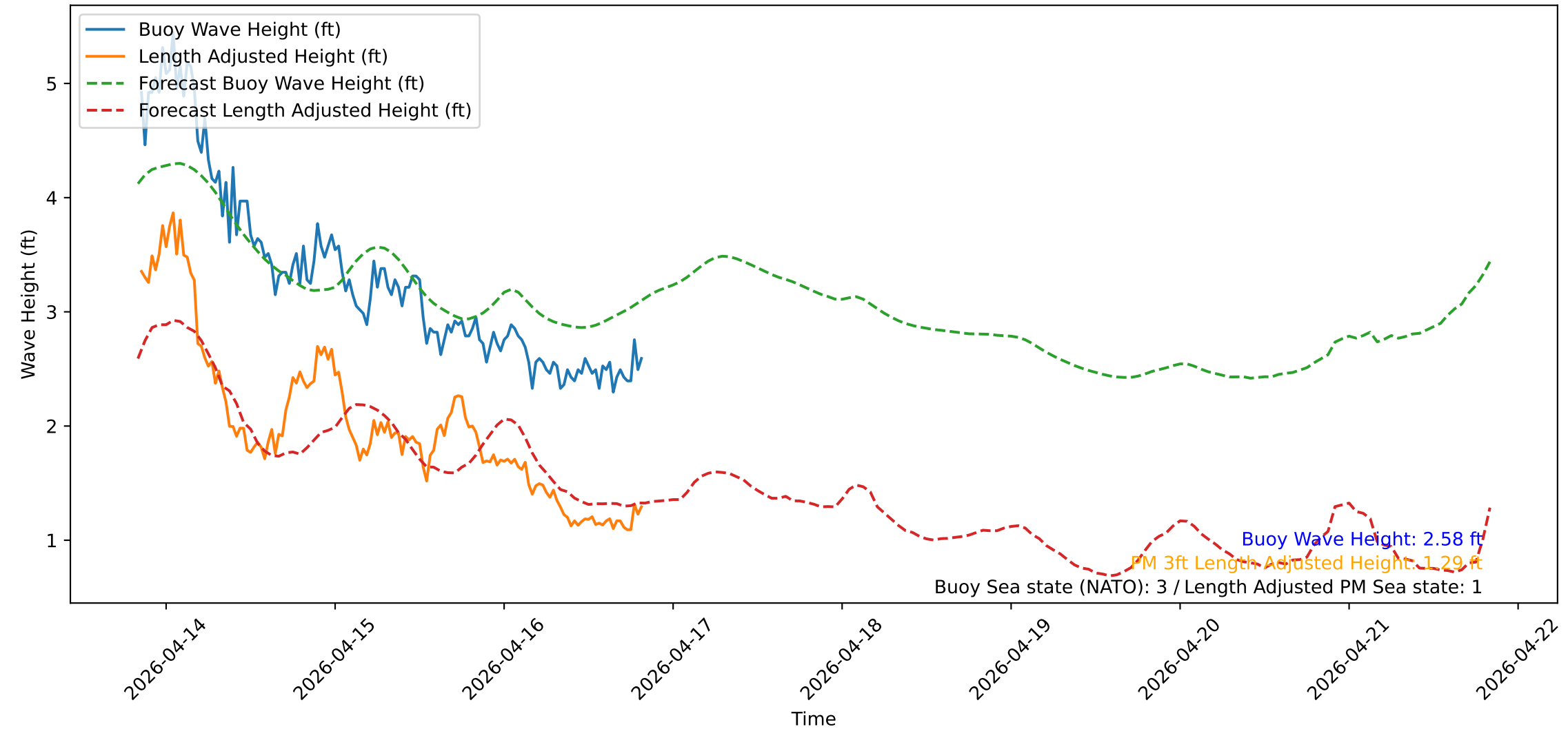
Wave Heights over Time for Oceanside Harbor at 2026-04-16 20:20:31
