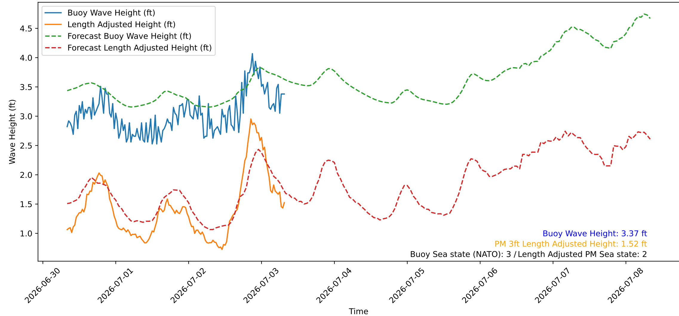
Wave Heights over Time for Green Beach at 2026-07-03 08:11:07
