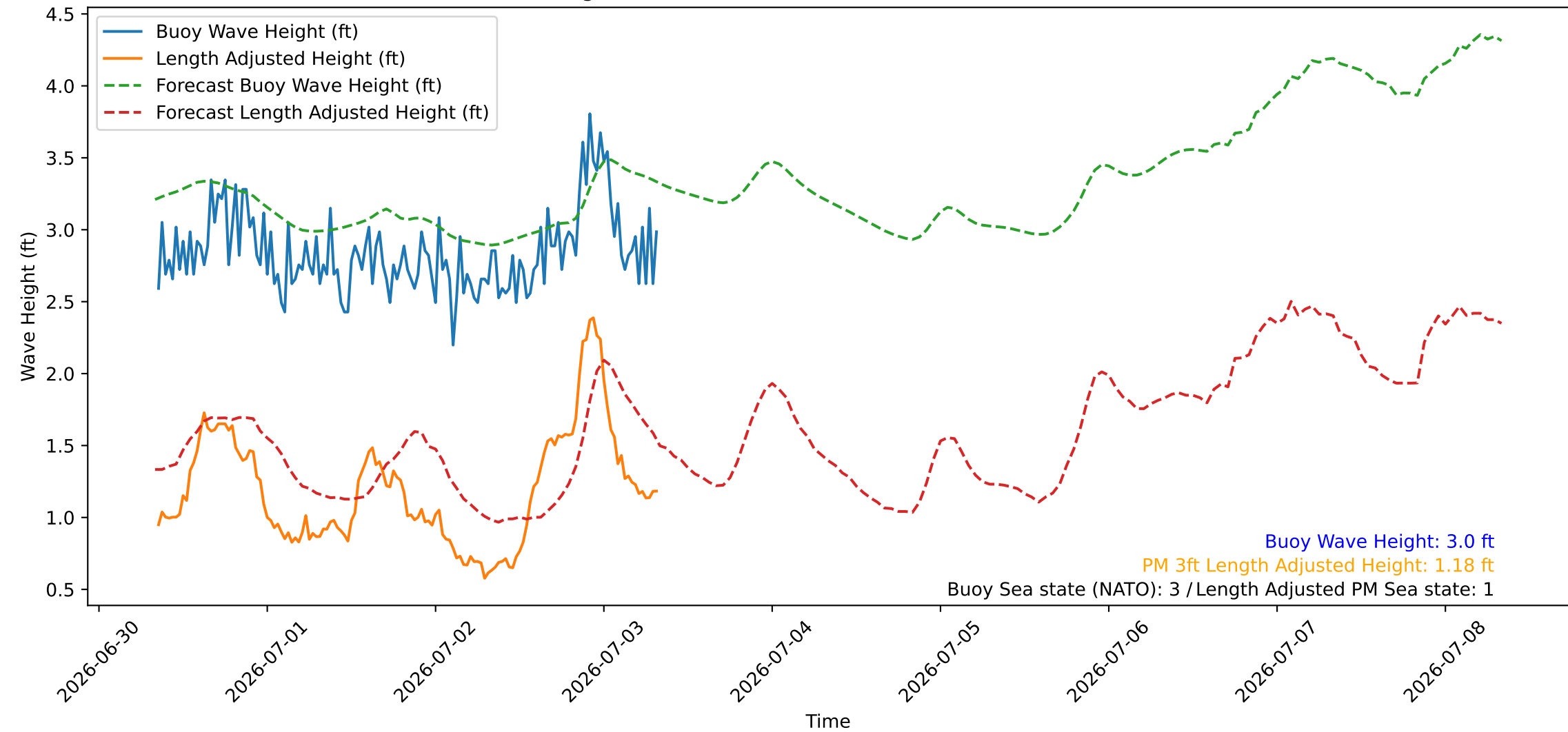
Wave Heights over Time for Red Beach at 2026-07-03 08:10:45
