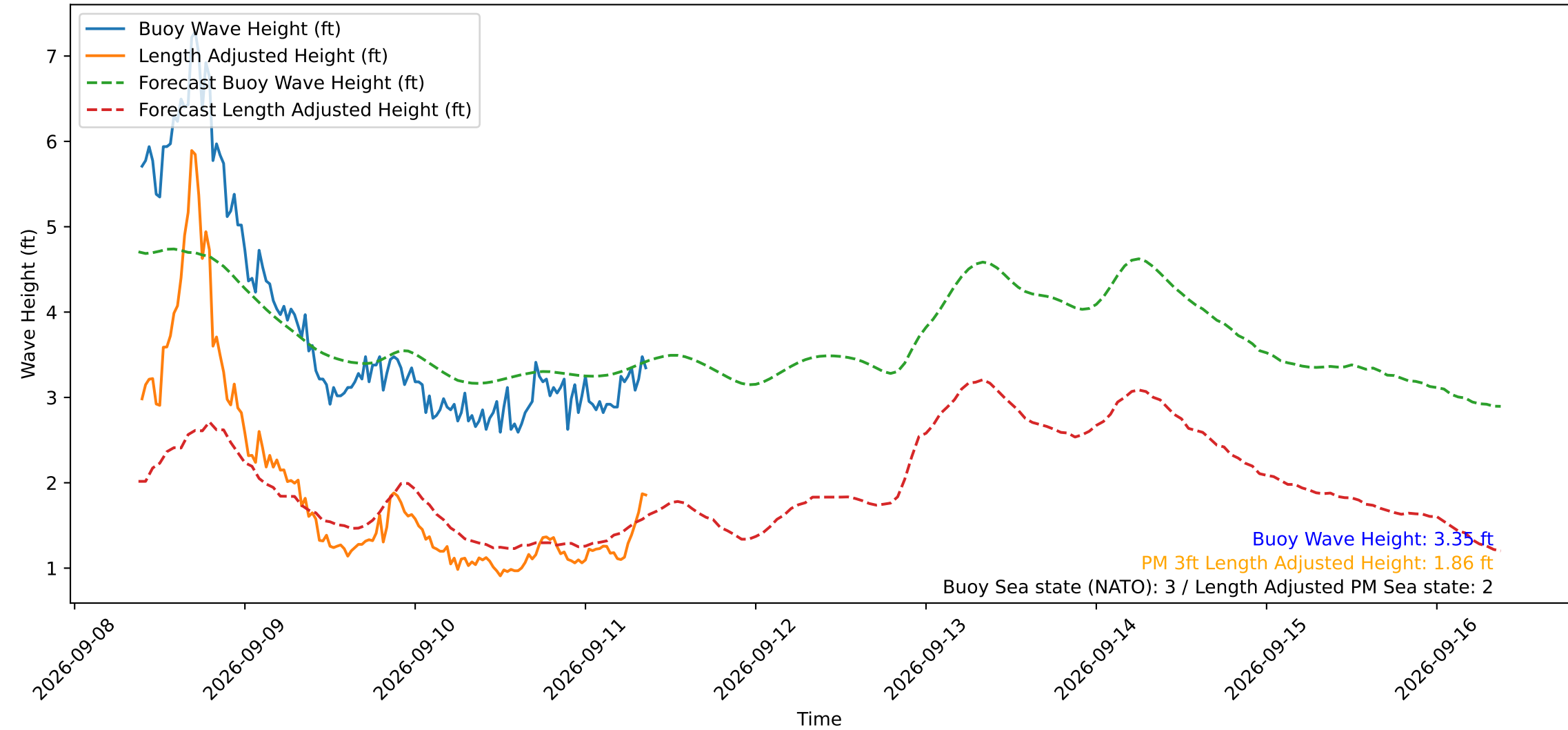
Wave Heights over Time for Green Beach at 2026-09-11 09:21:14
