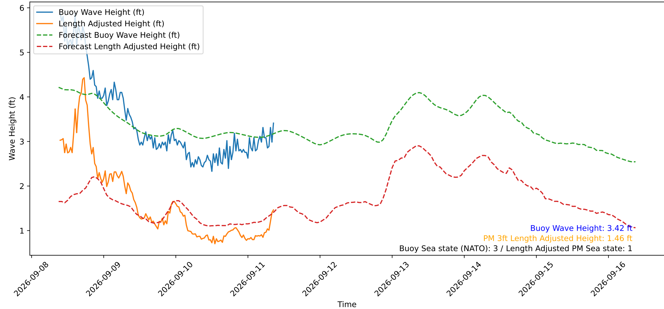
Wave Heights over Time for Red Beach at 2026-09-11 09:20:50
