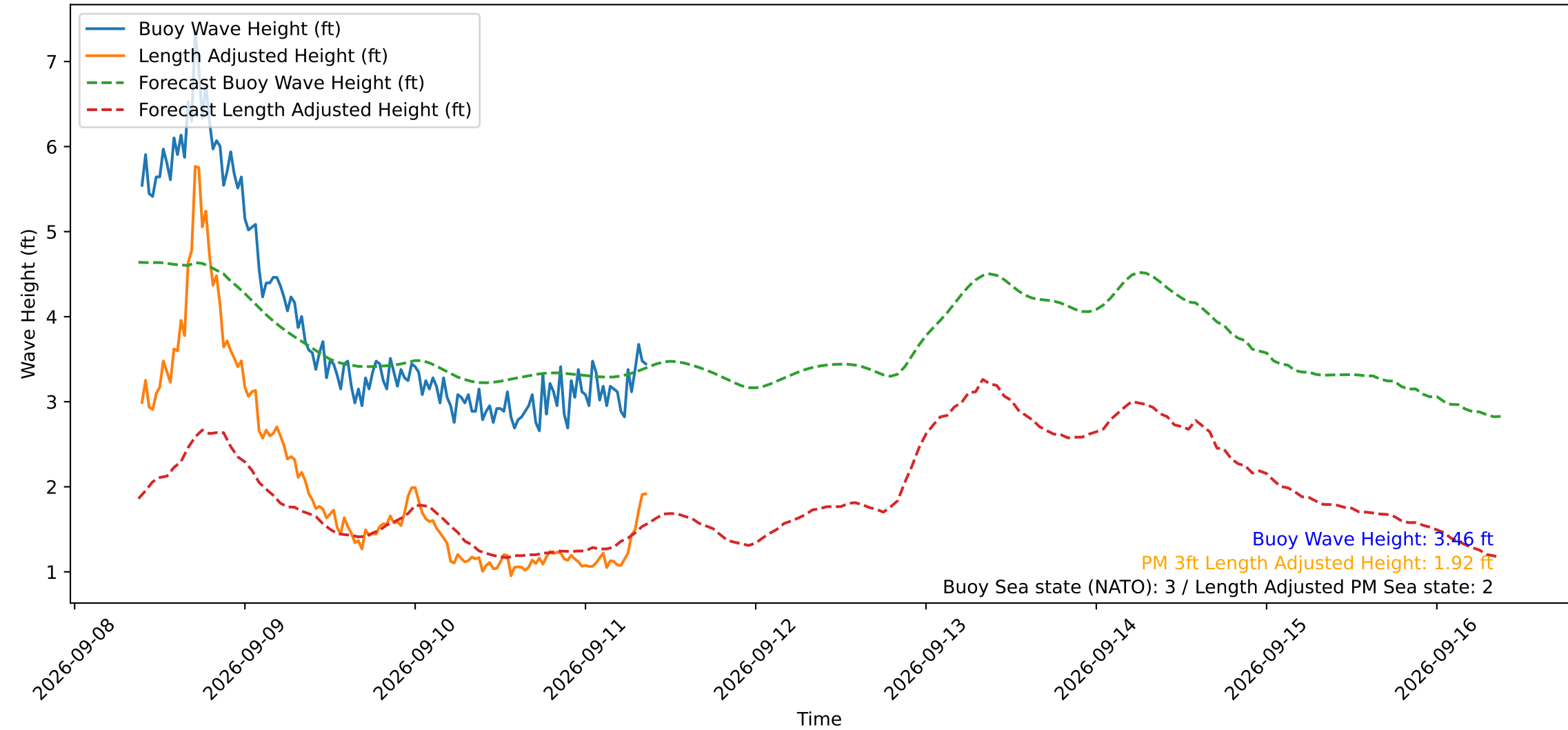
Wave Heights over Time for Oceanside Harbor at 2026-09-11 09:20:29
