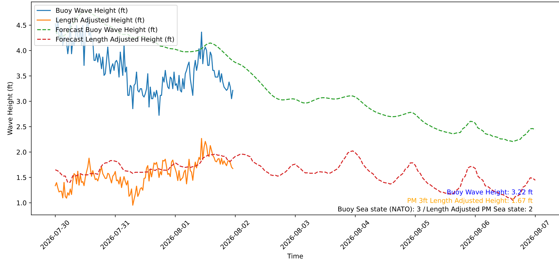
Wave Heights over Time for Oceanside Harbor at 2026-08-01 23:50:26
