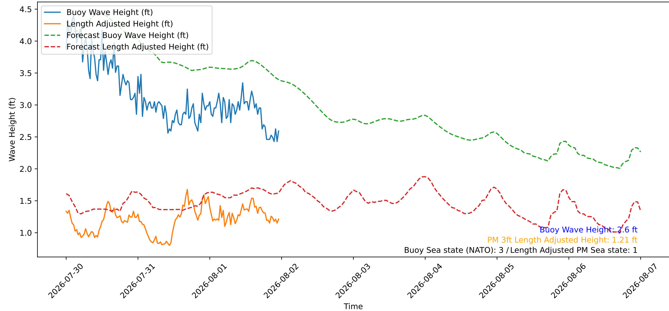
Wave Heights over Time for Red Beach at 2026-08-01 23:50:48
