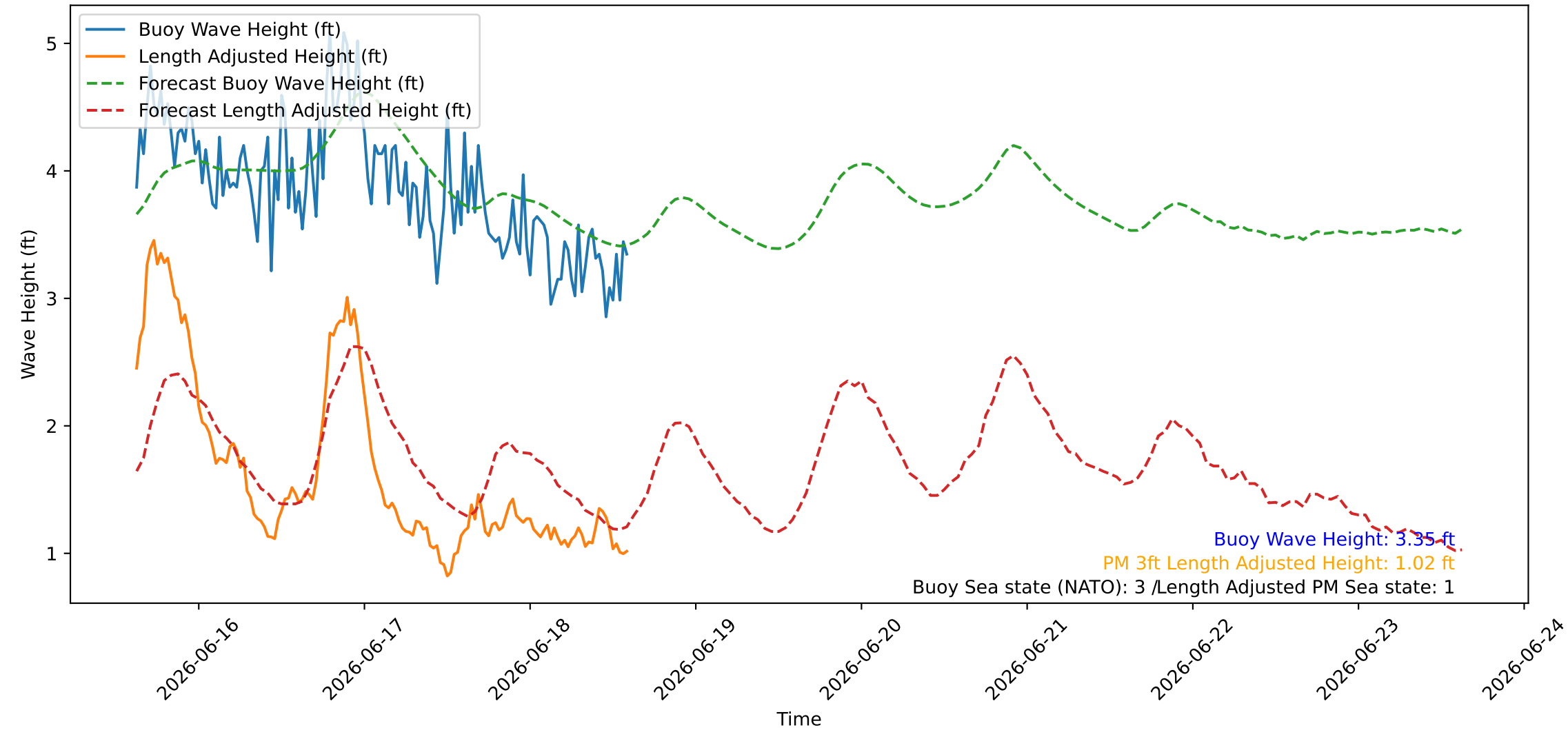
Wave Heights over Time for Green Beach at 2026-06-18 14:51:09
