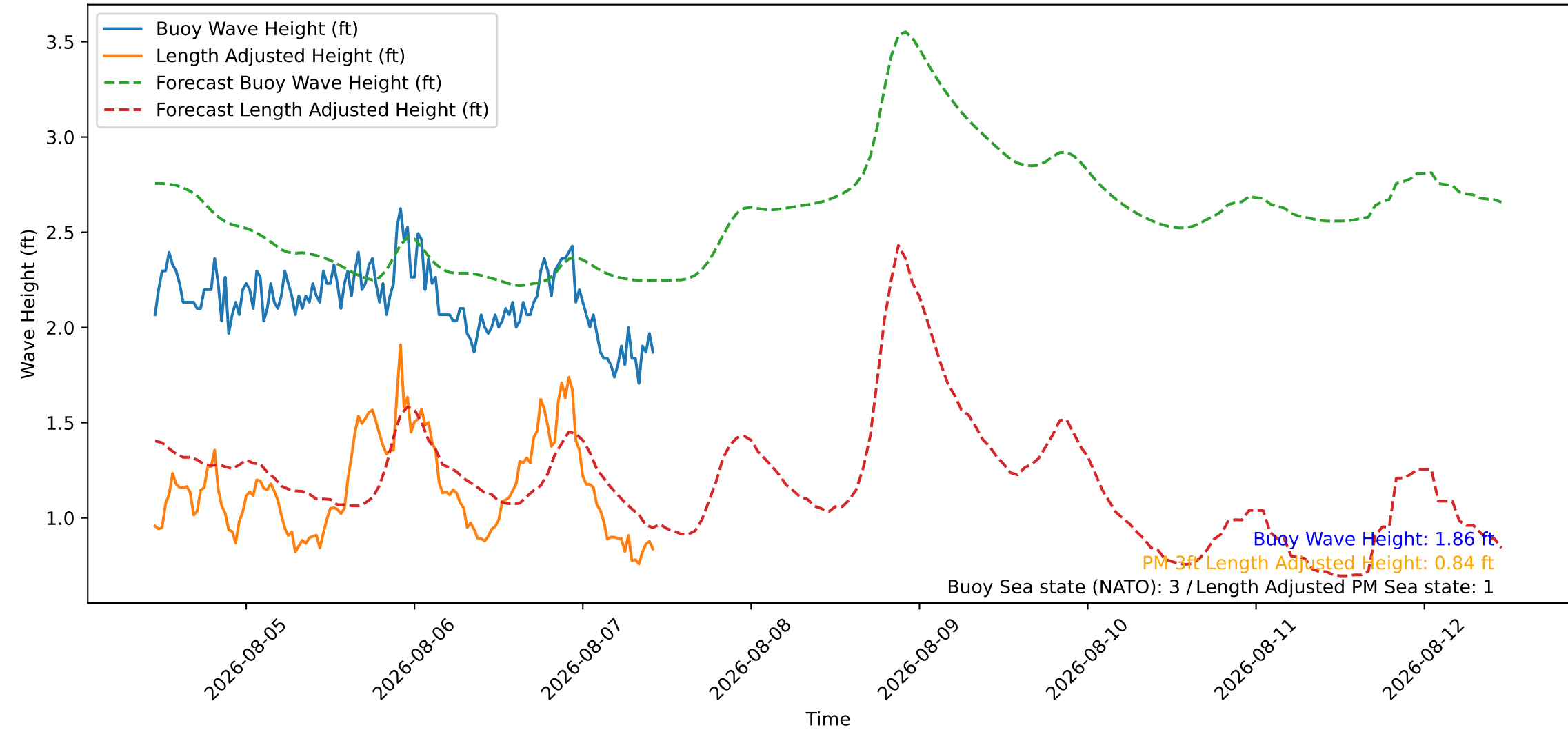
Wave Heights over Time for Green Beach at 2026-08-07 10:51:09
