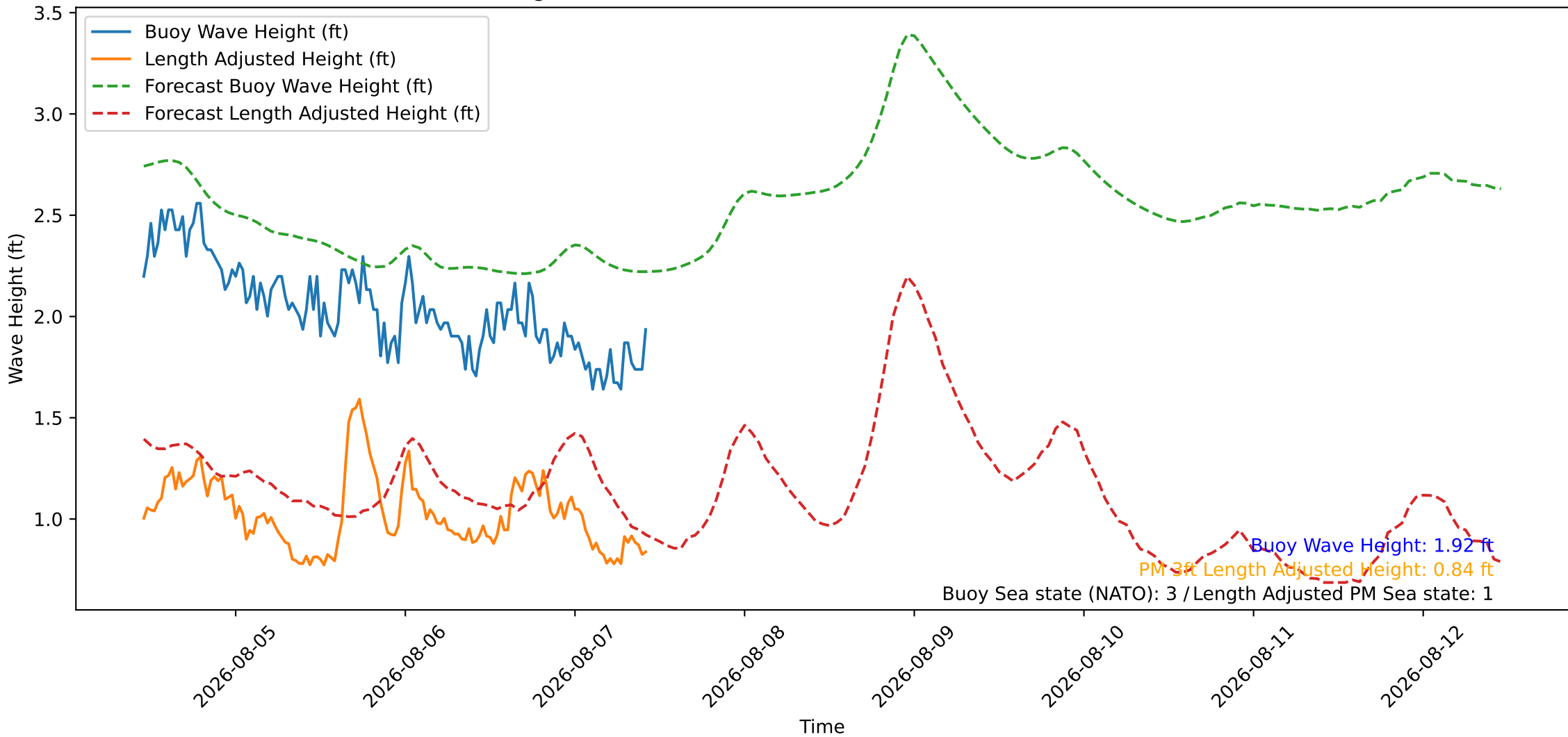
Wave Heights over Time for Oceanside Harbor at 2026-08-07 10:50:26
