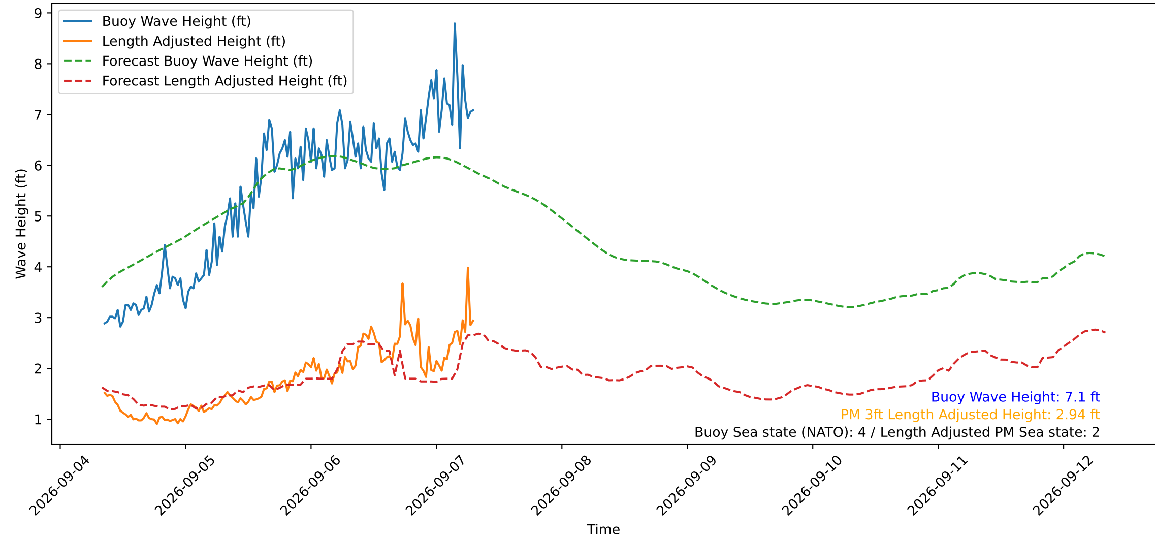
Wave Heights over Time for Green Beach at 2026-09-07 08:01:12
