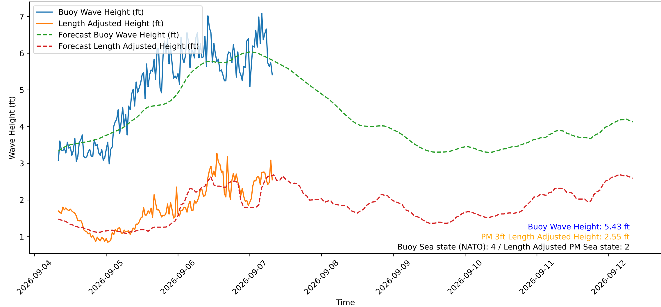
Wave Heights over Time for Oceanside Harbor at 2026-09-07 08:00:30
