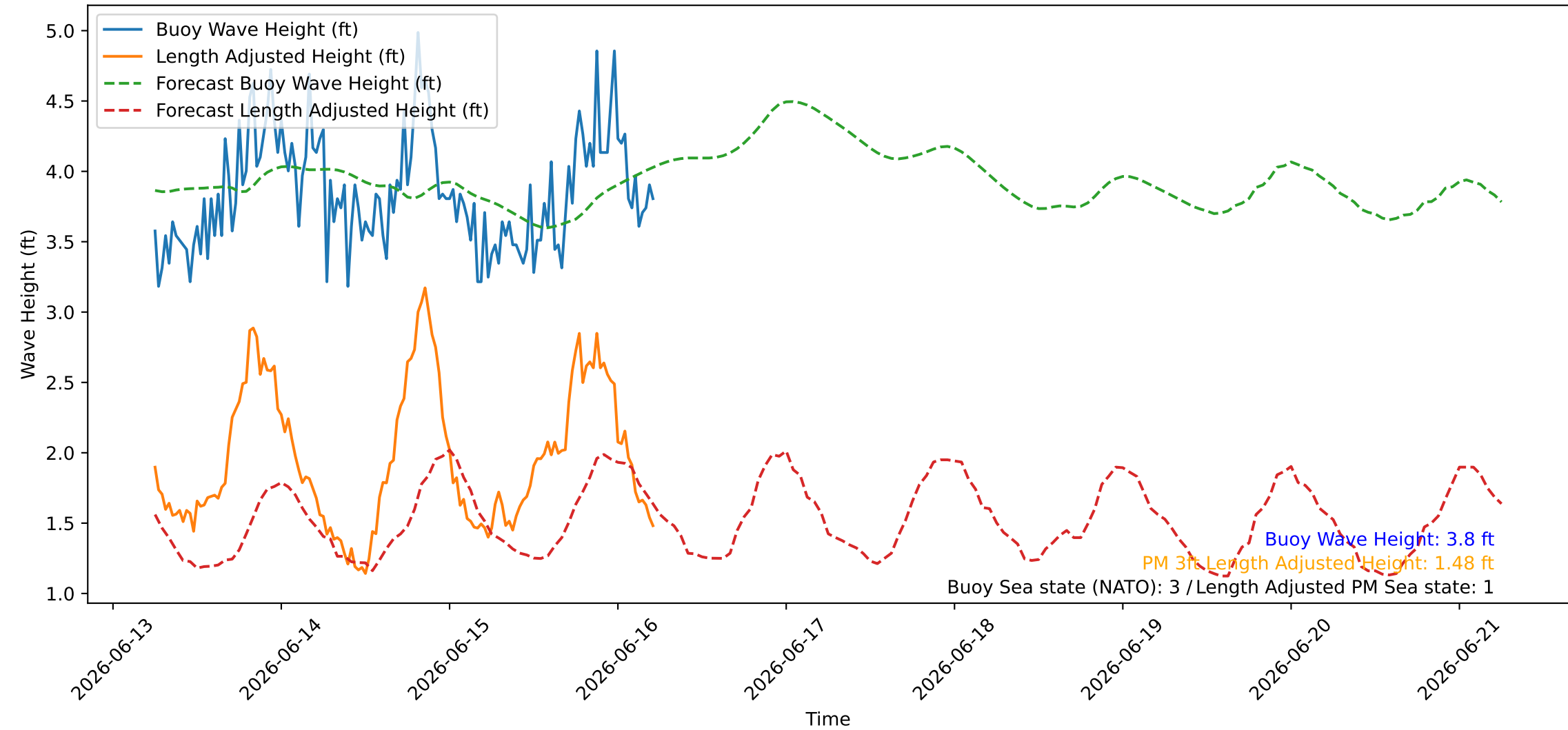
Wave Heights over Time for Oceanside Harbor at 2026-06-16 06:00:26
