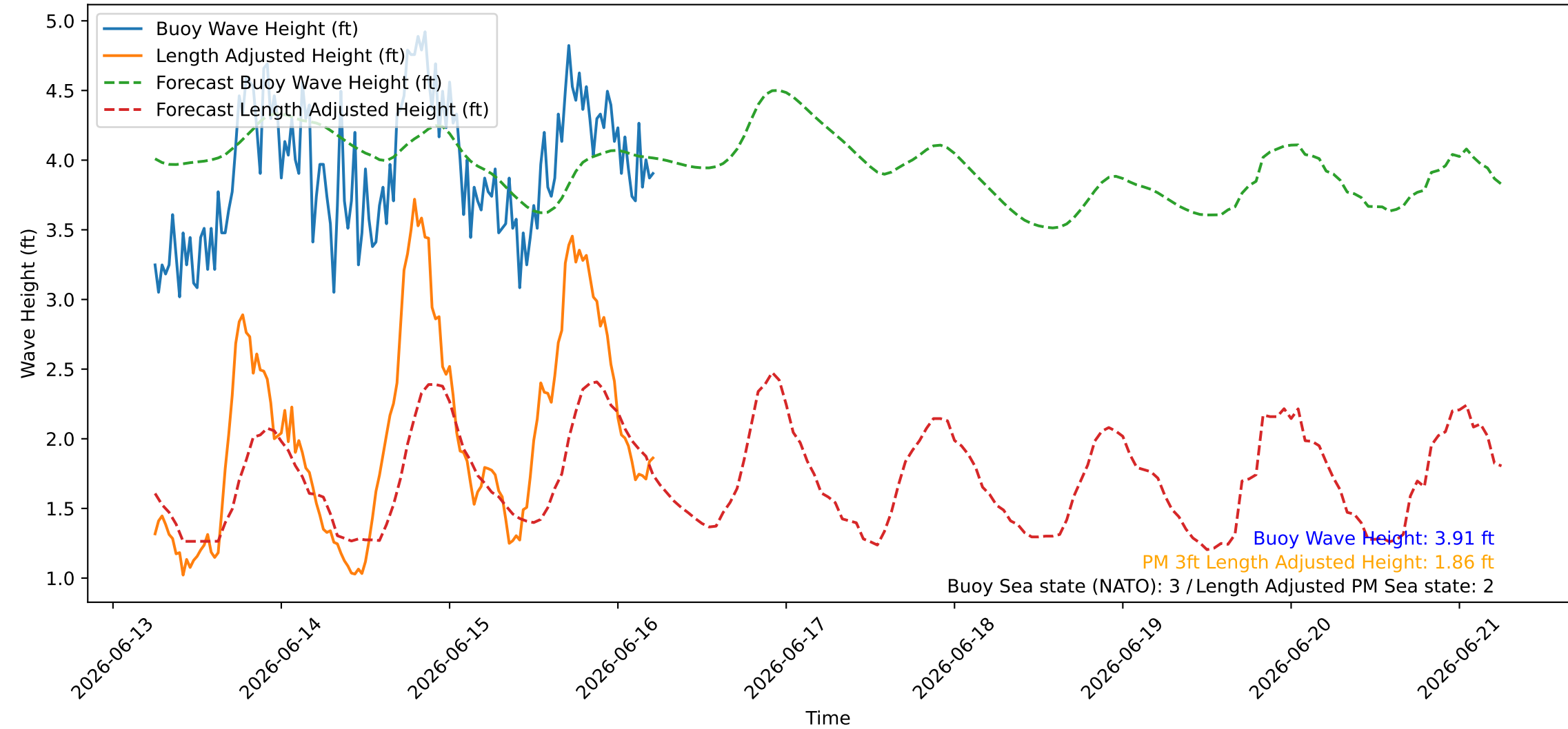
Wave Heights over Time for Green Beach at 2026-06-16 06:01:07
