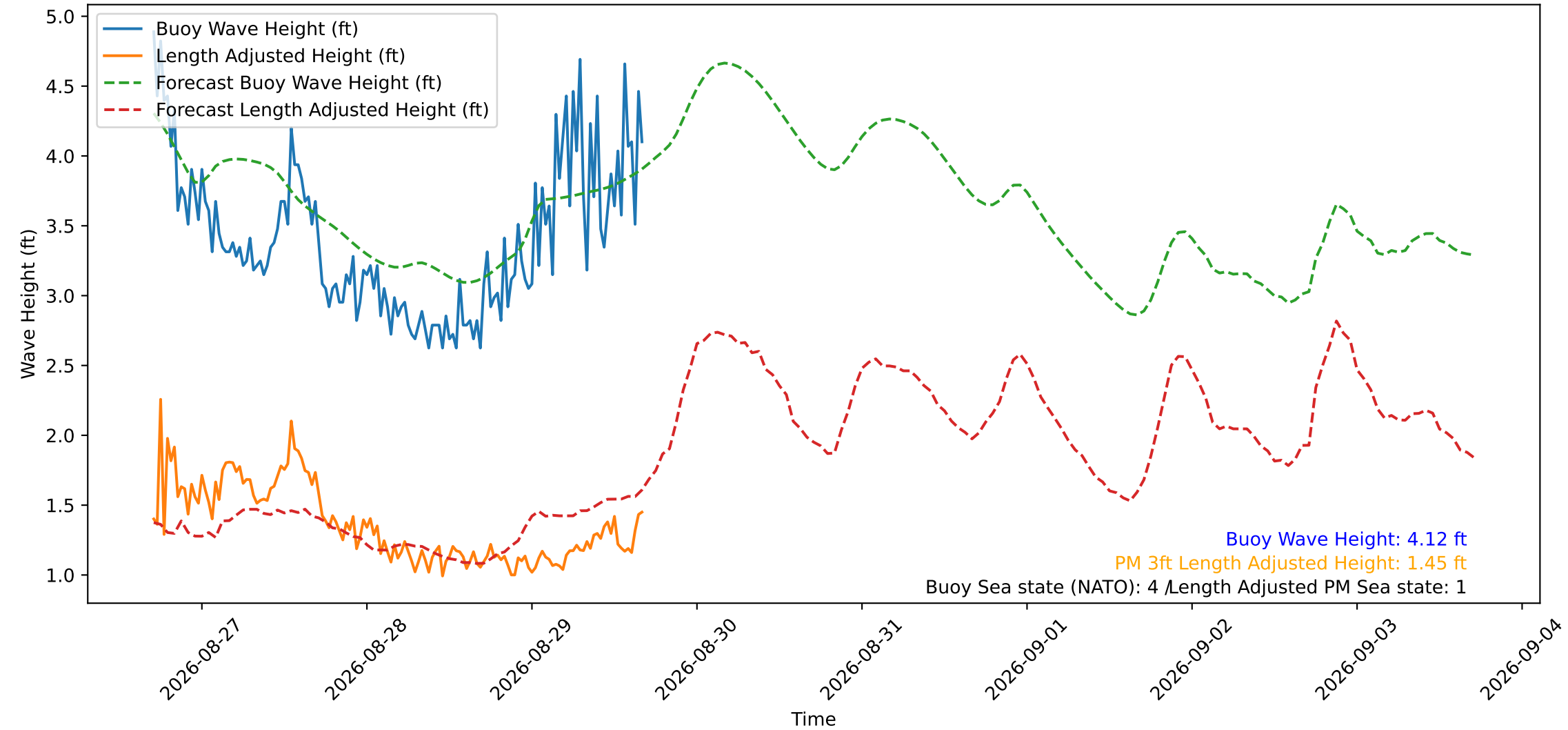
Wave Heights over Time for Red Beach at 2026-08-29 16:40:49
