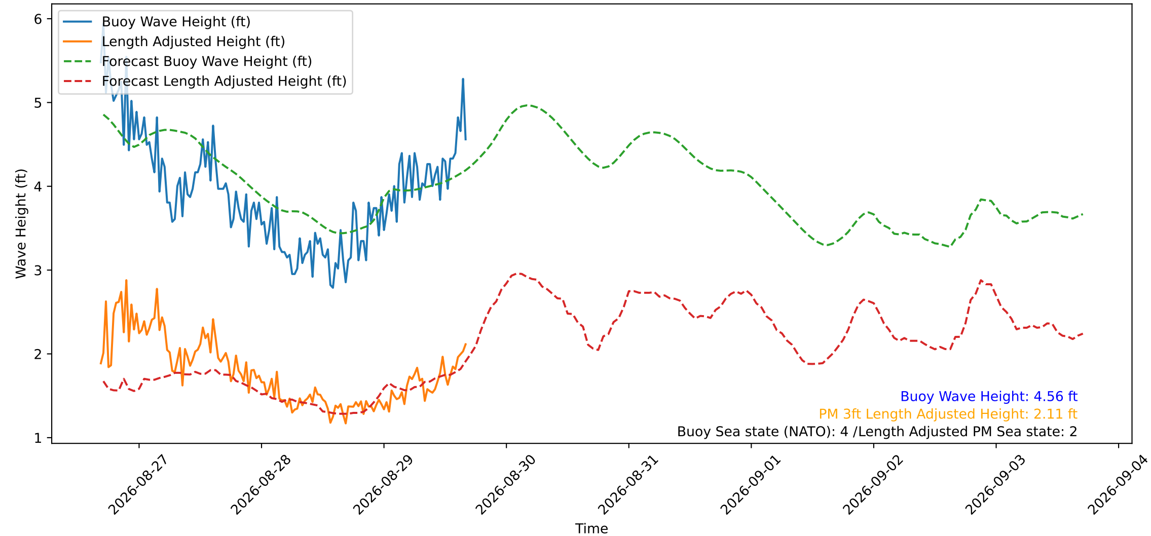
Wave Heights over Time for Oceanside Harbor at 2026-08-29 16:40:29
