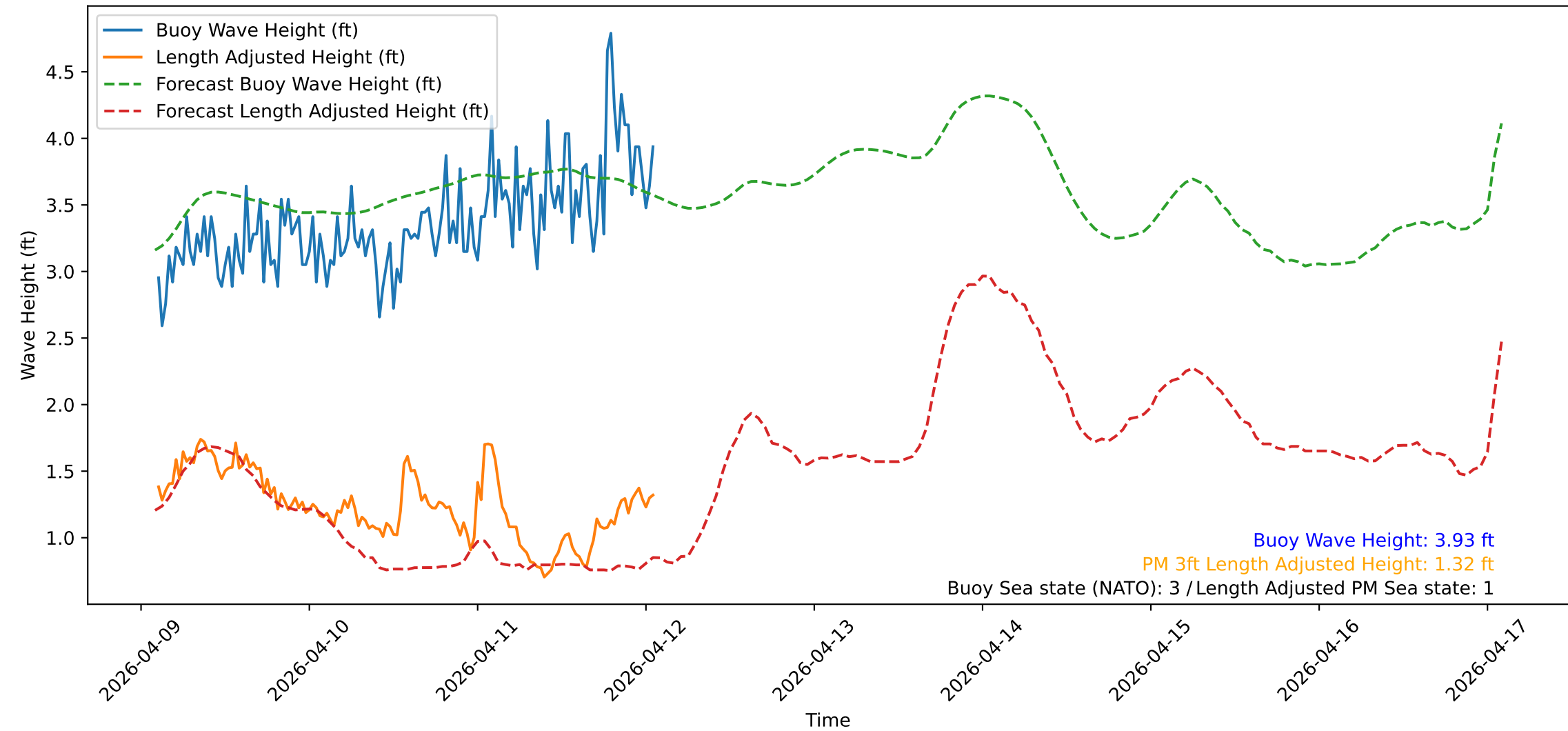
Wave Heights over Time for Oceanside Harbor at 2026-04-12 02:20:31
