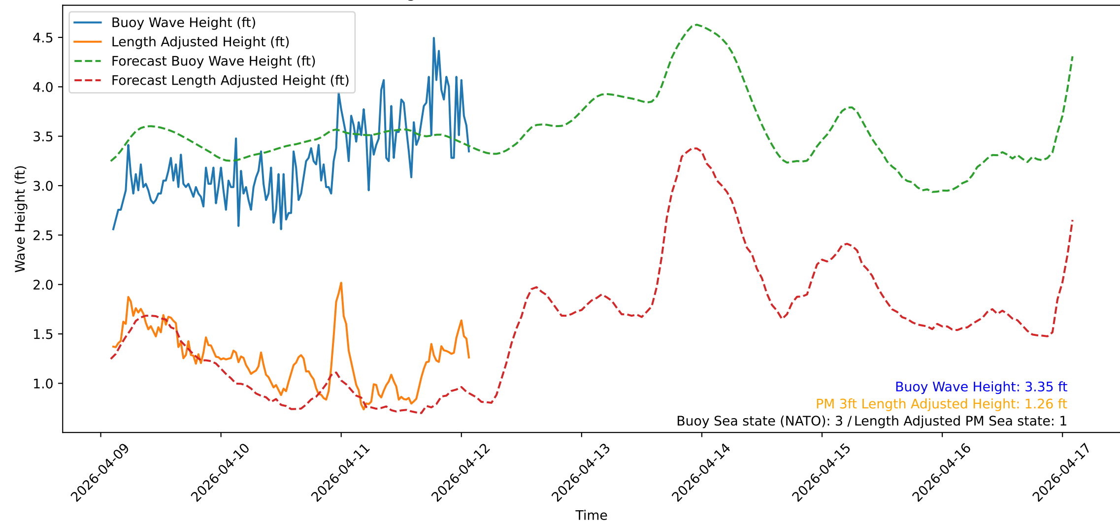
Wave Heights over Time for Green Beach at 2026-04-12 02:21:13
