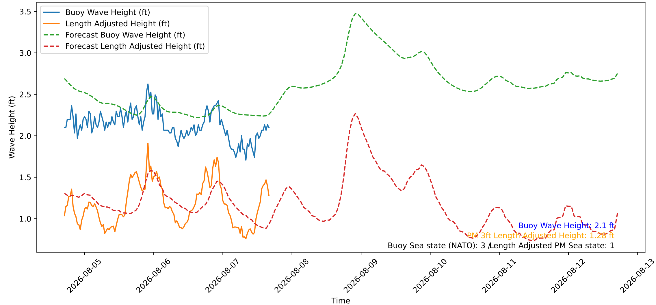
Wave Heights over Time for Green Beach at 2026-08-07 16:51:09
