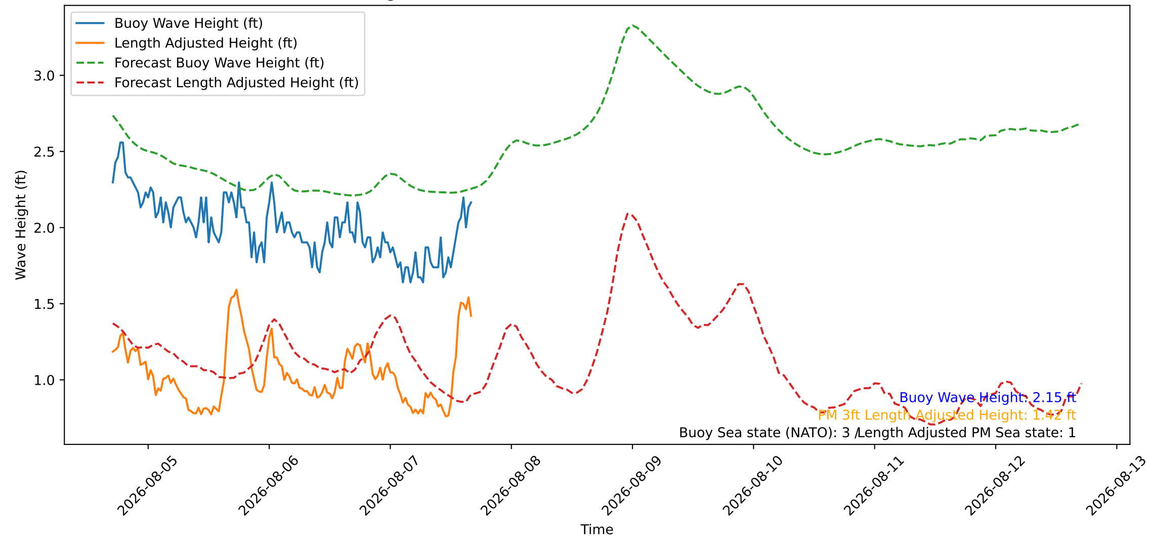
Wave Heights over Time for Oceanside Harbor at 2026-08-07 16:50:26
