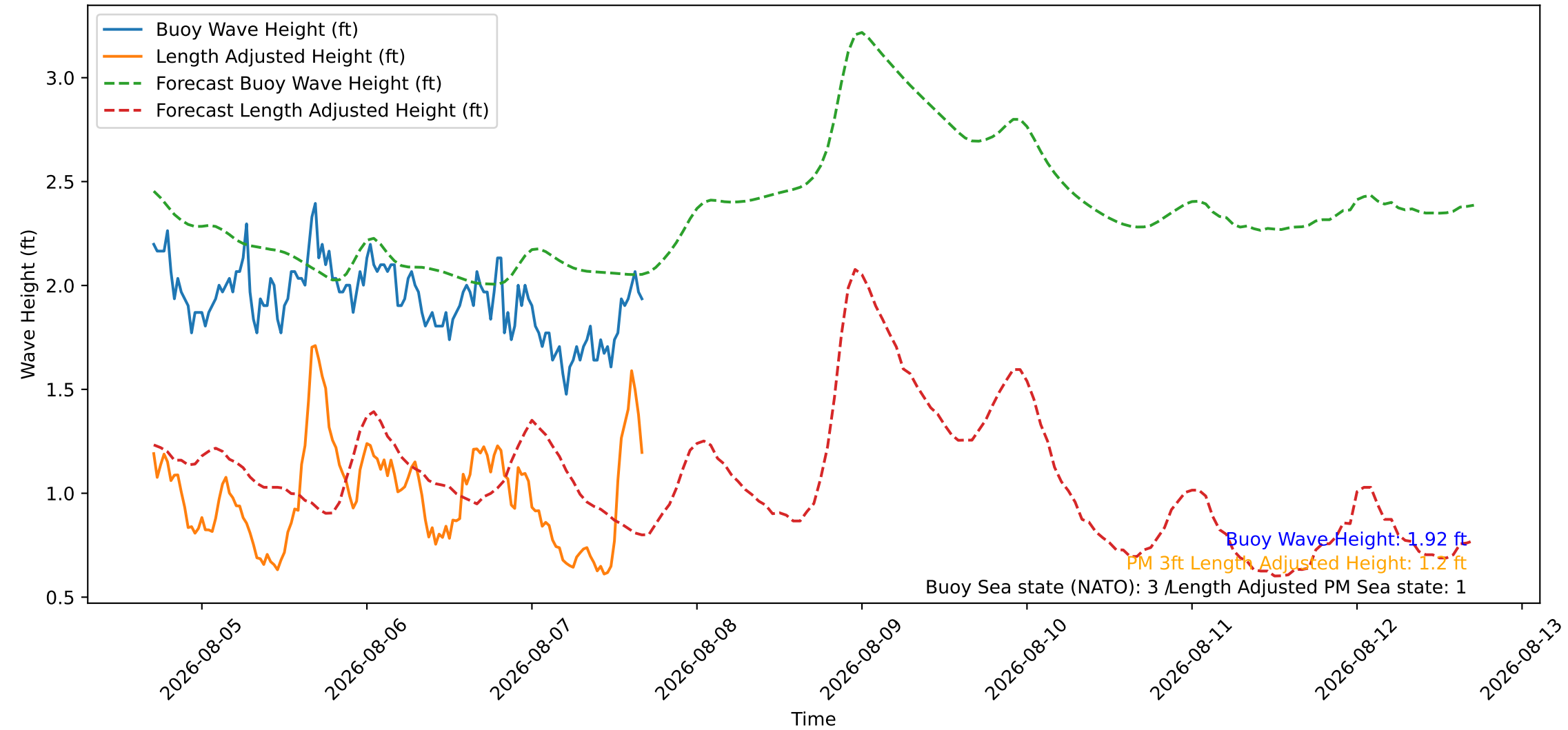
Wave Heights over Time for Red Beach at 2026-08-07 16:50:46
