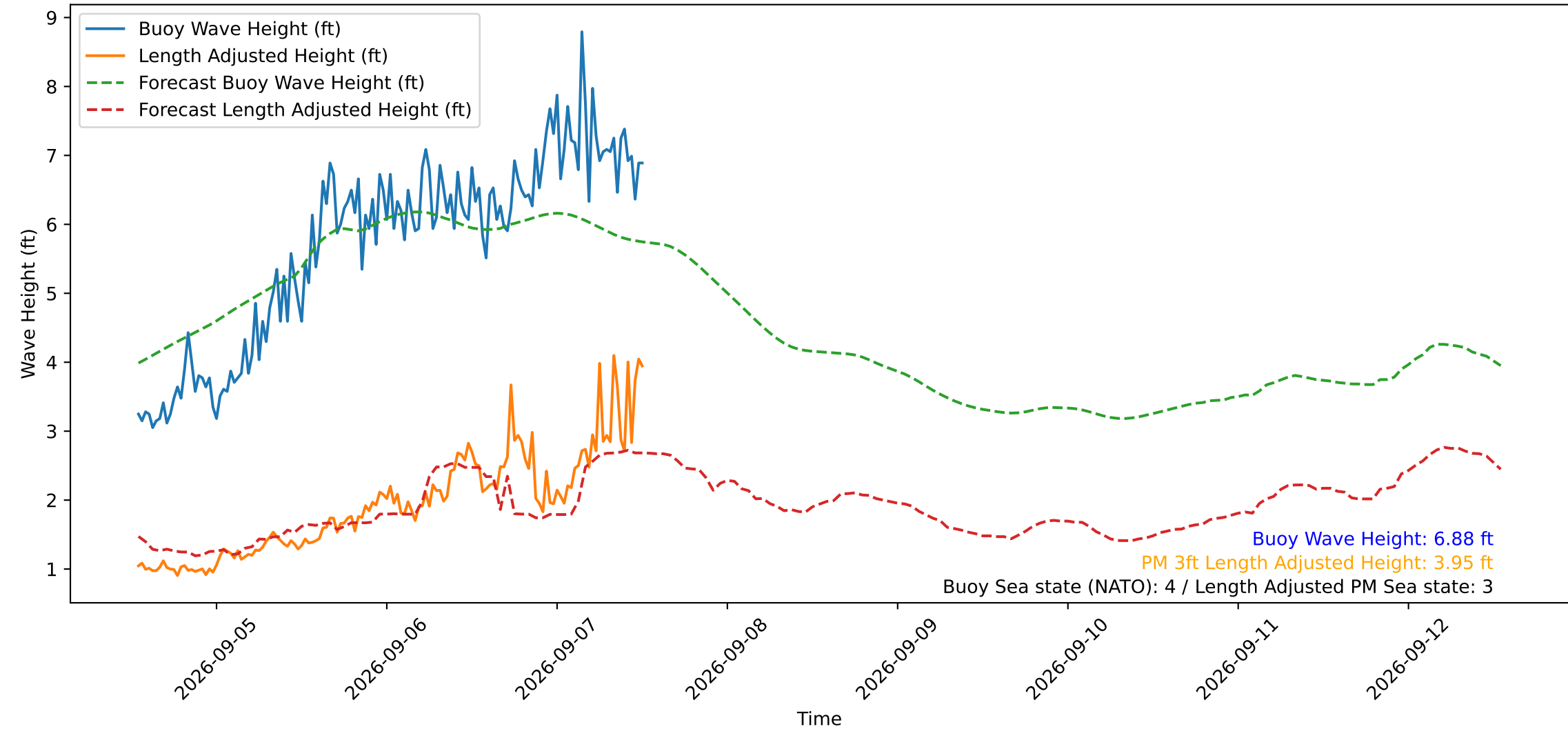
Wave Heights over Time for Green Beach at 2026-09-07 12:41:11
