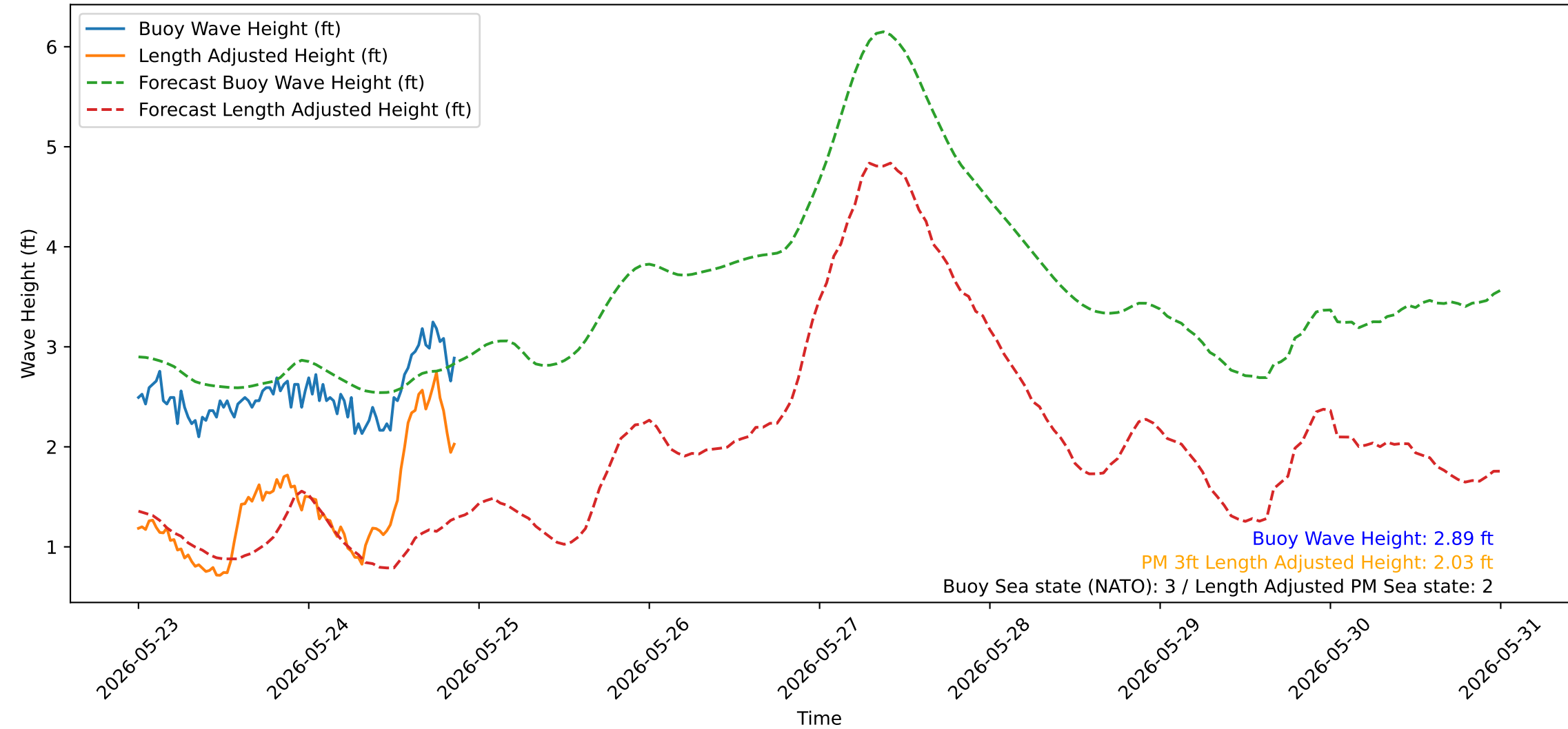
Wave Heights over Time for Oceanside Harbor at 2026-05-25 23:50:29
