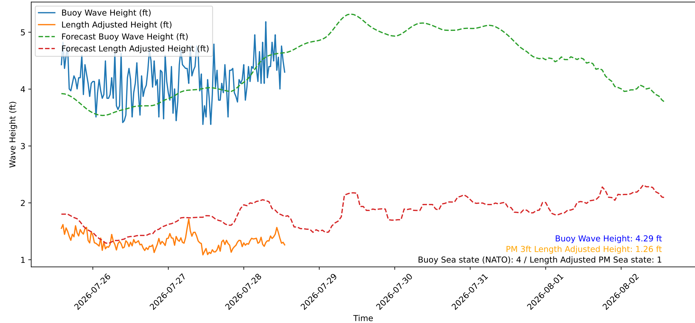
Wave Heights over Time for Green Beach at 2026-07-28 13:51:09
