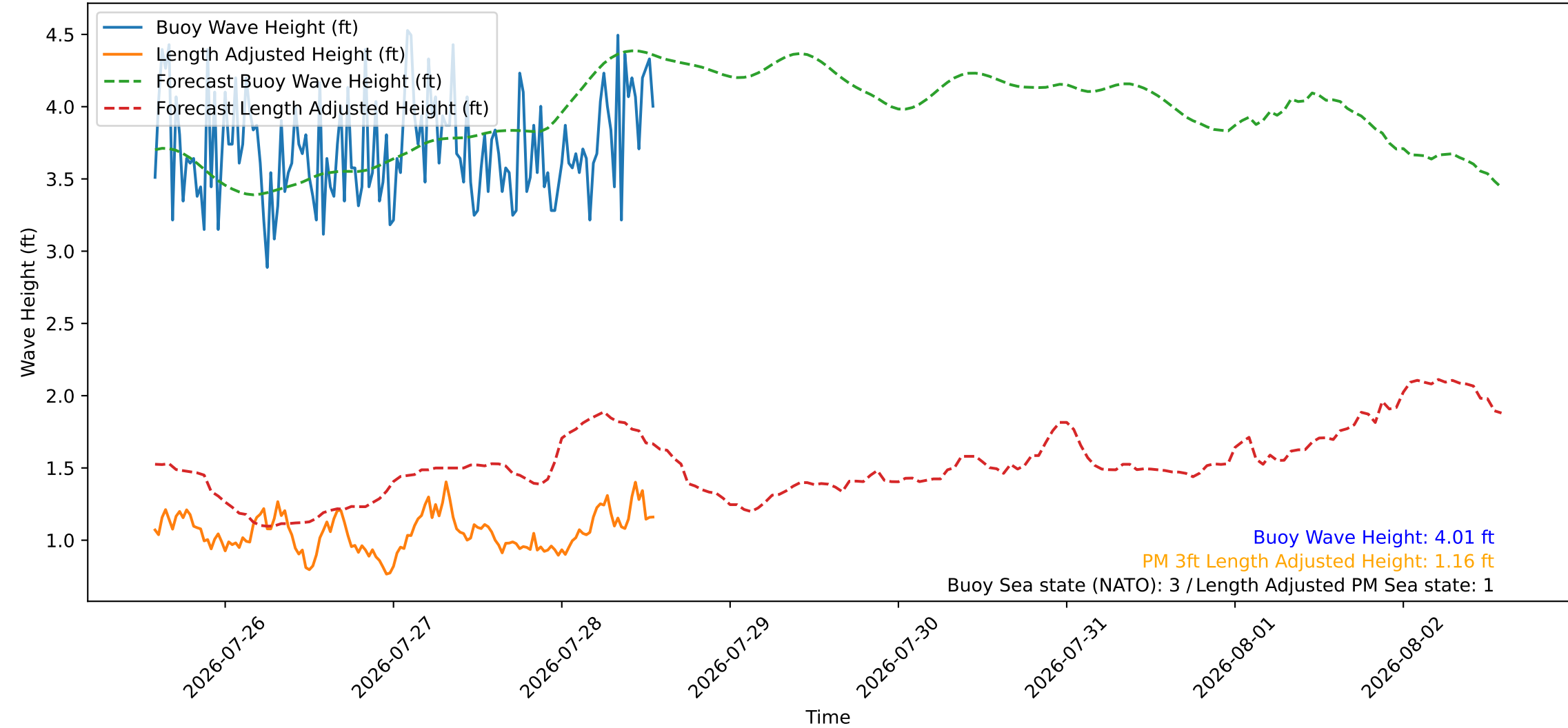
Wave Heights over Time for Red Beach at 2026-07-28 13:50:47
