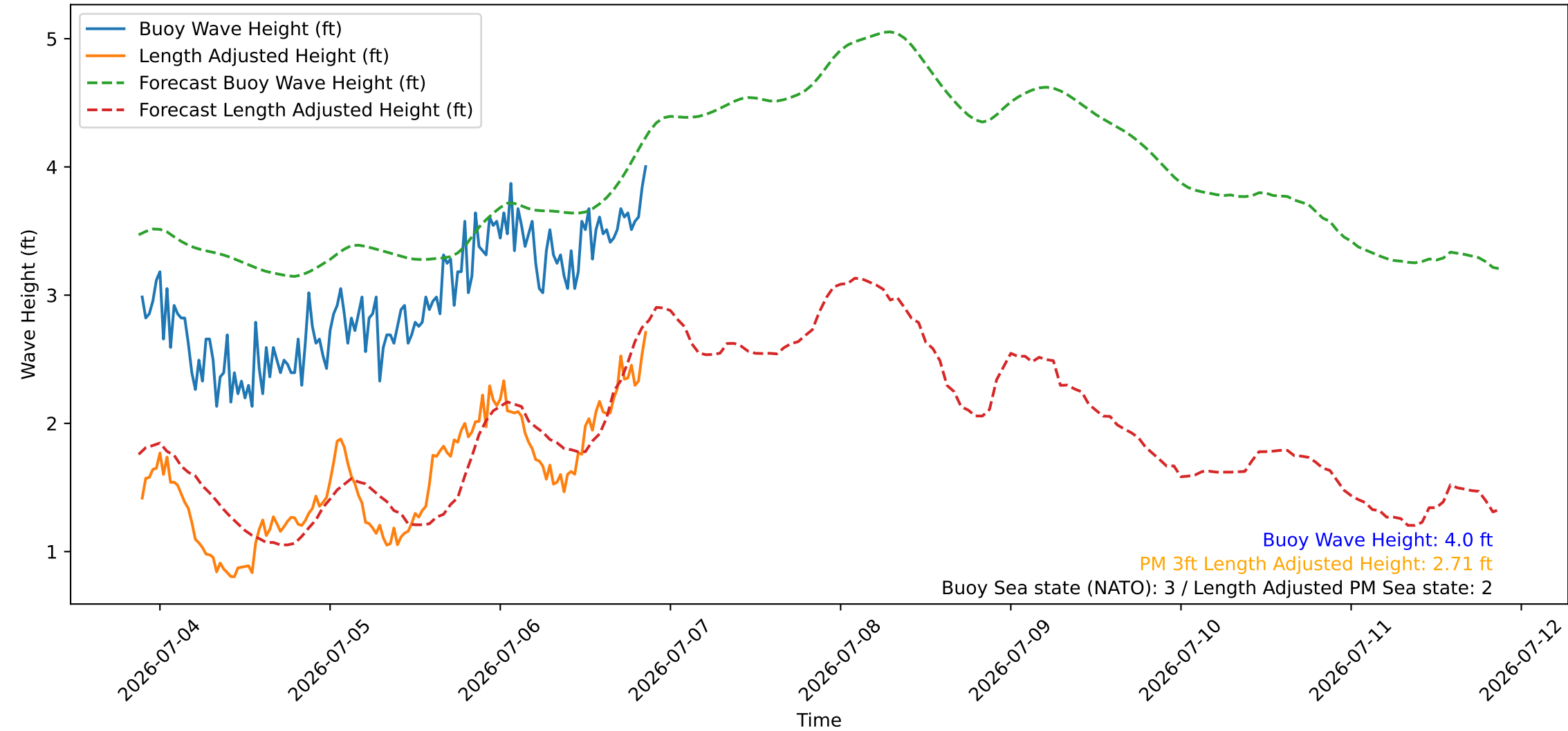
Wave Heights over Time for Oceanside Harbor at 2026-07-06 21:20:26
