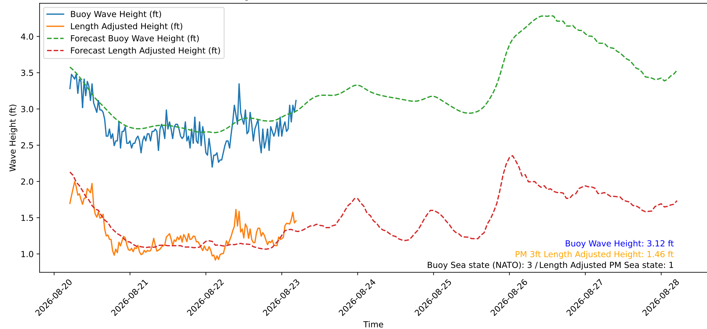
Wave Heights over Time for Oceanside Harbor at 2026-08-23 05:10:29
