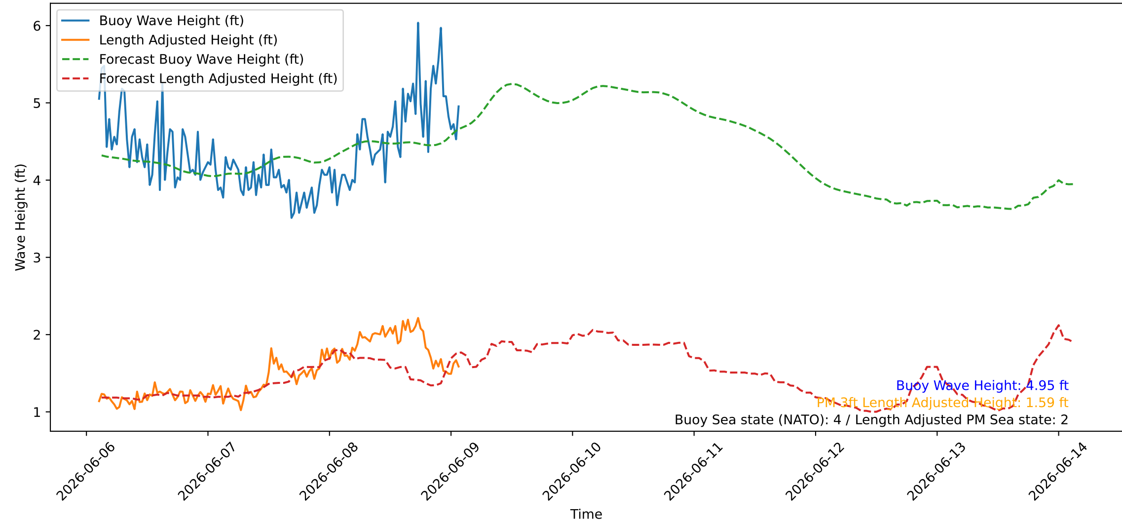
Wave Heights over Time for Oceanside Harbor at 2026-06-09 02:30:26
