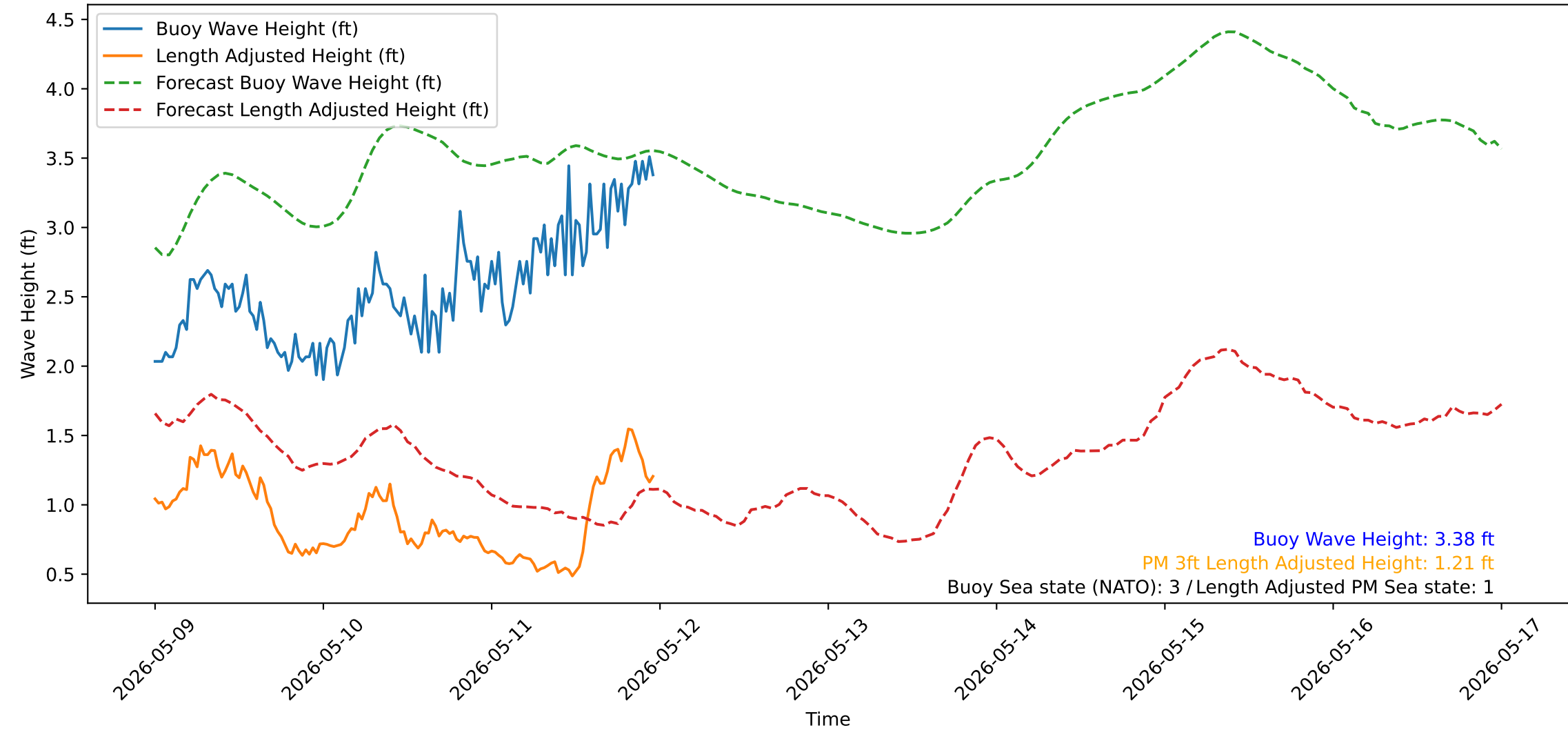
Wave Heights over Time for Green Beach at 2026-05-11 23:51:14
