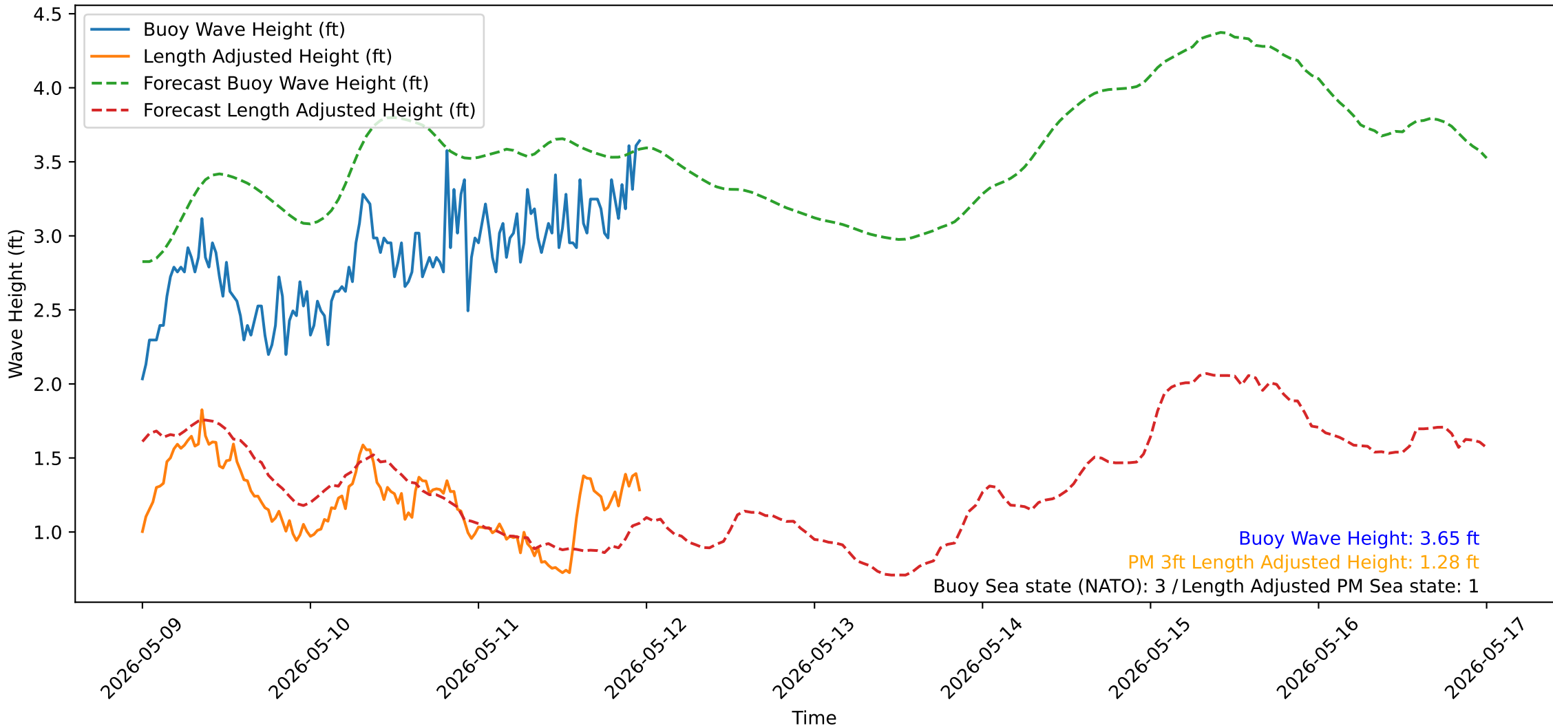
Wave Heights over Time for Oceanside Harbor at 2026-05-11 23:50:31
