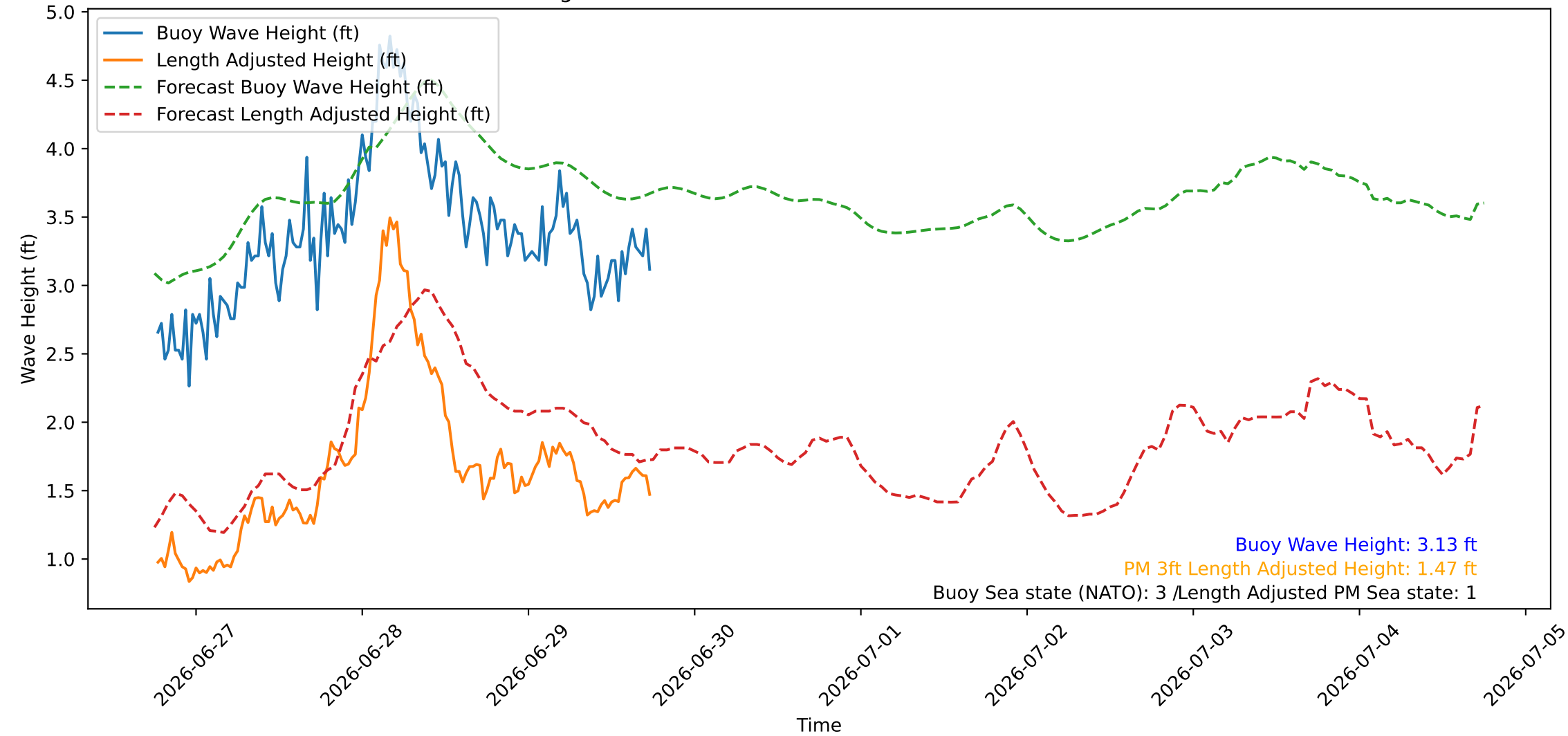
Wave Heights over Time for Green Beach at 2026-06-29 18:21:08
