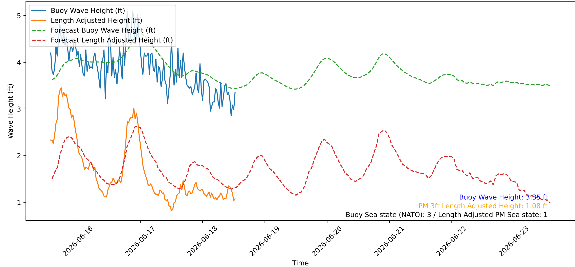
Wave Heights over Time for Green Beach at 2026-06-18 13:41:09
