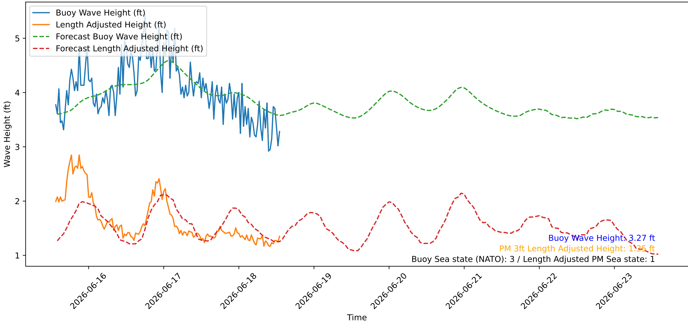
Wave Heights over Time for Oceanside Harbor at 2026-06-18 13:40:26
