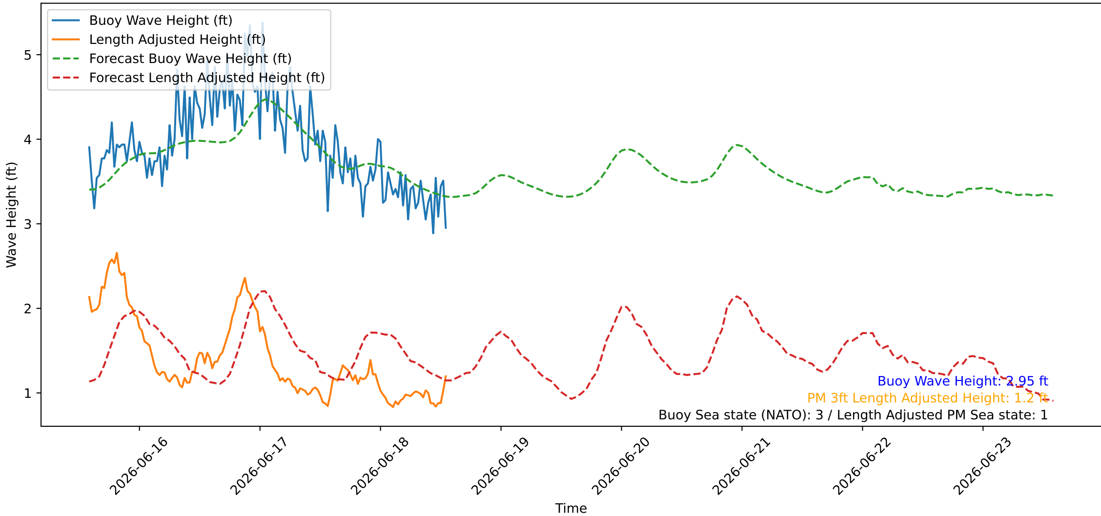
Wave Heights over Time for Red Beach at 2026-06-18 13:40:46
