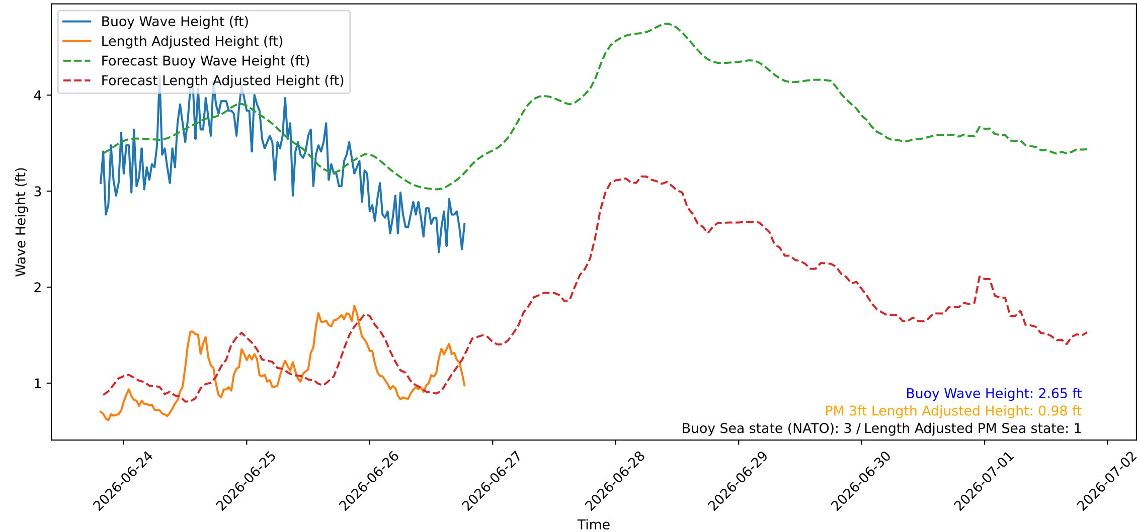
Wave Heights over Time for Green Beach at 2026-06-26 19:31:08
