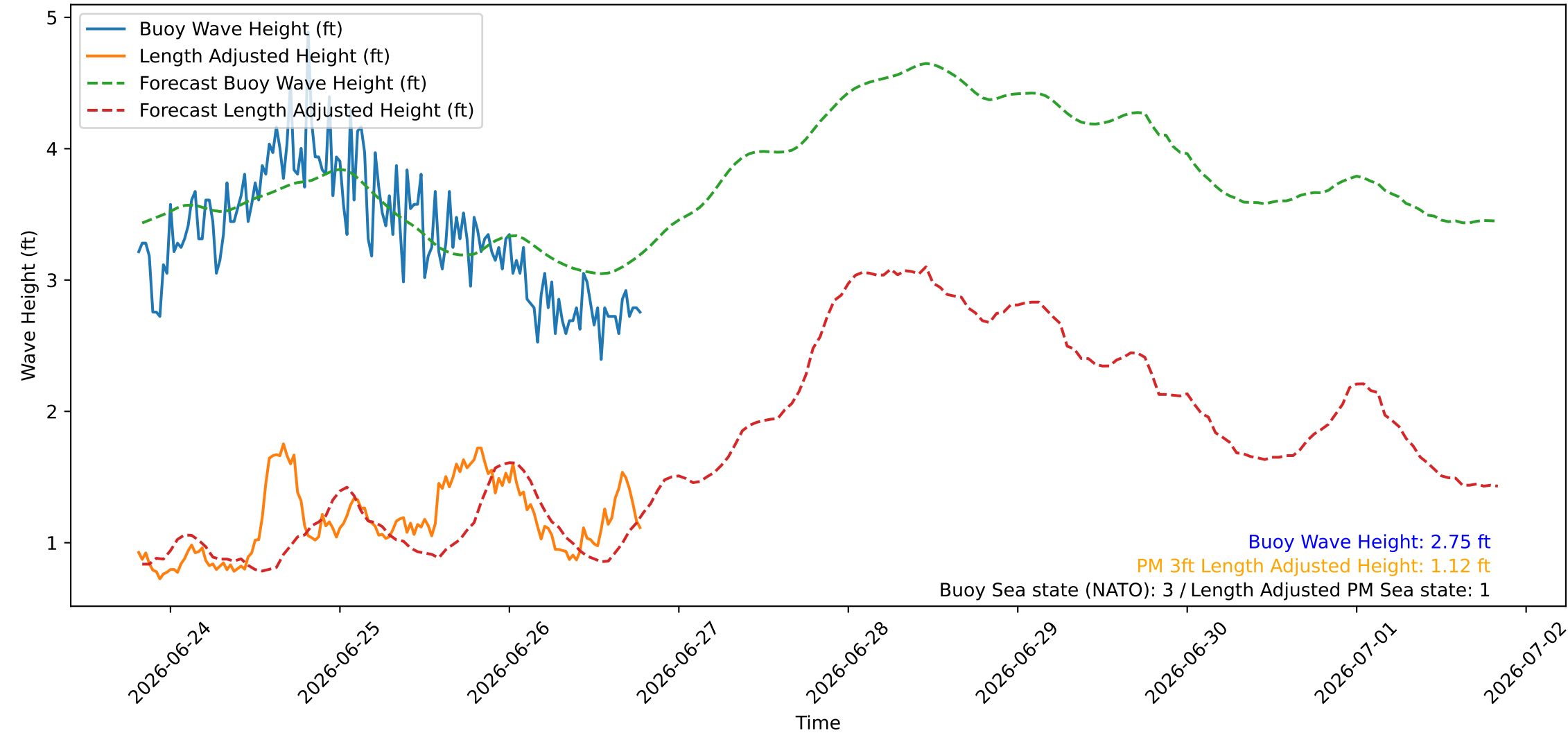
Wave Heights over Time for Oceanside Harbor at 2026-06-26 19:30:26
