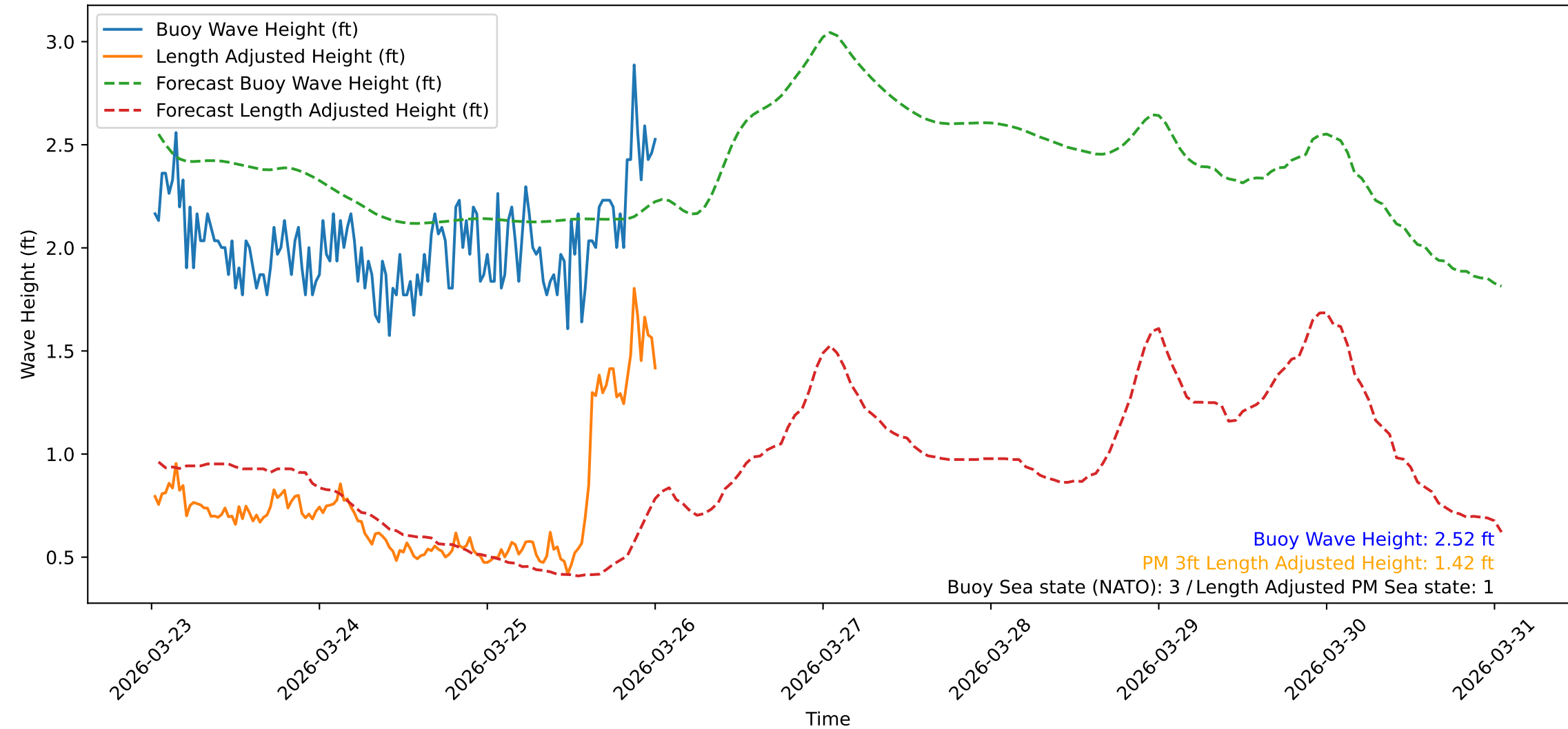
Wave Heights over Time for Oceanside Harbor at 2026-03-26 00:40:32
