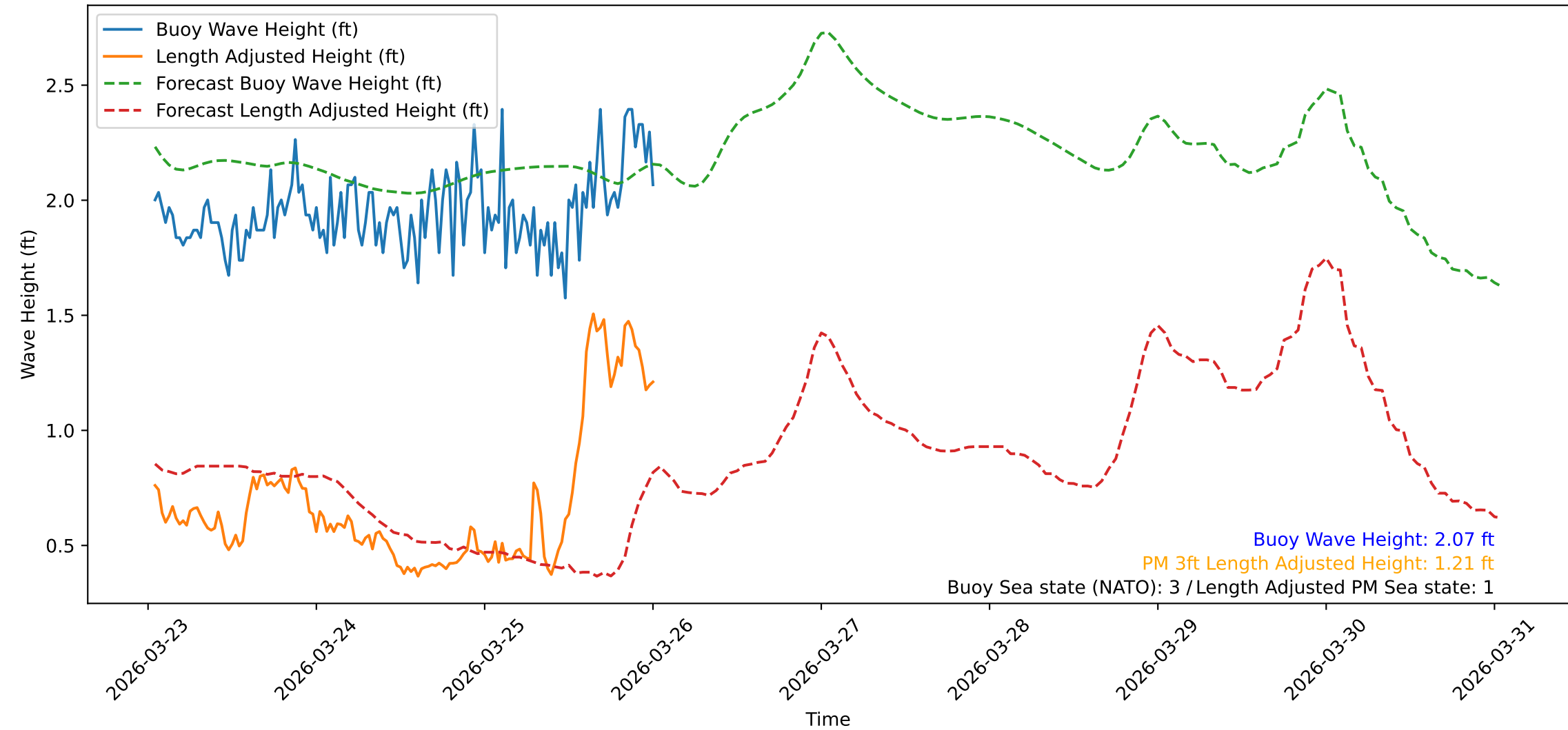
Wave Heights over Time for Red Beach at 2026-03-26 00:40:48
