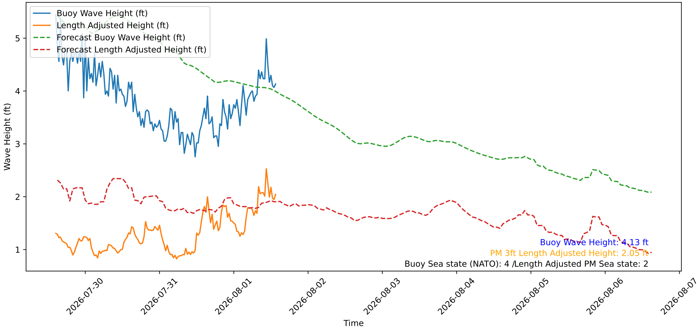
Wave Heights over Time for Green Beach at 2026-08-01 14:31:10
