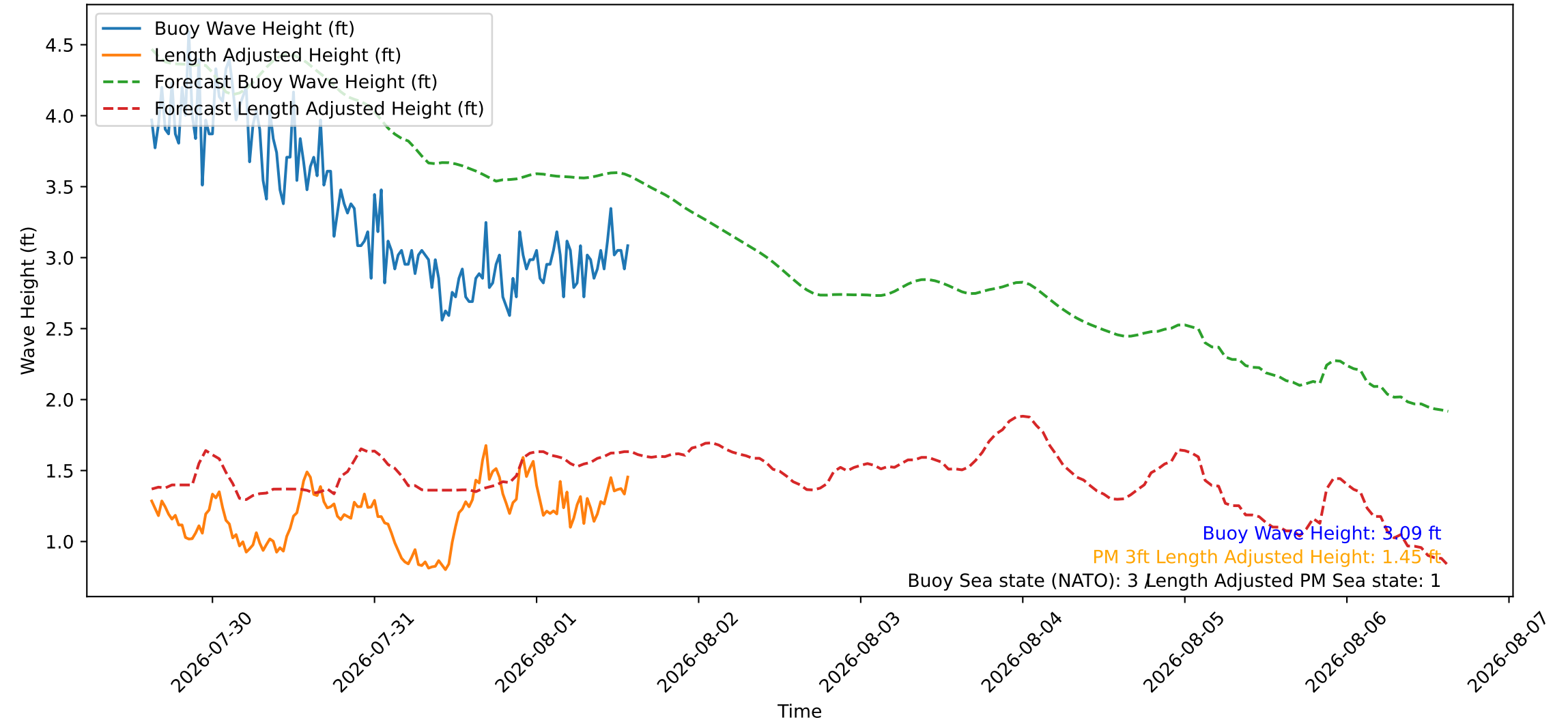
Wave Heights over Time for Red Beach at 2026-08-01 14:30:47
