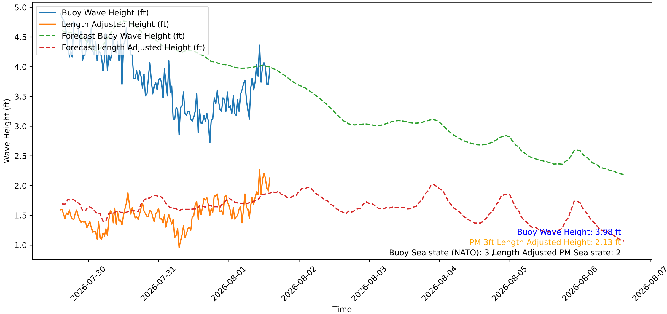
Wave Heights over Time for Oceanside Harbor at 2026-08-01 14:30:27
