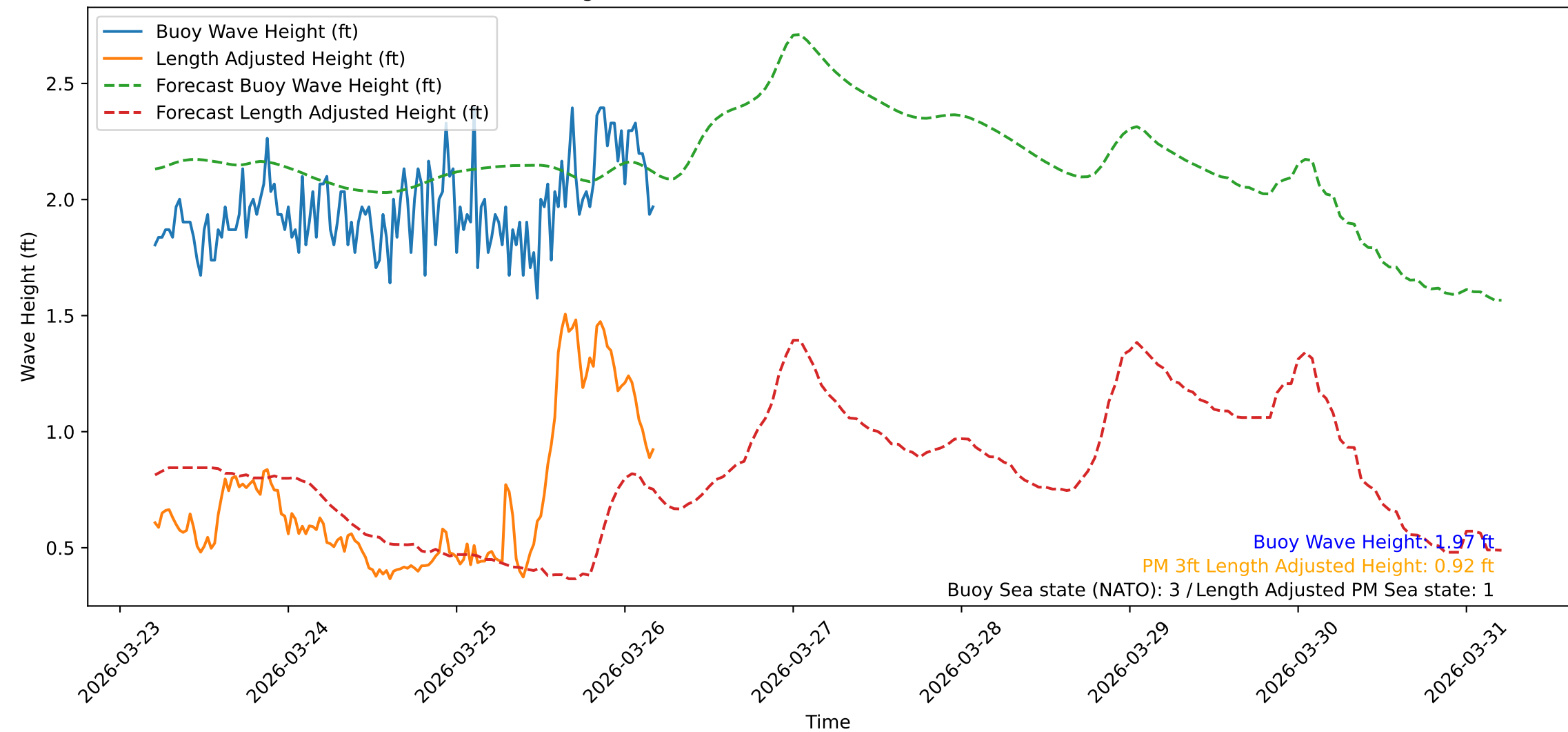
Wave Heights over Time for Red Beach at 2026-03-26 04:40:48
