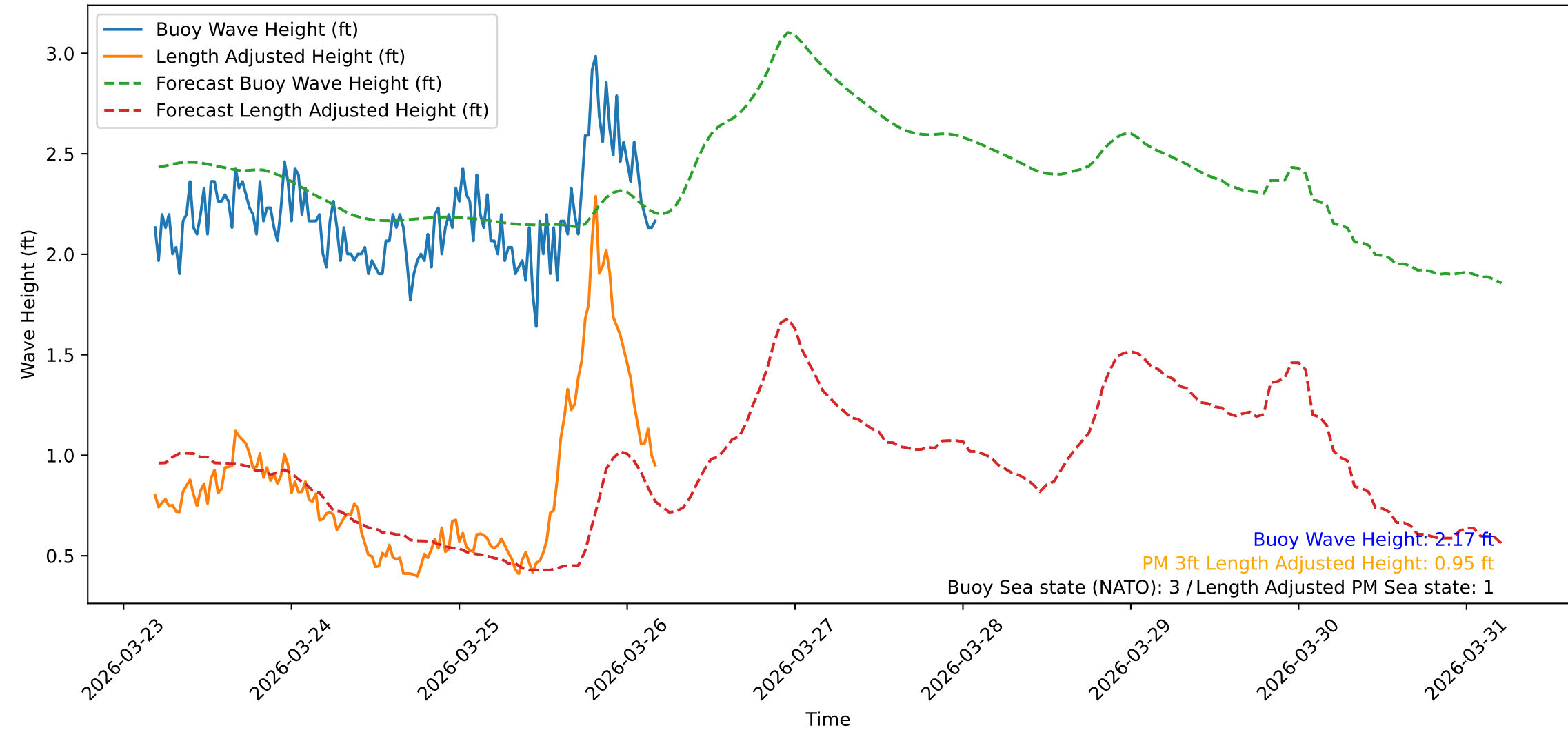
Wave Heights over Time for Green Beach at 2026-03-26 04:41:11
