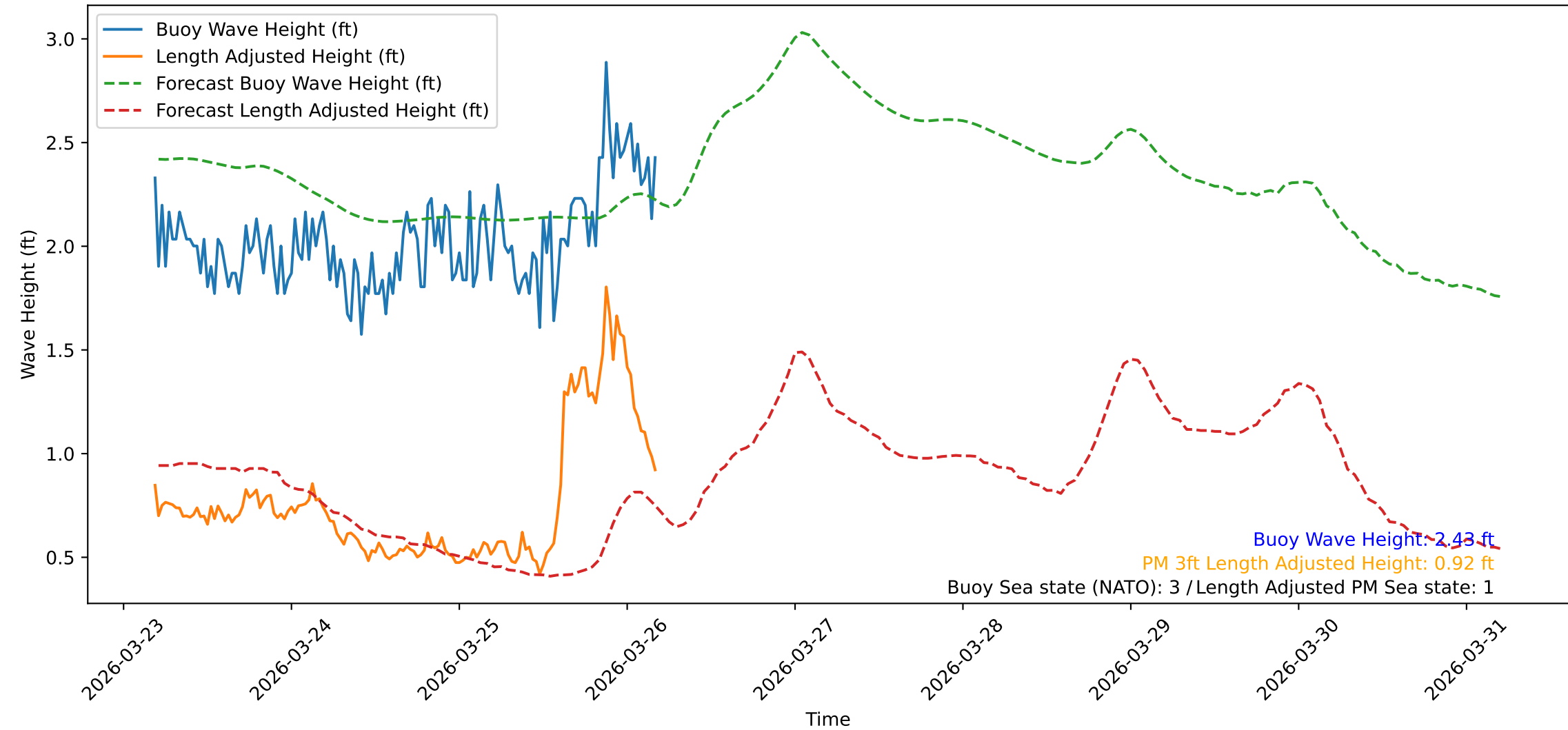
Wave Heights over Time for Oceanside Harbor at 2026-03-26 04:40:31
