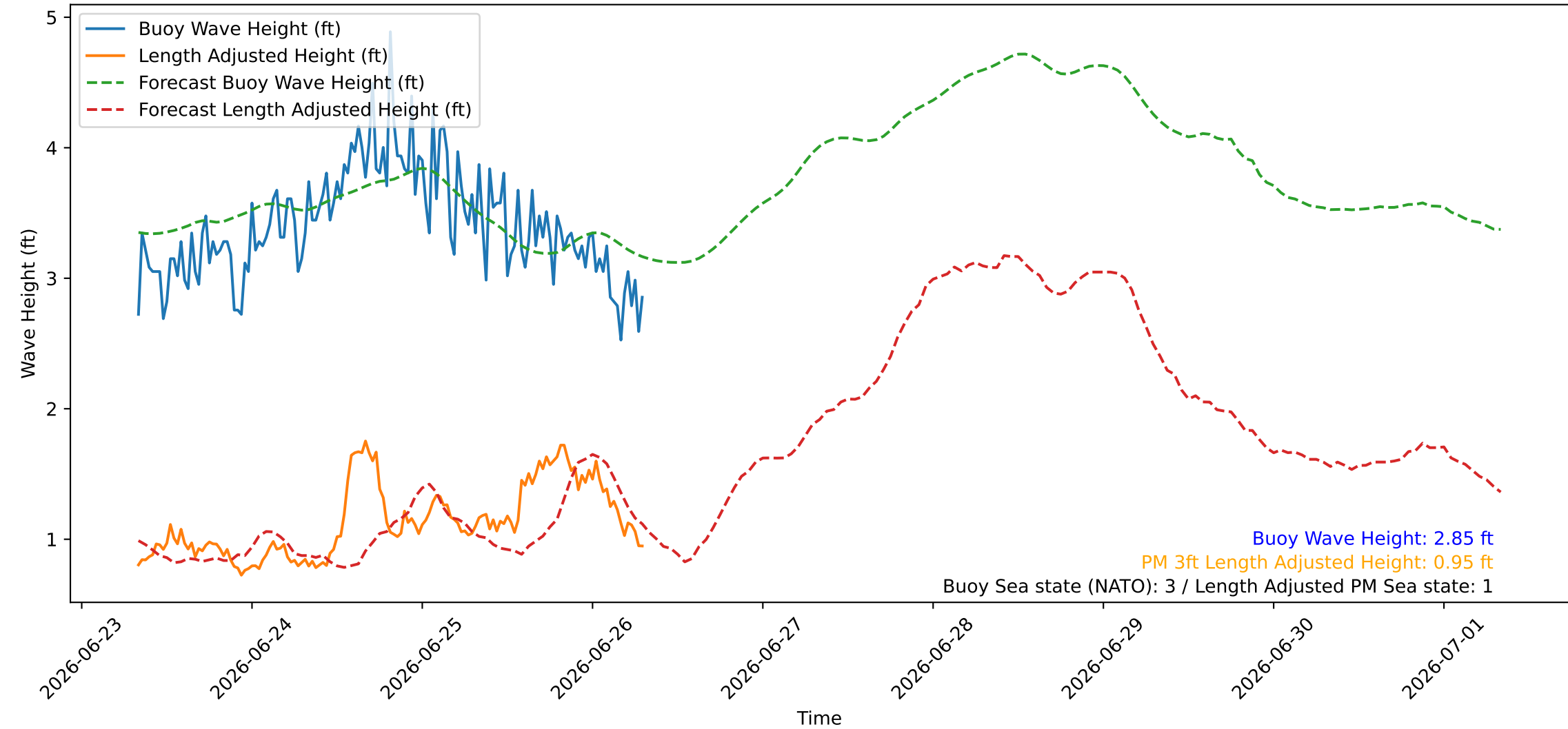
Wave Heights over Time for Oceanside Harbor at 2026-06-26 08:00:26
