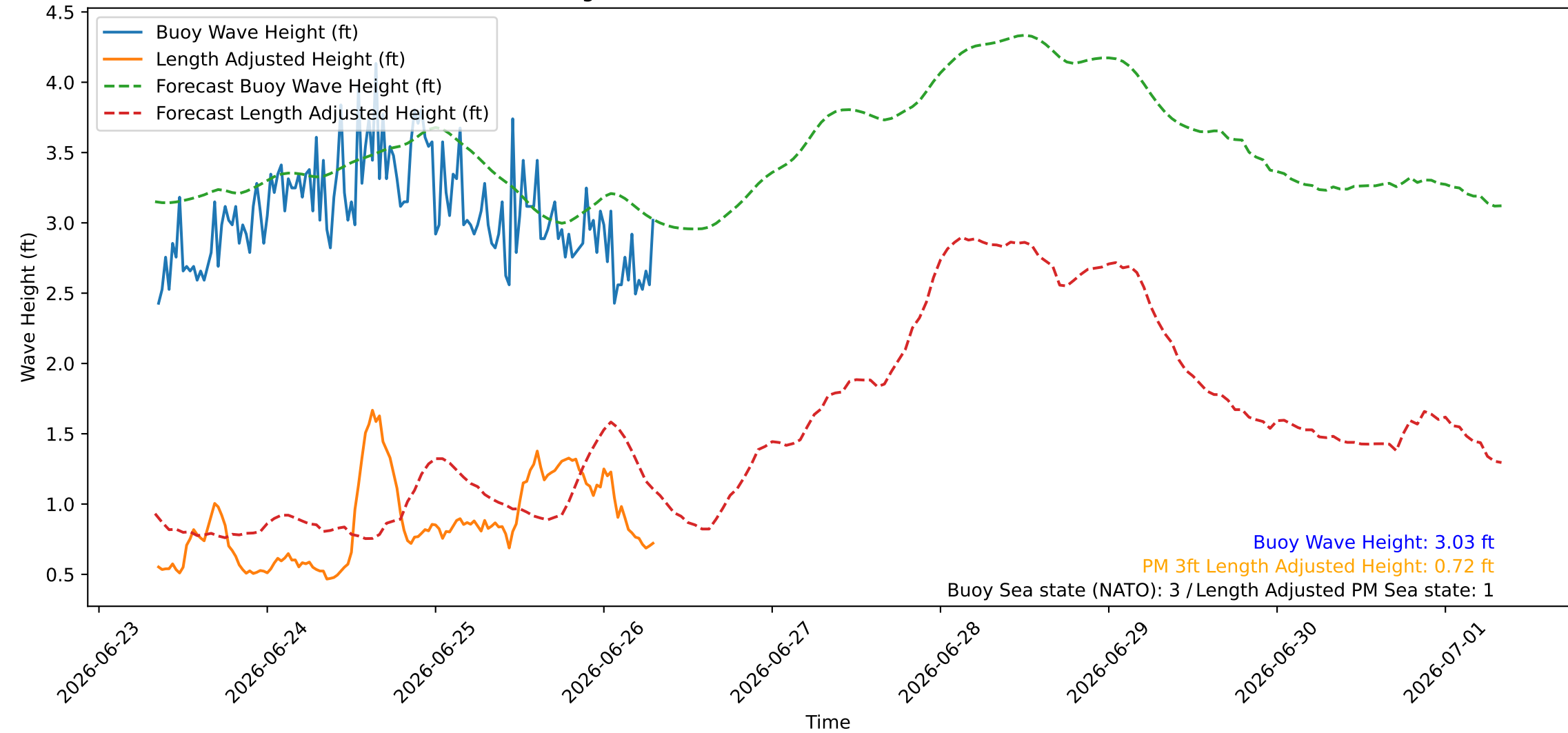
Wave Heights over Time for Red Beach at 2026-06-26 08:00:45
