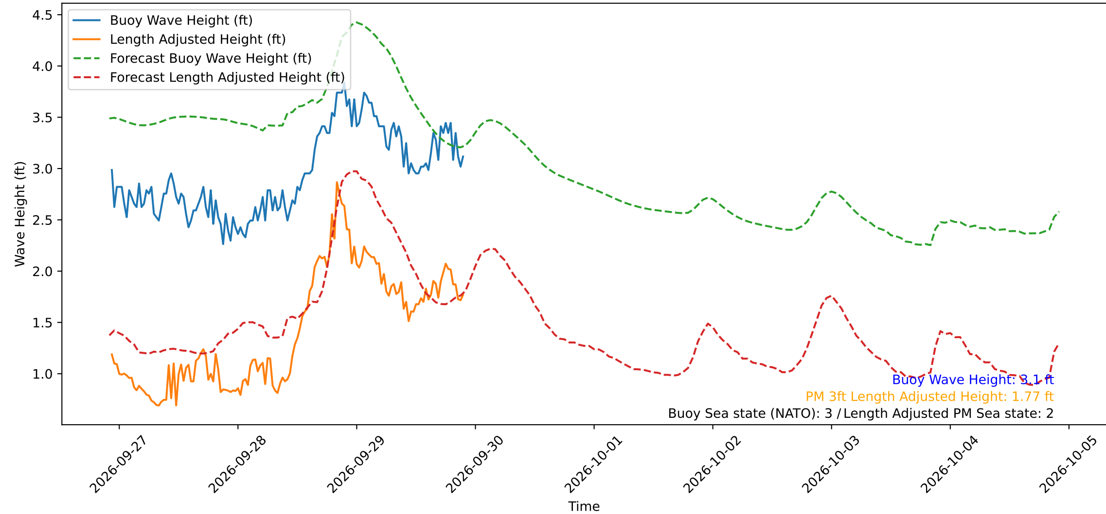
Wave Heights over Time for Red Beach at 2026-09-29 22:20:50
